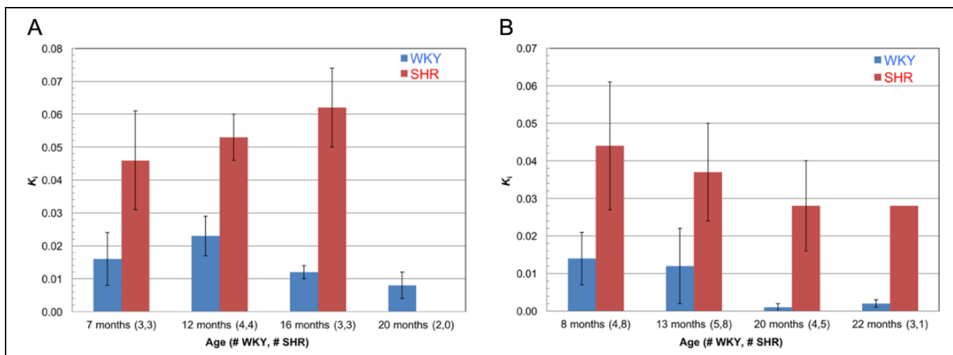
Figure 5. The ^{18}\text{F} -FDG influx rate constant K_i^{\text{FDG}} in myocardium as a function of age for the (A) 2009 to 2010 fed study and (B) 2011 to 2012 fasted study. The Patlak method 4,17 was used to calculate influx rate constant. FDG indicates fluorodeoxyglucose.
