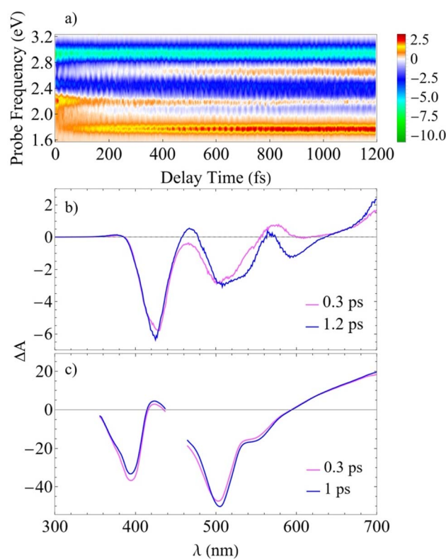
Fig. 7 The total TA-PP signal \overline{S}_{\text{int},M}(t, E_{\text{pr}}) (a) and two cuts of the signal at t = 0.3 and 1.2 ps, (b) evaluated at the magic angle ( 54.7^\circ ) between polarizations of the pump and probe pulses ( s_{\text{pu}} \cdot s_{\text{pr}} = 1/\sqrt{3} ), and (c) measured experimentally. 32
