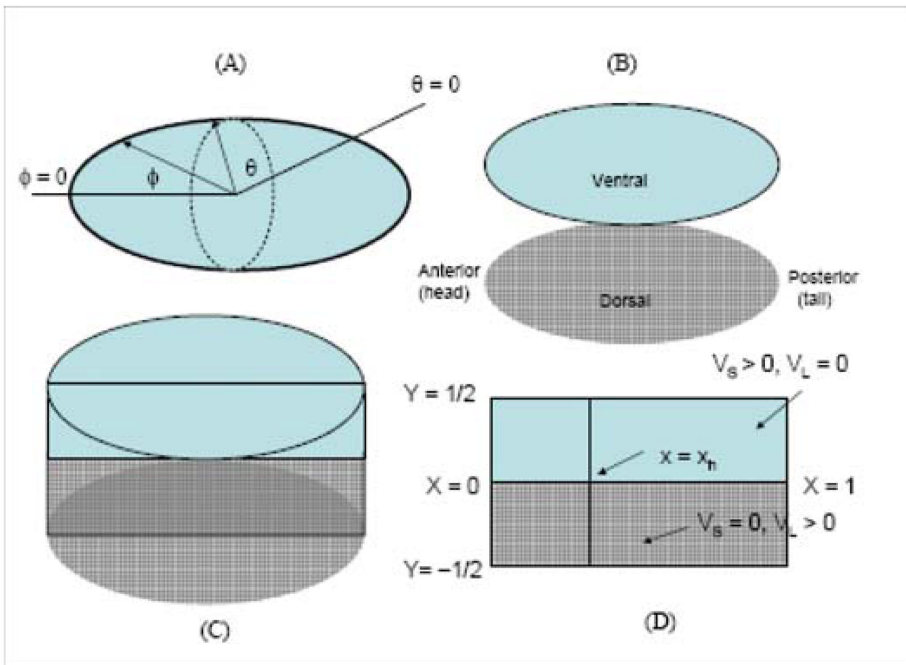
Figure 2. (A) Prolate spheroidal surface domain; (B) dorsal and ventral portion of prolate spheroidal surface; (C) half of the mirror-symmetric domain; (D) idealized half domain as a rectangle in the X,Y - plane.
