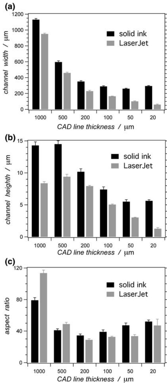
FIGURE 1. Comparison between relief features printed with a solid-ink printer (Xerox 8550D Phaser) and a LaserJet printer (HP 1320), reproducing CAD (FreeHand, v. 10) horizontal lines with different thicknesses. Dependence of: (a) feature width; (b) feature height; and (c) the width-to-height aspect ratio of the features, on the lines on the CAD images. The data are collected from profilometry measurements (six measurements per a data point; error bars represent 0.9 confidence limits, based on Student's t -distribution).
