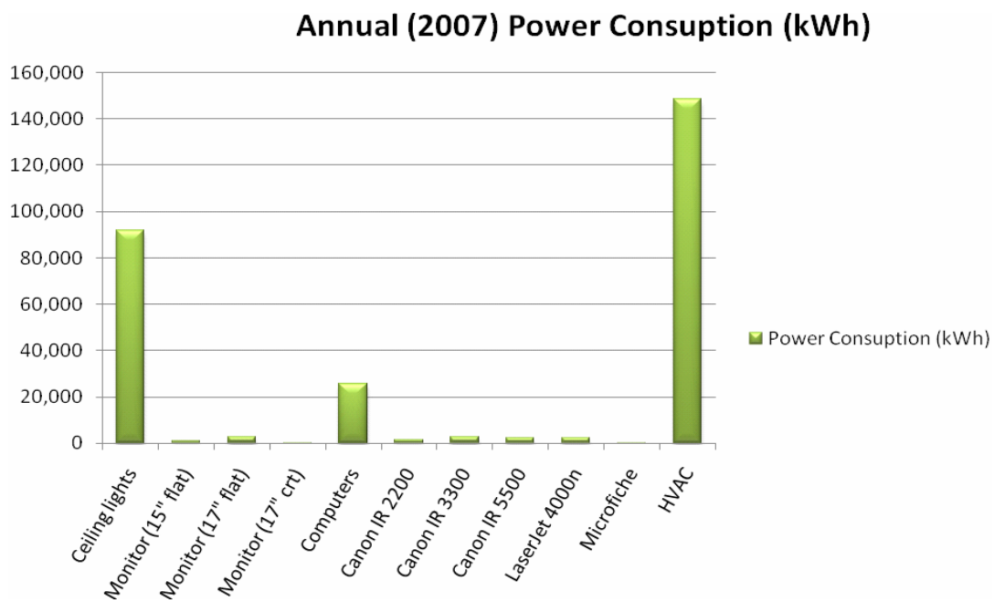
Fig.4 Bar graph of all power consumption for all the major electric items
