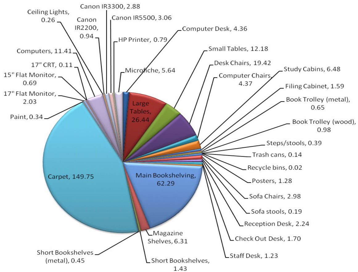
Fig.5 Pie chart of GWP for embodied energy of the infrastructure
