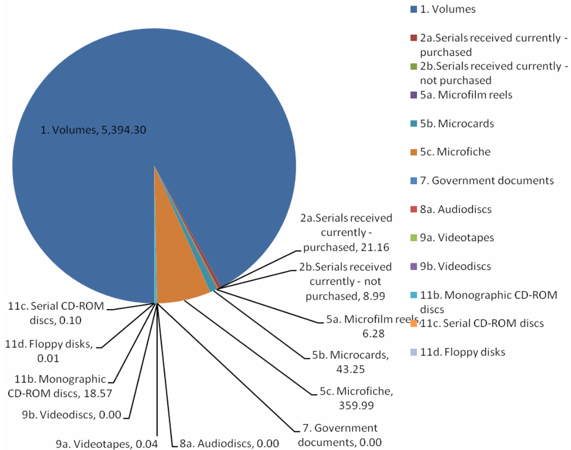
Fig.6 Pie chart of the GWP for the embodied energy of books and documents
