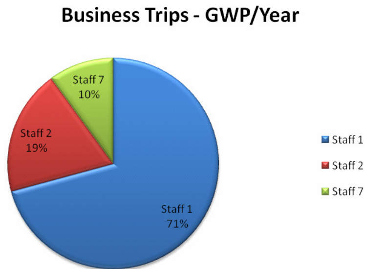
Fig.3 Pie chart of GWP/Year for staff business trips
