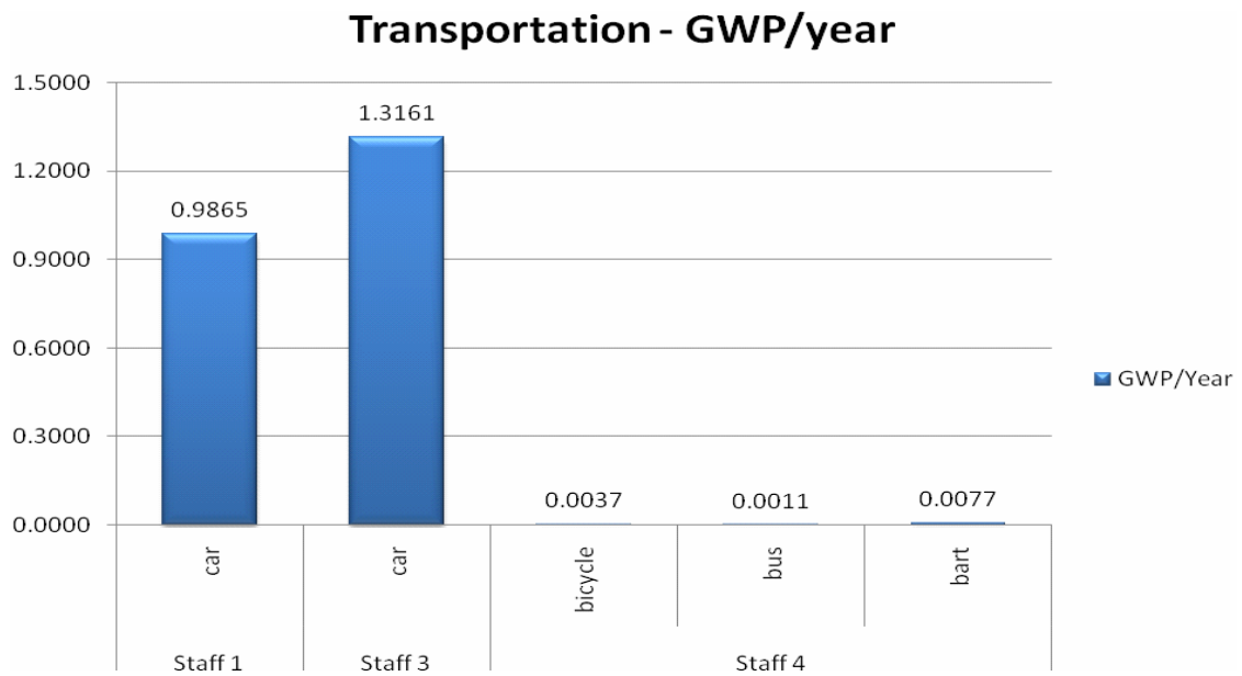
Fig.2 Bar graph of non-zero GWP/Year for Transportation
