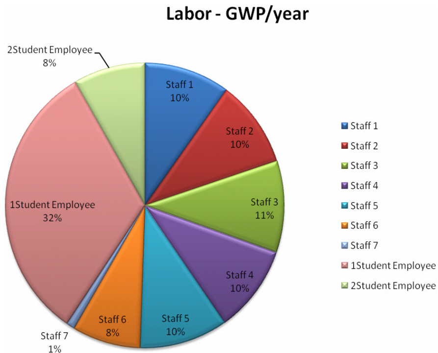
Fig.1 Pie chart of GWP/year distribution for Labor
