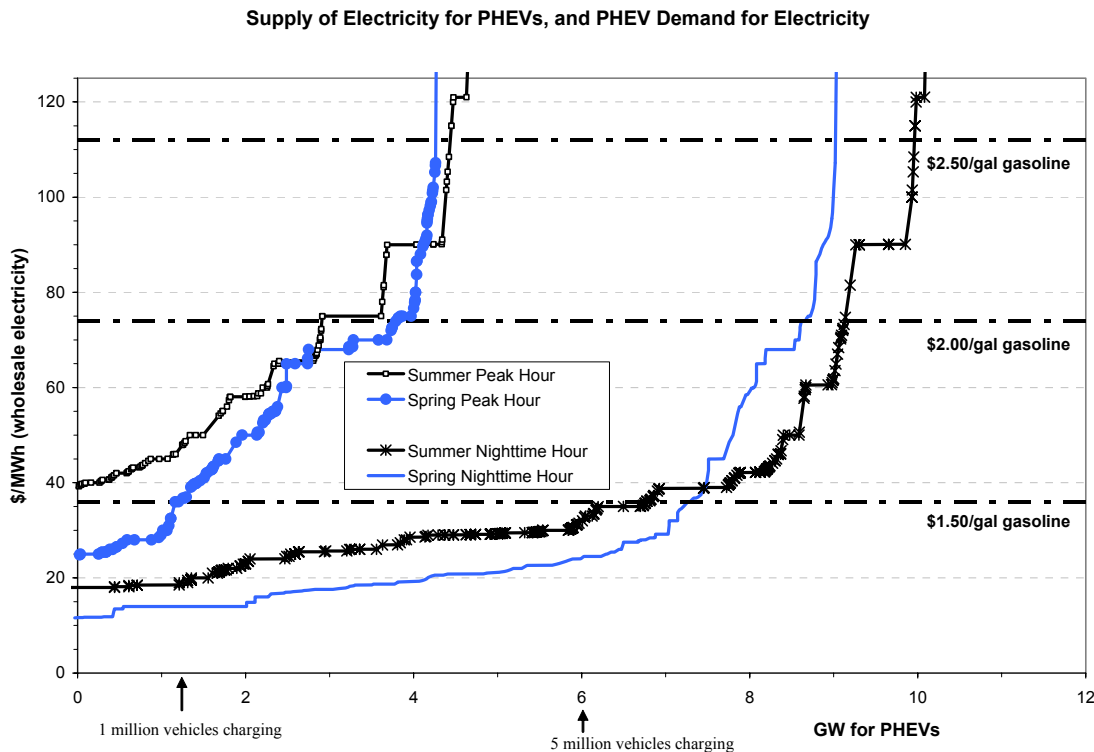
Figure 4-7: The quantity of electricity beyond observed demand available at each price, as determined by the supply bids given to the California Power Exchange in 1999. Also, the number of PHEVs that would need to charge during the hour to use that much electricity with a charge rate of 1 kWh/hr (or a charger size of 1.2 kW).
