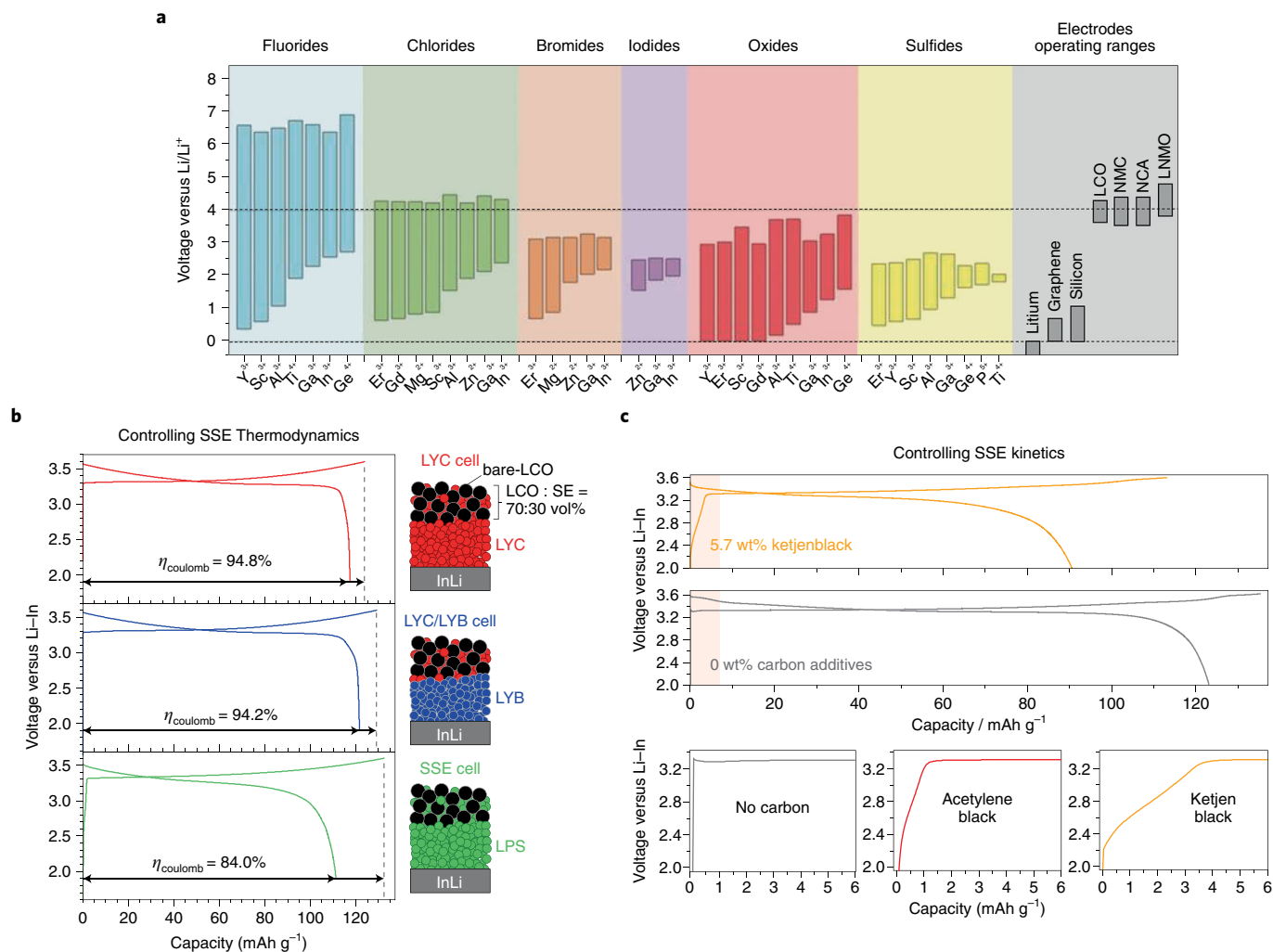
Fig. 2 | Electrochemical stability of various solid electrolytes and their effects on cell performance. a , Illustration of solid electrolytes stability windows versus common electrodes typical operating potential. LCO, lithium cobalt oxide; NMC, nickel manganese cobalt; NCA, nickel cobalt aluminium; LNMO, lithium nickel manganese oxide. b , Methods to improve thermodynamic stabilities of solid electrolytes, by using a solid electrolyte of higher oxidation stability. LYC, Li 3 YCl 6 solid electrolyte; LYB, Li 3 YBr 6 solid electrolyte. c , Methods to control decomposition kinetics of solid electrolytes, by using carbon with lower specific area. Adapted with permission from refs. 36,85, Wiley-VCH Verlag GmbH & Co. KGaA ( a and b , respectively); and ref. 42, American Chemical Society ( c ).
