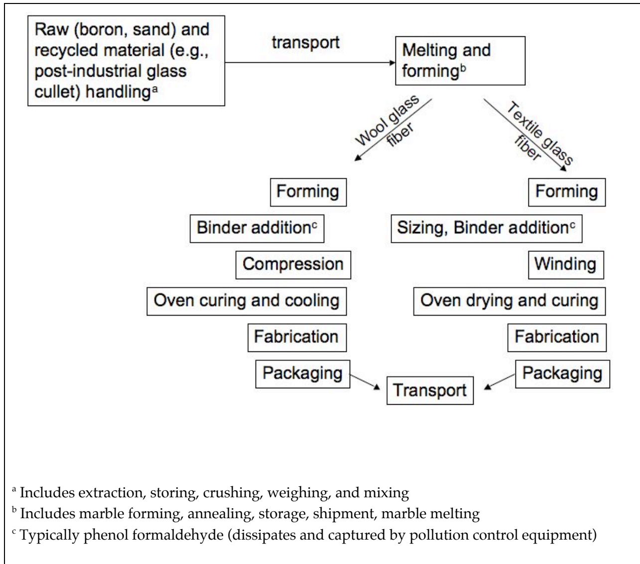
Figure 5. Materials and processes involved in the manufacture of fiberglass insulation (adapted from: EPA, 1985)
