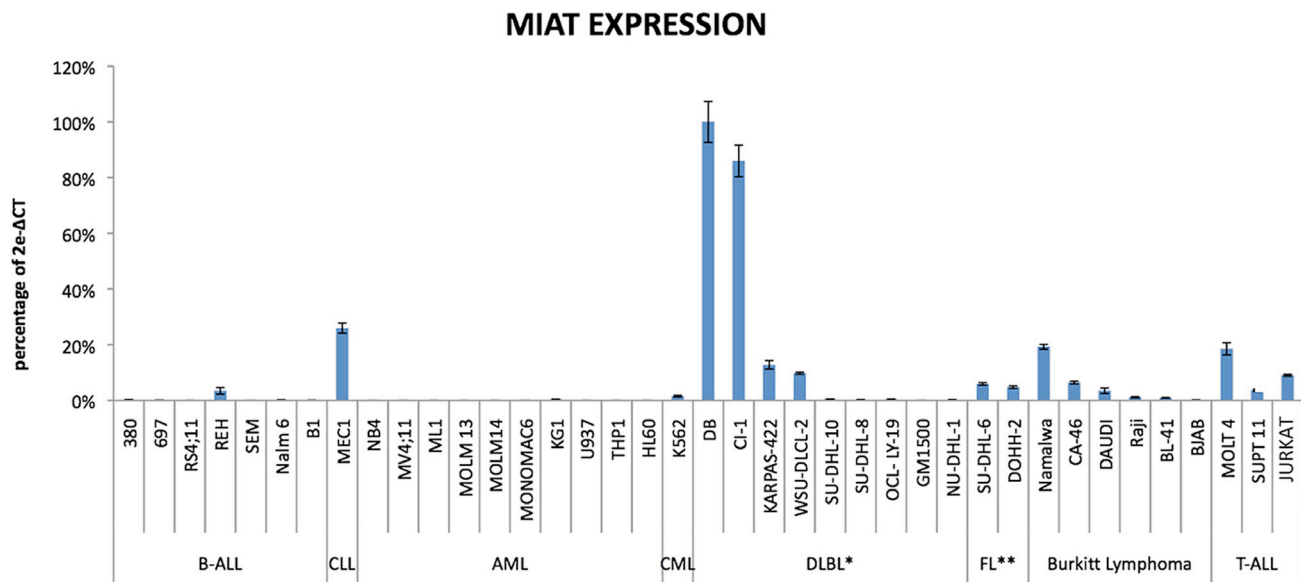
Figure 1: MIAT expression in Leukemia/Lymphoma cell lines. MIAT expression was shown as percentage against expression level of TBP according to the following formula: 2e^{-\text{critical threshold of MIAT}} - \text{critical threshold of TBP} \times 100 . Realtime RT-PCR was carried out in triplicate and standard error bar was on top. *: Diffuse Large B Cell Lymphoma. **: Follicular Lymphoma.
