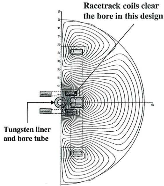
Figure 1: The cross section, field lines and the design concept of the proposed high field Nb 3 Sn design for muon collider.
