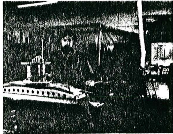
Winding in progress. Machine in background supplies conductor under controlled tension and applies spiral wrap insulation and epoxy coating. Supply spool on the fixture holds conductor for the second layer of the double pancake.
