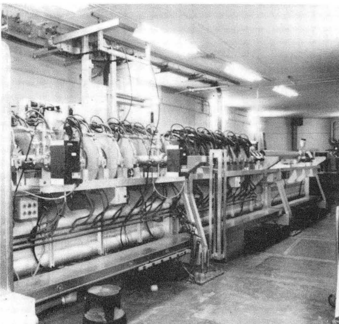
Fig. 2. The ALS linac, with the gun housing on the left. The gun-to-linac and first linac sections are surrounded by solenoid coils and supported on three rigid girders. The 3-GHz waveguide is visible at the top of the picture, and the switching magnet is at the extreme right. [CBB 900-9336]
