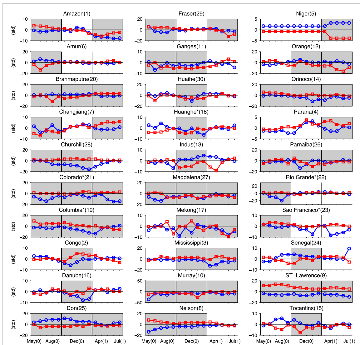
Figure 2. Composite monthly discharge anomalies for the EP El Niño (red) and CP El Niño (blue) for the thirty selected rivers. The discharge anomalies have been normalized by the standard deviation of the discharge calculated for that particular river basin for each particular calendar month. The normalization was performed to account for the fact that the magnitude of discharge variations varies from basin to basin. Rivers are listed in alphabetical order. The number in the parenthesis denotes the ranking of the drainage area size as shown in figure 1. The values shown are the discharge anomalies from zero in each river basin. Gray areas indicate the one or both of the CP and EP averaged discharge anomalies (to zero) in that phase pass the 90% significance level of a two-tailed Student's t test. Note that the y-axis scale is different for each river basin. The “*” symbol after the river name denotes that this river may be influenced by human interventions.
