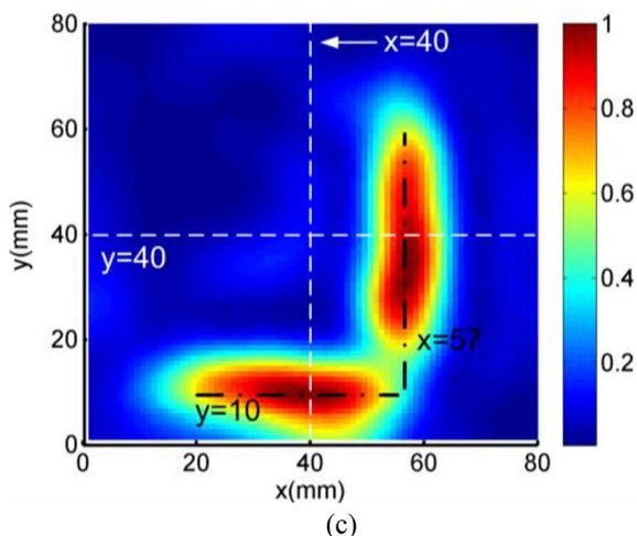
Fig. 13. Normalized magnitude of measured electric-field energy for right angle bent profile. (a) 2-D measured electric field probed by x -polarized monopole. (b) 2-D measured electric field probed by y -polarized monopole. (c) The combined measured near-field pattern through vector superposition. Dotted lines represent the patterned electric fields with the direction along the line. Dashed lines are the sampled lines for focusing effects.
