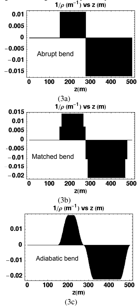
Figure 3. Inverse instantaneous radius of curvature ( m^{-1} ) as a function axial distance (m) for (a) an abrupt bend, (b) a matched bend, and (c) an adiabatic bend, using driver parameters of table 1. Peak strength is shown, with bend occupancy of 0.65.
