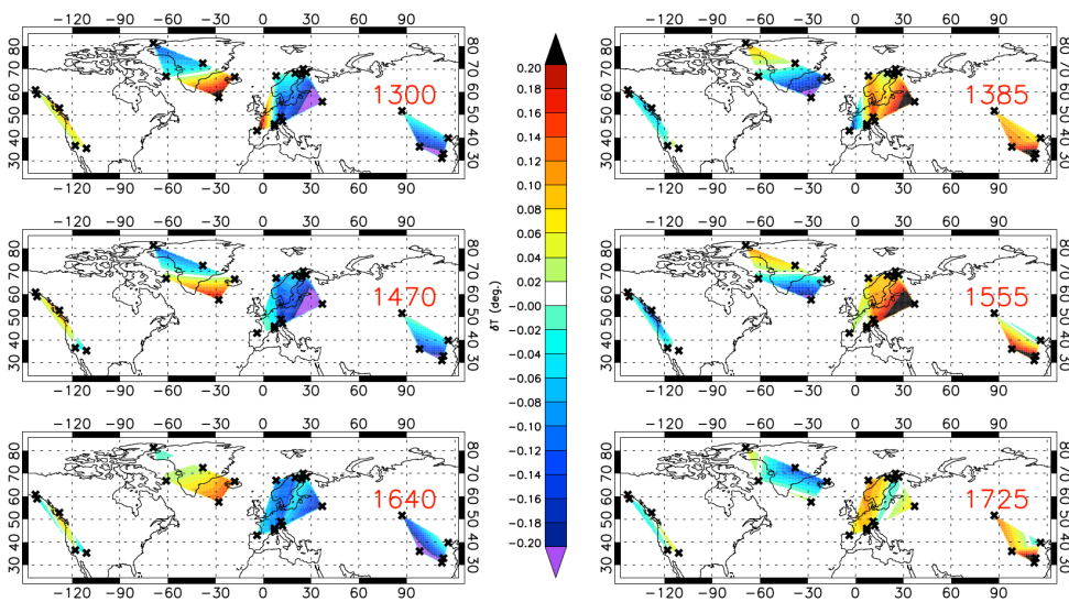
Fig. 9 RC triplet 6-8 of temperature anomalies that captures variability on the time scale of \sim 170 yr. The spatial patterns are shown at half-period intervals, over three full cycles of the oscillation. The contour interval for the anomalies is 0.02^{\circ}\text{C} ; the maximum/minimum contours are at \pm 0.2^{\circ}\text{C} respectively.
