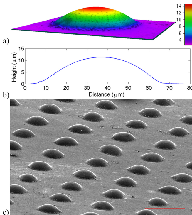
FIG. 3. (Color online) (a) 3D image of lens mold by optical profilometer (μm). (b) Example of microlens mold profile. (c) SEM image of microlens. Scale bar = 100 μm.
