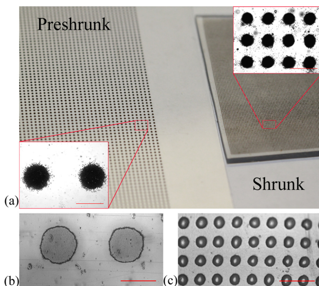
FIG. 2. (Color online) Images of PS mask and PO mold: (a) Macro image of preshrunk and shrunk PS mask. Left inset ink spots on preshrunk PS. Right inset ink spots on shrunk PS. Scale bar = 500 μm. (b) Photoresist spots on preshrunk PO. Scale bar = 200 μm. (c) Photoresist spots on shrunk PO. Scale bar = 200 μm.
