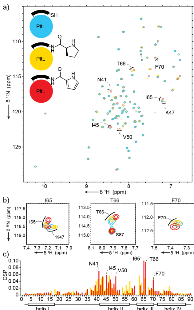
Figure 2. a, HSQC overlay of ^{15}\text{N} - holo -PltL, ^{15}\text{N} -prolyl-PltL, ^{15}\text{N} -pyrrolyl-PltL. b, Highlights of ^{15}\text{N} -HSQC data, illustrating perturbations of residues I65, T66, and F70. c, CSP plots of ^{15}\text{N} -prolyl-PltL and ^{15}\text{N} -pyrrolyl-PltL relative to ^{15}\text{N} - holo -PltL.
