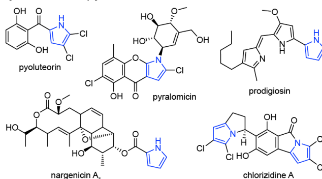
Figure 1. Structures of pyrrole containing natural products.
