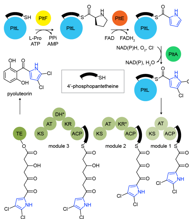
Scheme 1. Biosynthesis of pyoluteorin. Asterisks indicate inactive domain.
