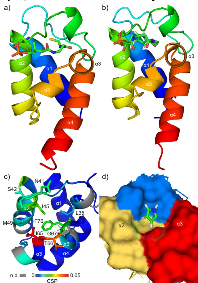
Figure 4. Solution NMR structures of PltL species. a, holo -PltL. b, pyrrolyl-PltL. c, Expanded view of pyrrolyl-PltL with colors corresponding to CSP values from Fig. 2. Key residues are labelled. CSPs not determined are shown in grey. d, Expanded view of surface-filled pyrrolyl-PltL structure illustrating pyrrole sequestration between the helix II/III cleft.
