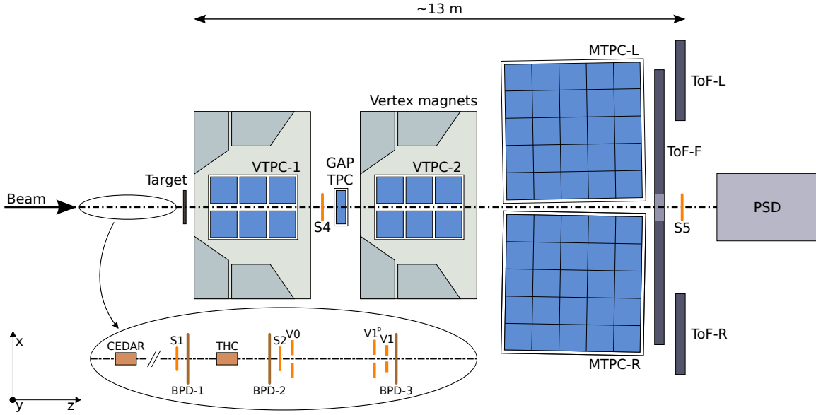
Fig. 1: (Colour online) The schematic layout of the NA61/SHINE experiment at the CERN SPS (horizontal cut, not to scale). The beam and trigger detector configuration used for data taking on p+p interactions in 2009 is shown. Alignment of the chosen coordinate system is shown on the plot; its origin lies in the middle of VT-PC-2, on the beam axis. The nominal beam direction is along the z axis. The magnetic field bends charged particle trajectories in the x - z (horizontal) plane. The drift direction in the TPCs is along the y (vertical) axis.
