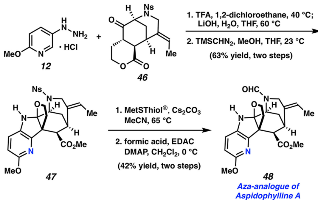
Figure 4. Synthesis of aza-analogues.
