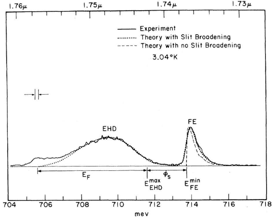
Figure 1.9: Photoluminescence spectrum of free electrons (FE) and electron-hole droplets (EHD) for bulk Ge as a function of laser energy (bottom scale) and wavelength (top scale). Solid line, small dashed line, and large dashed line represent experimental data, calculations based on electron-hole droplet theory with slit broadening, and calculations based on electron-hole droplet theory without slit broadening, respectively. E_F is the Fermi energy of the liquid, \phi_s is the condensation energy, E_{EHD}^{max} and E_{FE}^{min} are the maximum EHD energy and minimum FE energy, respectively. Measurements were performed at 3.04K. Adapted from Lo et al. 18 .
