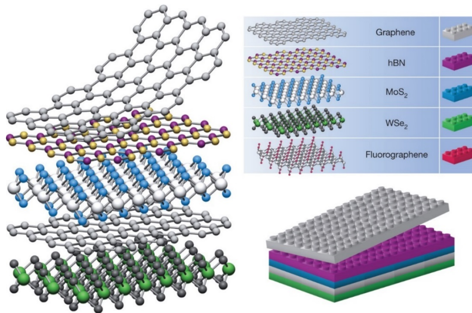
Figure 2.7: Schematic of van der Waals heterostructure assembly with a variety of 2D material constituents. Adapted from Geim et al. 25 .
