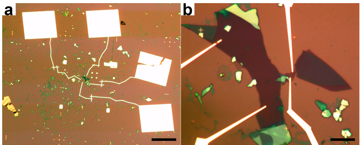
Figure 3.13: Optical images of a graphene-MoTe 2 -graphene optoelectronic device under (a) 5x (scale bar is 200 μm) and (b) 100x (scale bar is 10 μm) magnification.
