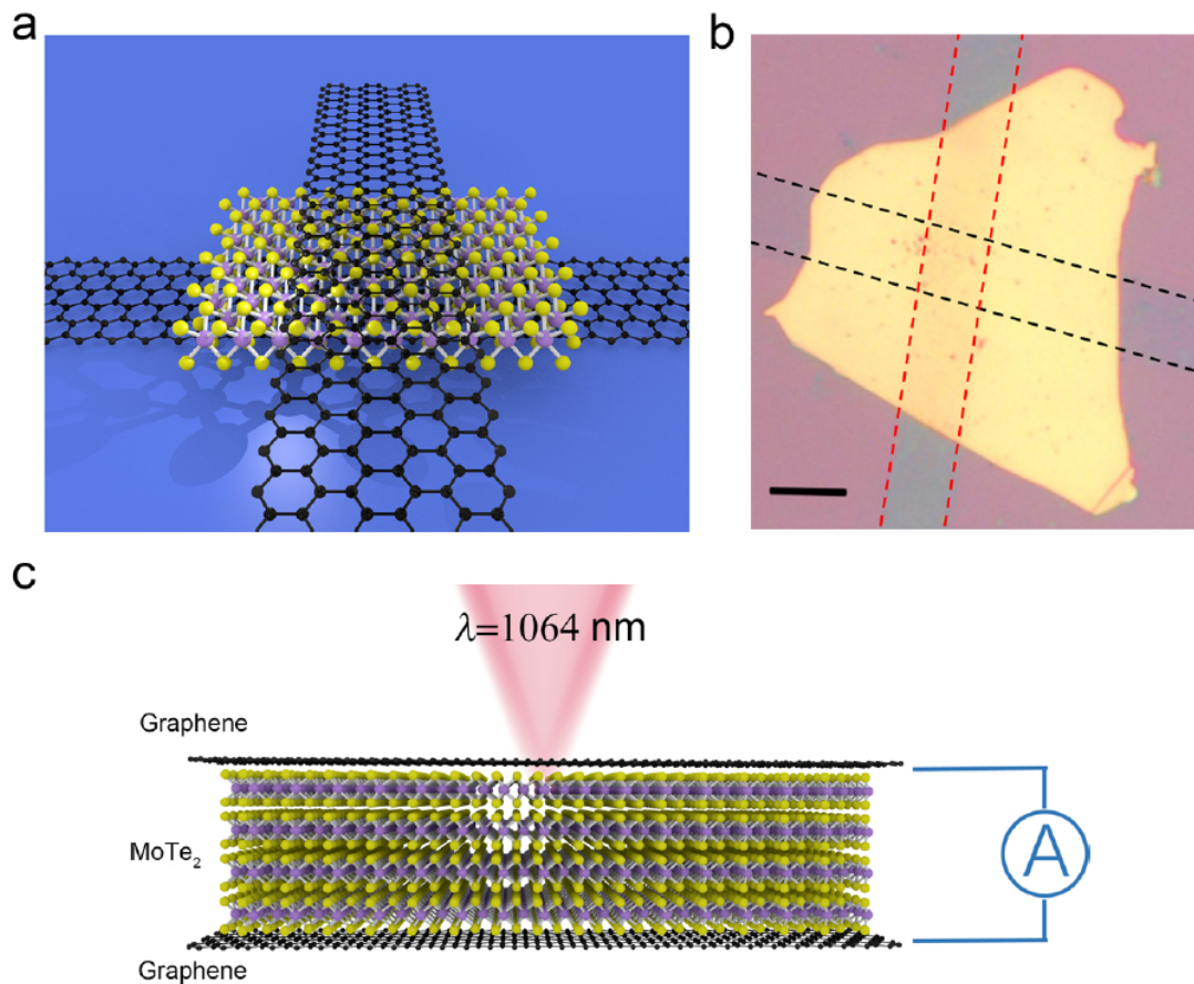
Figure 2.9: Graphene-MoTe 2 -graphene photodetector. (a) Schematic representation of the device. (b) Optical image of the device. Scale bar is 10 \mu\text{m} . (c) Side profile schematic of device showing laser illumination at \lambda = 1064 \text{ nm} and interlayer contacts attached to the top and bottom layers of graphene. Adapted from Zhang et al. 29 .
