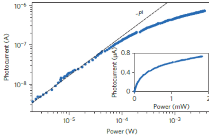
Figure 1.4: Power dependence of the interlayer photocurrent in a graphene-WSe 2 -graphene heterostructure. Dashed line indicates linear relationship. Inset, same power dependence data presented on a linear scale. Adapted from Massicotte et al. 5 .
