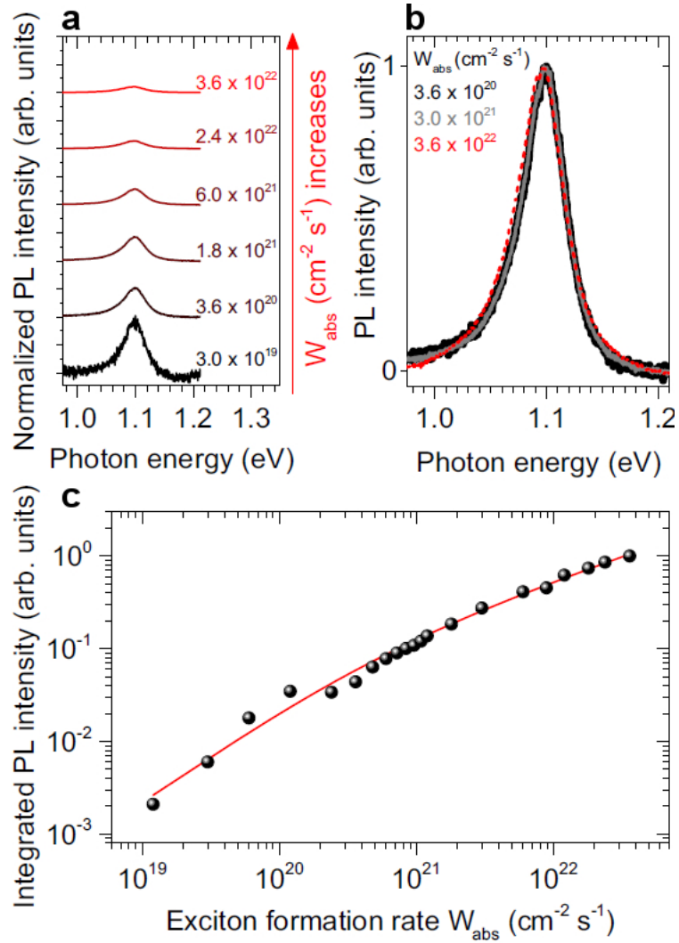
Figure 1.6: Photoluminescence of monolayer MoTe 2 . (a) MoTe 2 PL for increasing exciton formation rate, W_{\text{abs}} and also normalized by W_{\text{abs}} . (b) MoTe 2 PL for various exciton formation rates, normalized to unity. (c) Integrated MoTe 2 PL as a function of exciton formation rate (black circles). Red solid line indicates fit of exciton-exciton annihilation model to the data. Adapted from Froehlicher et al. 7 .
