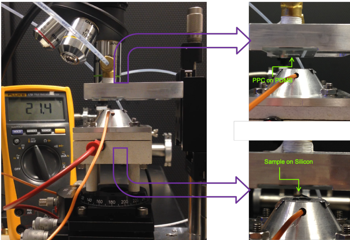
Figure 3.9: Optical image of a customized microscope system used in the dry transfer process of assembling graphene-MoTe 2 -graphene heterostructures. Left image, side profile of the microscope, showing all components. Upper right image, zoomed-in profile of the cantilever with stamp attached. Lower right image, zoomed-in profile of bottom sample stage.
