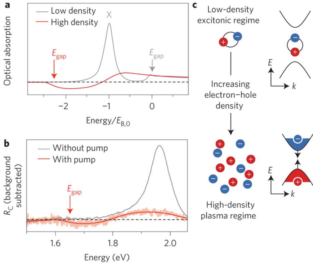
Figure 1.7: Optical absorption of bilayer WS 2 at high charge carrier density. (a) Predicted absorption vs. energy of an ultrathin TMD derived from many-body theory, where energy is normalized by the exciton binding energy E_{B,0} . Grey line indicates the predicted absorption at low electron-hole density while the red line represents the predicted absorption at high electron-hole densities. E_{gap} reflects the renormalized band gap at high carrier densities. (b) Experimental reflection contrast between sample and substrate vs. laser energy, with background response subtracted out from the data. Grey line indicates reflectance without pump pulse while light red data represents reflectance with pump pulse. Solid red line is a guide to the eye for the reflectance data in light red, determined by a smoothing function. E_{gap} denotes the renormalized band gap position. (c) Schematic of transition from a low-density excitonic regime to a high-density plasma. Adapted from Chernikov et al. 13 .
