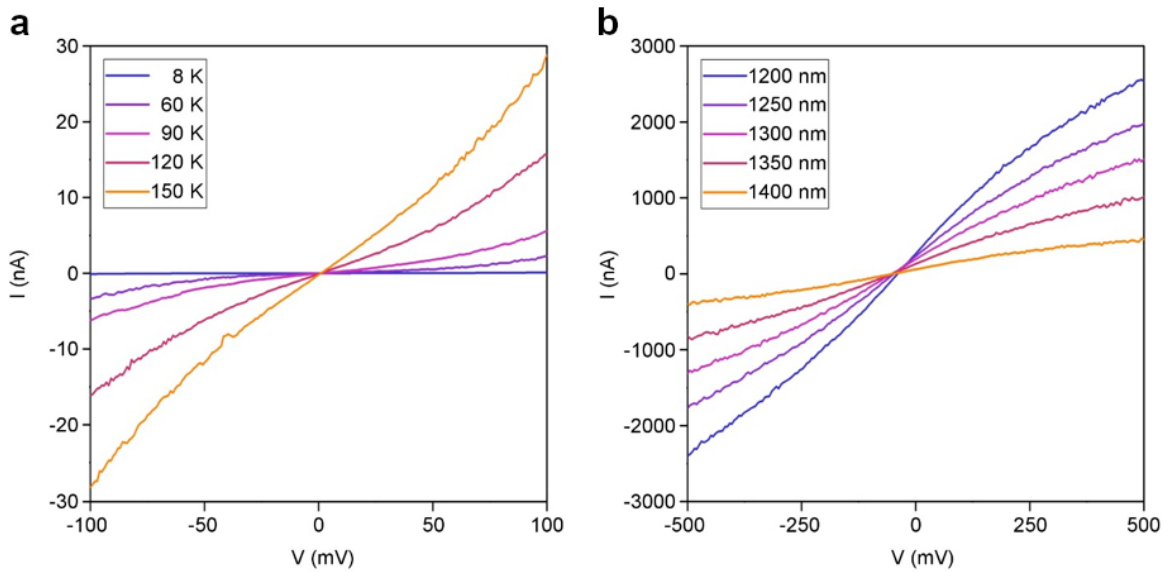
Figure 4.4: Temperature and wavelength dependence of I - V characteristics of a graphene-MoTe 2 -graphene photocell. (a) I - V curves as a function of temperature. Power = 23.0 mW, Wavelength = 1200nm. (b) I - V curves as a function of incident laser wavelength. Power = 4.80 mW, Temperature = 296 K.
