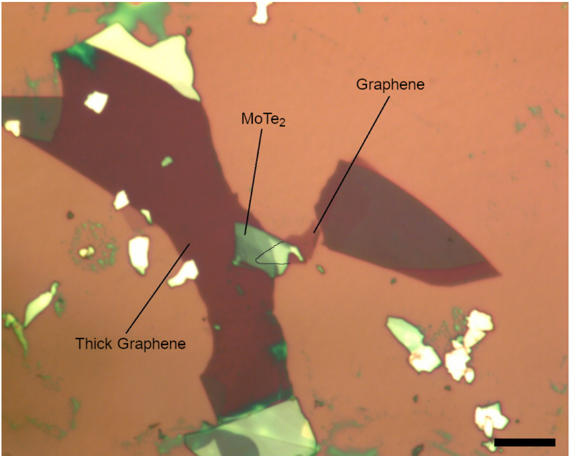
Figure 3.10: Optical image of a graphene-MoTe 2 -graphene heterostructure produced by dry transfer using a custom-built transfer microscope, with each layer labelled. Scale bar is 10 \mu\text{m} .
