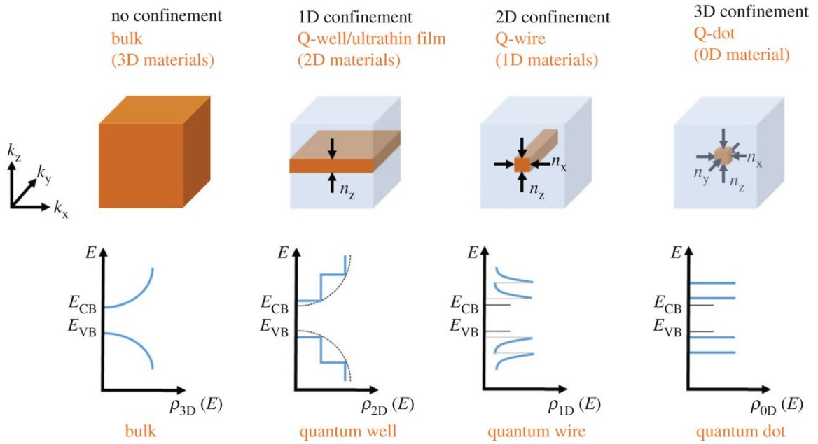
Figure 0.1: Schematic of physical form and density of states for increasing quantum confinement. Adapted from Edvinsson 1 .
