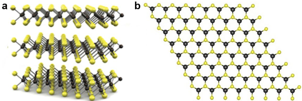
Figure 2.1: Crystal structure of hexagonal MoTe 2 . Mo atoms in black and Te atoms in yellow. (a) Side profile, revealing several atomic layers. (b) Top-down profile.
