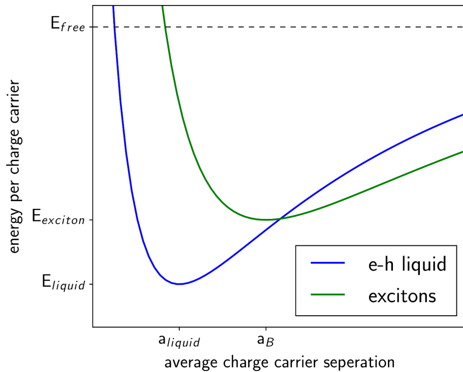
Figure 6.5: Schematic energy diagram for photoexcited carriers in MoTe 2 showing the energy curves for the e-h liquid and standard excitons.
