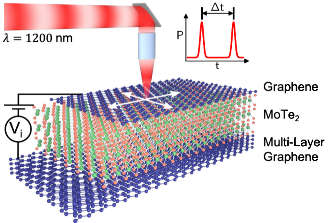
Figure 3.1: Schematic of graphene-MoTe 2 -graphene photocell with graphene layers labelled in blue and MoTe 2 layer labelled in green and orange. An ultrafast pulsed laser with \lambda = 1200 \text{ nm} photoexcites the device. White arrows indicate the spatial scanning capability of the laser. An interlayer bias potential, V_i , is applied vertically across the structure. Upper right inset, laser power P vs. time t , showing pulses separated by time delay \Delta t .
