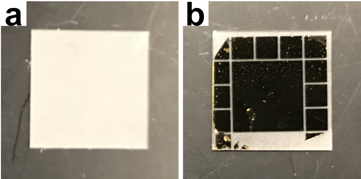
Figure 3.14: Optical images of a sapphire wafer (a) before and (b) after fabrication into a chip carrier for graphene-MoTe 2 -graphene optoelectronic devices.
