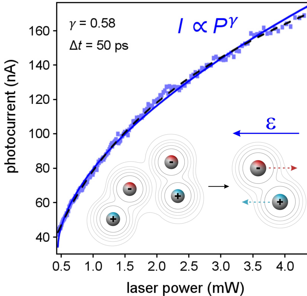
Figure 5.1: One-pulse photocurrent vs. optical power taken at a point in the center of the heterostructure (blue data). Solid blue line denotes the power law fit. Black dashed line shows the predicted power dependence of the photocurrent from the model. Inset, 2-particle Auger recombination results in one electron and one hole, which are swept away in the electric field \epsilon .
