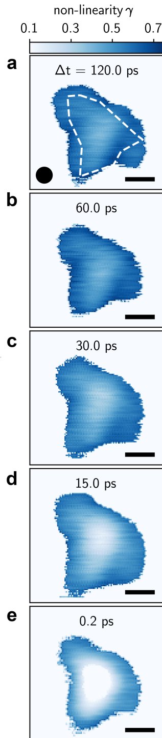
Figure 6.2: Spatial maps of nonlinearity \gamma(x, y) as a function of (a-e) two-pulse time delay \Delta t (labeled). Dashed line in a outlines the graphene-MoTe 2 -graphene heterostructure. Scale bars 3 \mu\text{m} . Black circle indicates the full width at half maximum of the diffraction-limited beamspot.
