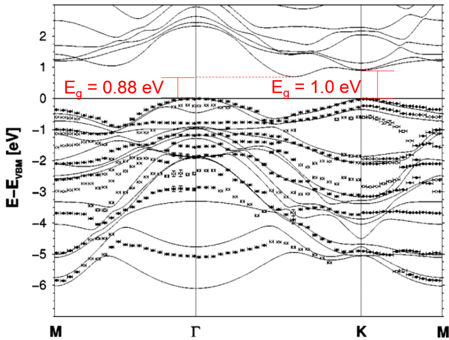
Figure 2.3: Calculations of MoTe 2 electronic band structure (solid lines) and experimental ARPES measurements of the valence band structure in MoTe 2 (symbols). Adapted from Boker et al. 23 .
