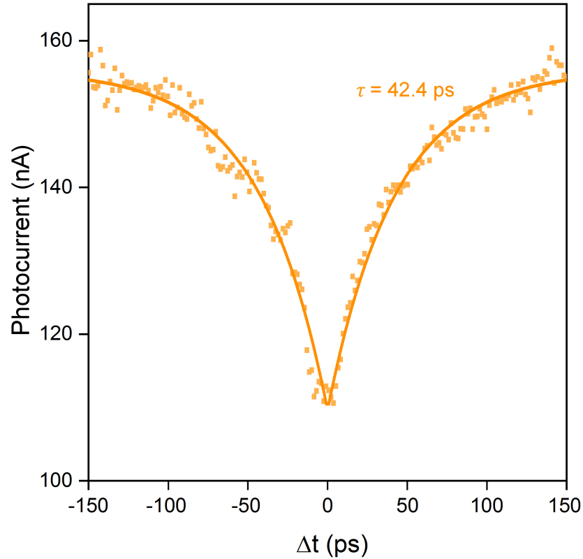
Figure 2.6: Photocurrent as a function of time delay in a graphene-MoTe 2 -graphene photocell at a laser power of 4.3 mW and no interlayer bias potential applied across the top and bottom layers of graphene. Orange symbols represent experimental data, and the orange solid line indicates a biexponential fit to the data.
