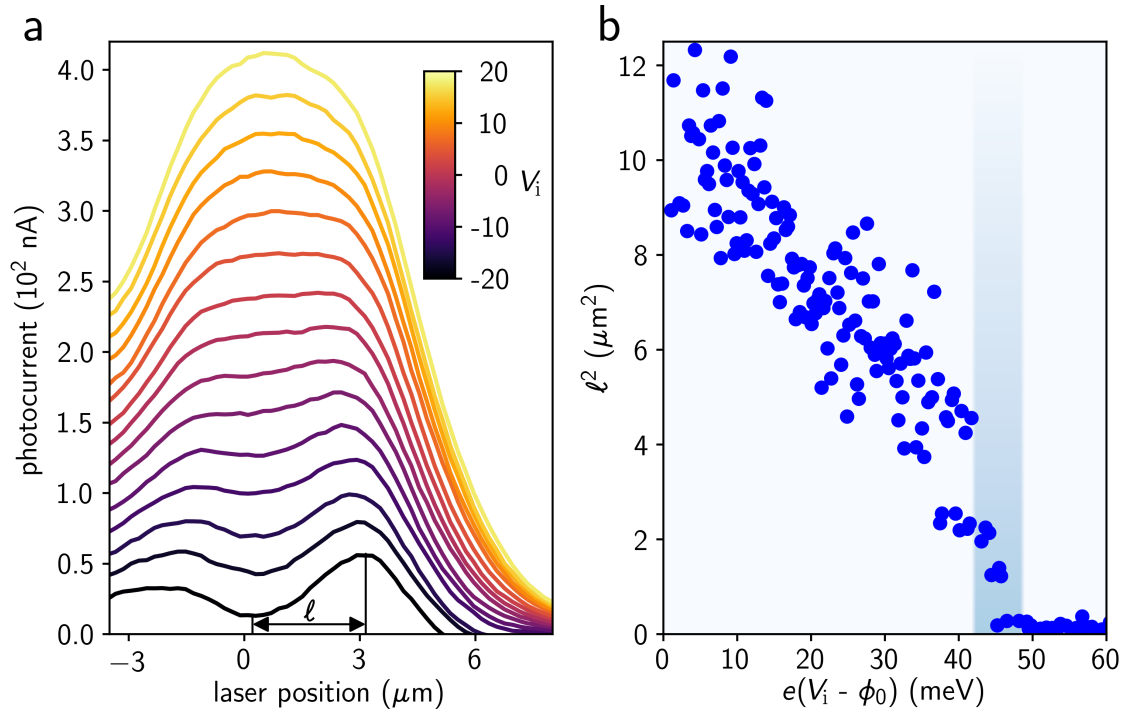
Figure 6.7: Interlayer voltage dependence of the 2D electron-hole liquid. (a) Spatial line cuts of the photocurrent as a function of interlayer voltage V_i ; \Delta t = 0.2 ps. (b) Photocurrent ring peak-to-valley distance \ell^2 vs. interlayer voltage. \phi_0 is the built-in potential of the graphene-MoTe 2 -graphene photocell.
