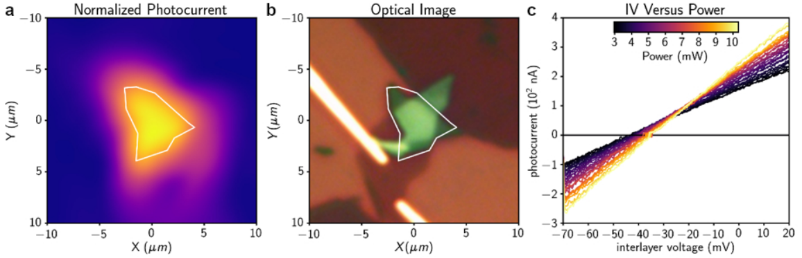
Figure 4.3: Optoelectronic I - V characteristics of a graphene-MoTe 2 -graphene photocell. (a) Spatial photocurrent map of device with heterostructure region outlined in white. (b) Optical image of region shown in a with overlap region outlined in white. (c) I - V curves as a function of laser power. Data taken at room temperature and a laser wavelength of 1200 nm.
