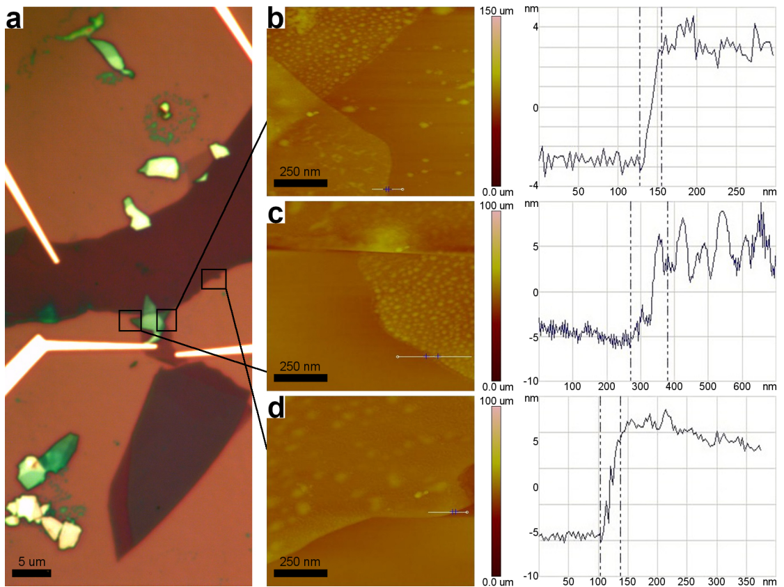
Figure 4.1: AFM of a graphene-MoTe 2 -graphene photocell. (a) Optical image of the device with boxes indicating areas where AFM scans were taken. (b), (c), (d) Left – AFM images of corresponding regions in (a) . White solid lines indicate regions where line traces were obtained, and blue crosses indicate the region over which the change in height was calculated. (b), (c), (d) Right – AFM line traces corresponding to images on the left.
