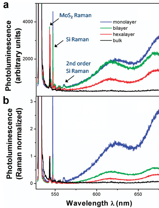
Figure 1.3: Thickness-dependent photoluminescence of a terraced MoS 2 flake. (a) Raw photoluminescence data. (b) Photoluminescence efficiency determined by normalizing the raw photoluminescence data in a with the Raman intensity. Adapted from Splendiani et al. 4 .
