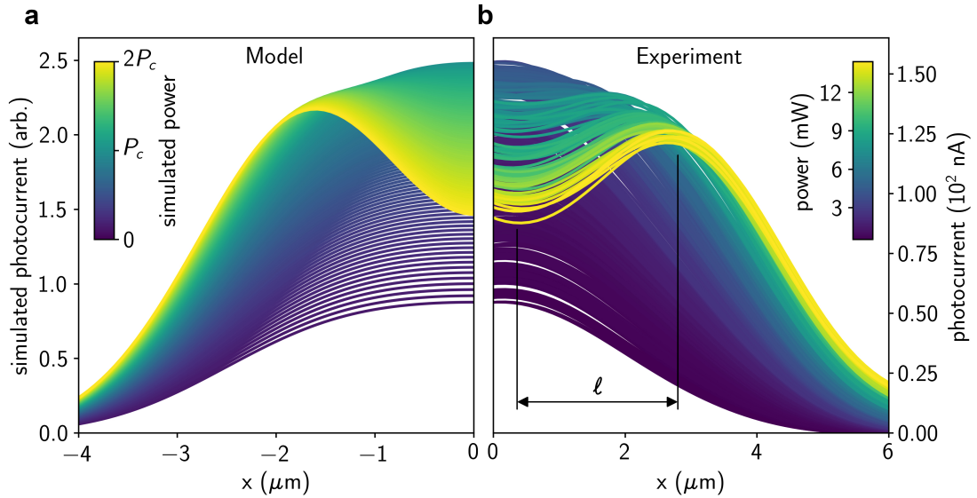
Figure 6.6: Room temperature 2D electron-hole liquid and comparison to spatial photocurrent imaging in the MoTe 2 photocells. (a) Calculated spatially resolved photoresponse of the electron-hole condensate showing the suppression of photocurrent in the center of the sample above the critical power P_c . (b) Photocurrent line profiles measured across the center of the sample for increasing power; T = 297 K, \Delta t = 0.2 ps.
