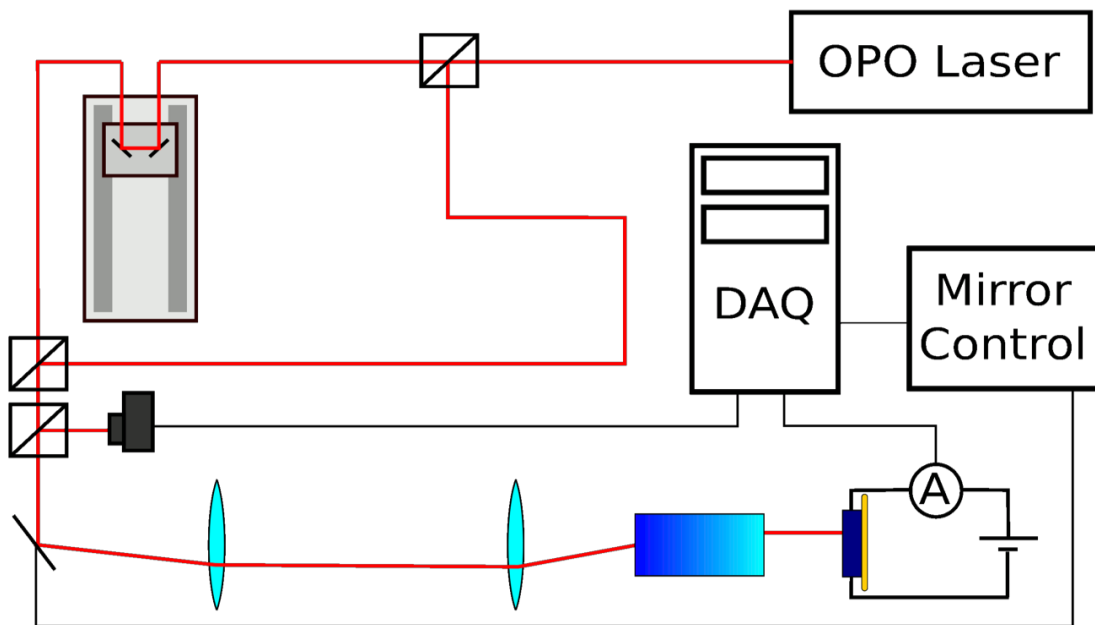
Figure 3.15: Schematic of ultrafast pulsed laser system and measurement apparatus.
