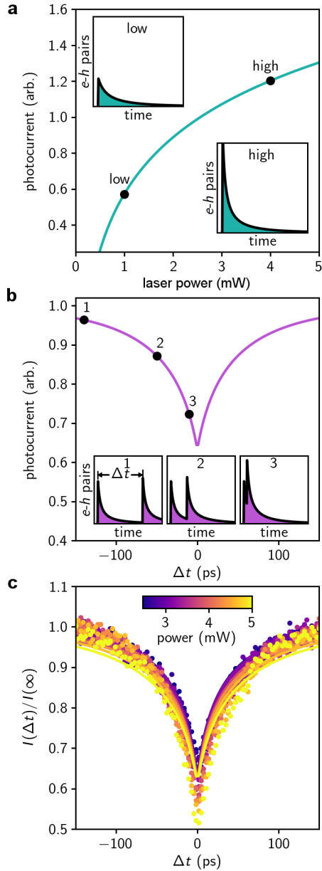
Figure 5.3: Two-particle electron-hole recombination model and comparison to infrared photocurrent in the G-MoTe 2 -G photocell. The solution of Eqn. 7 for a single laser pulse as a function of laser power (Eqn. 9) (a) and for two pulses as a function of two pulse time delay, \Delta t (Eqn. 8) (b) . The photocurrent is proportional to the integral of the number of e-h pairs versus time, shown in the insets, which is initially driven to a maximum value proportional to laser power, then exponentially decays. (c) Normalized photocurrent vs. \Delta t as a function of power (data) fitted to the model (solid lines), values for model parameters are extracted from these fits (supplementary materials of Arp, Pleskot et al. 33 ). All calculations in a and b use these values.
