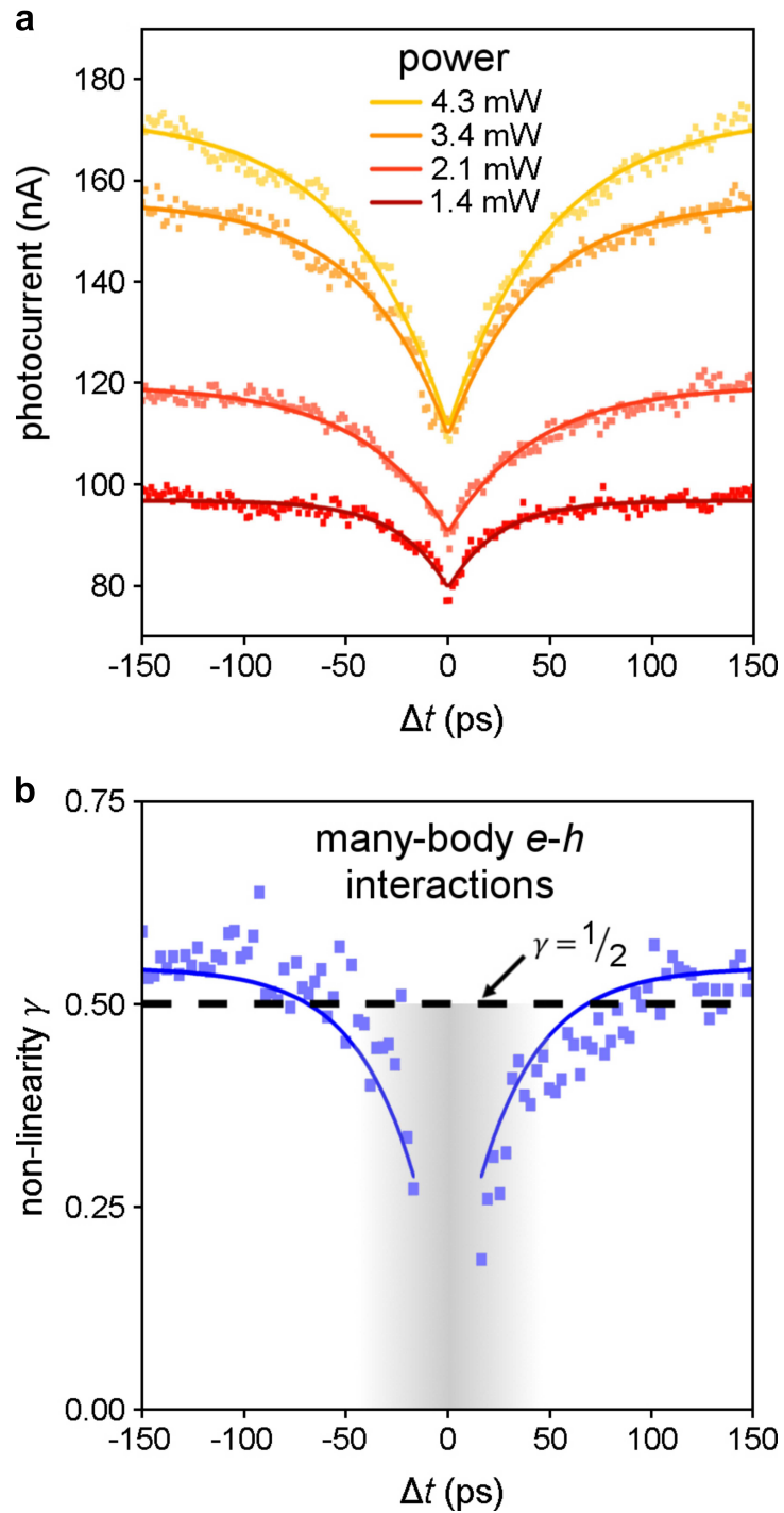
Figure 5.2: Dynamic photoresponse measurements of the vdW heterostructure photocell. (a) Example two-pulse photocurrent vs. time delay as a function of total (two-pulse) power. Solid lines represent exponential fits to the data. (b) Non-linearity \gamma vs. time delay (blue data). Solid blue lines represent an exponential fit to the data with a characteristic time constant of \tau = 29.8 ps. Black dashed line highlights \gamma = 0.5 .
