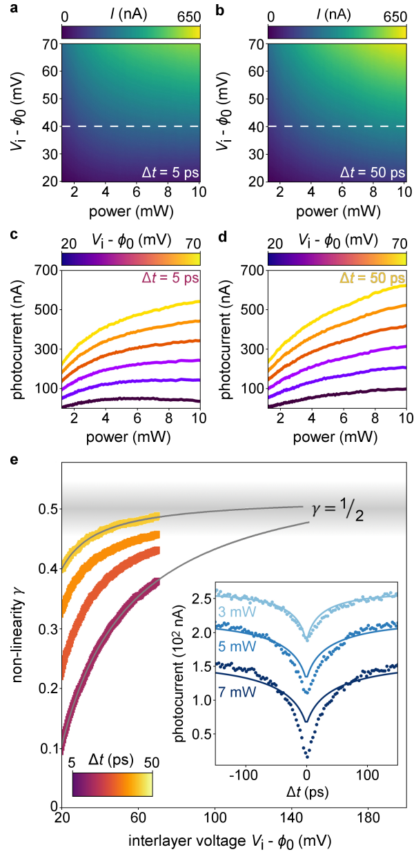
Figure 5.4: Interlayer voltage control of the competition between Auger recombination and charge carrier escape in the vdW heterostructure photocell. Photocurrent vs. optical power and interlayer voltage for time delay, \Delta t = 5 ps (a) and 50 ps (b) . White dashed lines represent line traces of photocurrent vs. power taken at a specific voltage from these datasets. Photocurrent vs. power as a function of interlayer voltage for time delay = 5 ps (c) and 50 ps (d) . (e) Non-linearity \gamma vs. interlayer voltage as a function of time delay. Solid grey lines denote rational fits of the data extended to 160 mV. Inset, photocurrent vs. time delay as a function of power, offset for clarity. Solid lines indicate fits from the model used to extract parameters \alpha and \tau_{es} .
