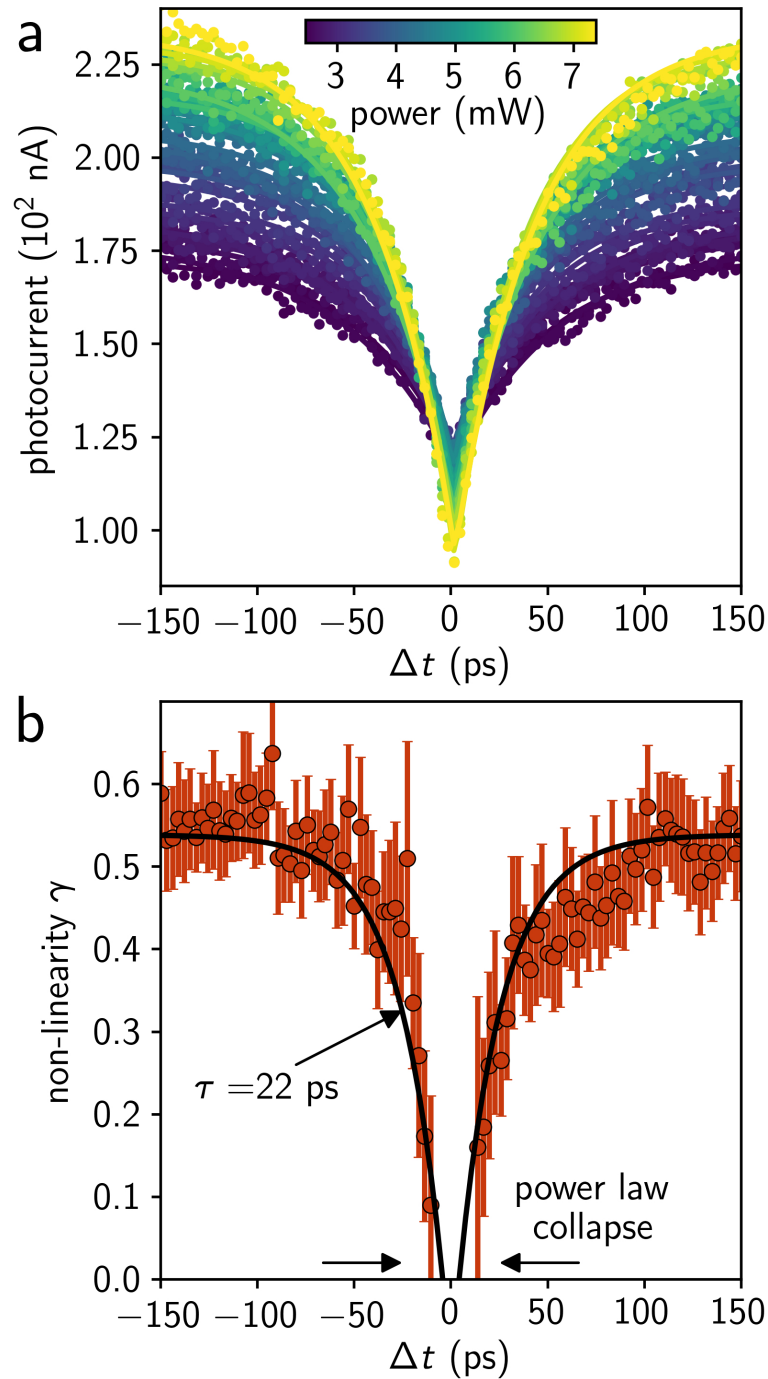
Figure 6.8: Dynamic photoresponse of the 2D electron-hole liquid. (a) Photocurrent vs. \Delta t for increasing optical power. The laser is fixed at the center of the device. Solid lines are exponential fits to the data at each power. (b) Power law exponent \gamma as a function of \Delta t , extracted by fitting the data in a to I \propto P^\gamma . Solid black line is an exponential fit with a characteristic time-scale \tau = 22 ps.
