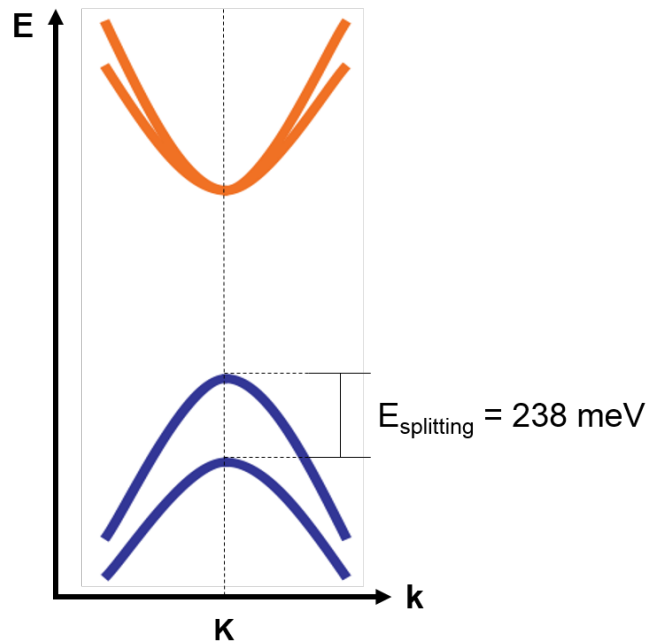
Figure 2.4: Schematic of MoTe 2 band structure at the K Brillouin point, highlighting the splitting of the valence band and high spin-orbit coupling. Adapted from Mak et al. 24 .
