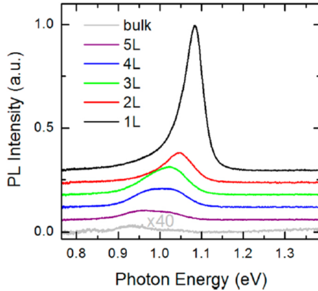
Figure 2.2: Photoluminescence spectra of MoTe 2 for various layer thicknesses ranging from monolayer (1L) to 5 atomic layers (5L), as well as bulk material. Spectra are shifted vertically for clarity. Adapted from Ruppert et al. 22 .
