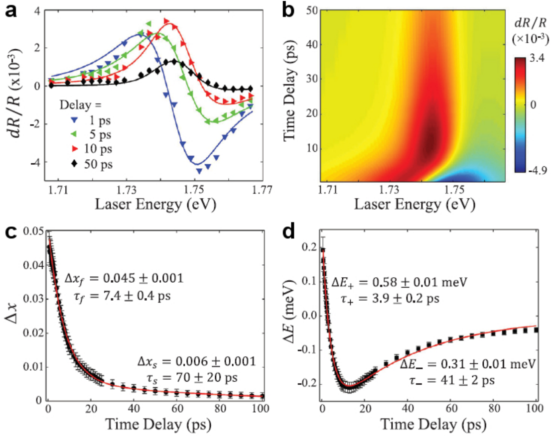
Figure 1.8: Ultrafast reflectance spectroscopy and exciton optical susceptibility model of monolayer WSe 2 . (a) Experimental dR/R spectra (symbols) for various time delays. Solid lines represent fits of model derived from Equation (4) to data. (b) Calculated dR/R from the model as a function of both time delay and laser energy. (c) and (d) are plots of fit parameters \Delta x and \Delta E from the model (symbols) as a function of time delay, respectively. Solid red lines indicate biexponential fits according to Equation (5). Adapted from Aivazian et al. 14 .
