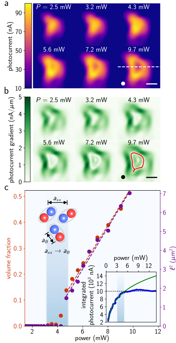
Figure 6.3: Critical onset of ring-like photoresponse revealed in analysis of spatial photocurrent maps. (a) Spatially resolved photocurrent measured at various powers (labeled) and \Delta t = 0.2 ps. Dashed line indicates location of photocurrent line profiles. (b) Photocurrent gradient |\nabla I| calculated from photocurrent maps in a . The contour |\nabla I| \approx 0 encloses the photocurrent ring (red contour in the image at P = 9.7 mW). Scale bars 5 \mu\text{m} , circles indicate the beamsport FWHM. (c) Photocurrent ring volume fraction (red data) vs. laser power. Volume fraction is the ratio of the volume enclosed by the |\nabla I| \approx 0 contours to the active photocell volume (area). Peak-to-valley distance \ell (purple data) vs. optical power extracted from photocurrent line cuts in a . Red (purple) dashed lines are linear fits to volume fraction ( \ell^2 ) vs. optical power above P = 6 mW. Inset top, inter-exciton spacing a_{xx} approaches the exciton Bohr radius a_B . Inset bottom, spatially integrated photocurrent vs. power (blue data) and power law fit below 6 mW (solid green line).
