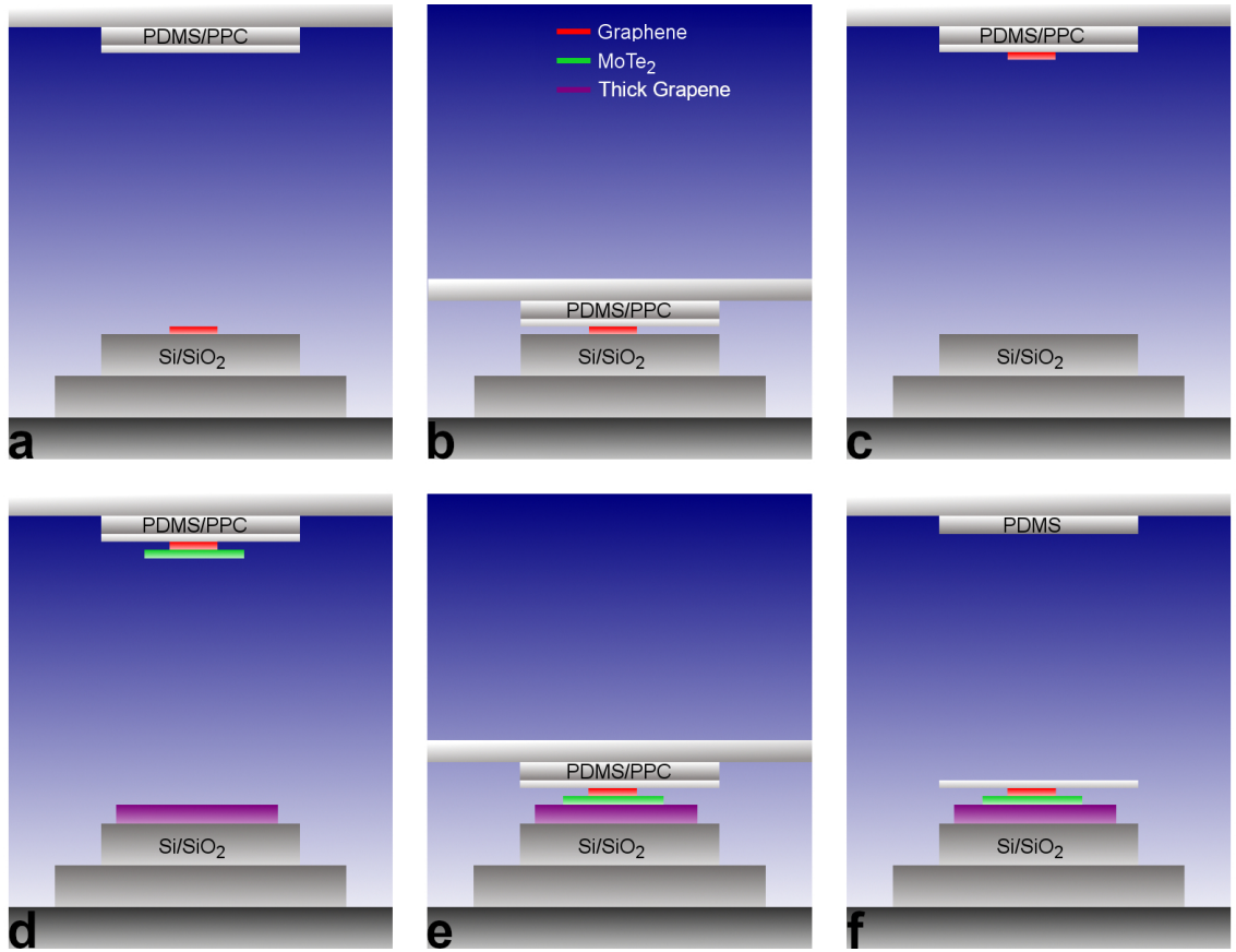
Figure 3.11: Schematic of standard method of dry transfer assembly of graphene-MoTe 2 -graphene heterostructures. (a) Initially, a graphene flake is placed on the sample stage and a stamp is made consisting of a glass slide, PDMS, and PPC. (b) The stamp is lowered until it encounters the graphene on the sample stage. (c) After heating the stage to 40°C and allowing it to cool back to room temperature, the stamp is quickly removed from the stage, picking up the graphene flake. (d) The same procedure is used to pick up the next layer of MoTe 2 , and then the final layer of graphene is placed on the sample stage. (e) The flakes are aligned on top of each other and the stamp is lowered until it contacts the stage. (f) The stage is heated to 80°C to melt the PPC layer, and the stamp is raised slowly to allow the PPC to separate from the PDMS, leaving the completed heterostructure on the desired substrate. The PPC layer is then removed in an acetone bath.
