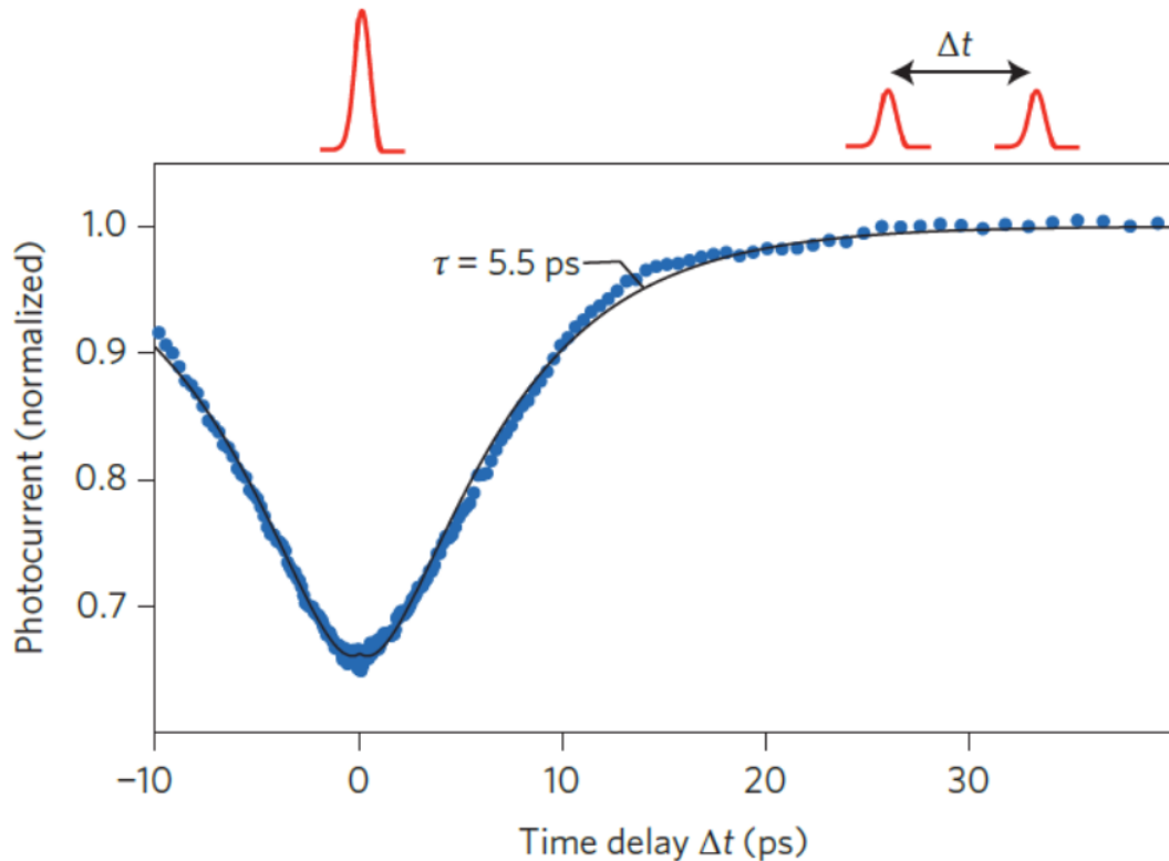
Figure 2.5: Photocurrent as a function of time delay in a graphene-WSe 2 -graphene photocell at a laser power P = 300 \mu\text{W} and an interlayer bias potential applied across the top and bottom layers of graphene V_B = 1.2 \text{ V} . Blue dots indicate experimental data and black solid line represents biexponential fit to the data. The laser profile is displayed above the plot both at short and long time delays. At short time delay, the two pulses overlap to generate a single intense pulse. At long time delay, the two smaller pulses are separated by \Delta t . Adapted from Massicotte et al. 5 .
