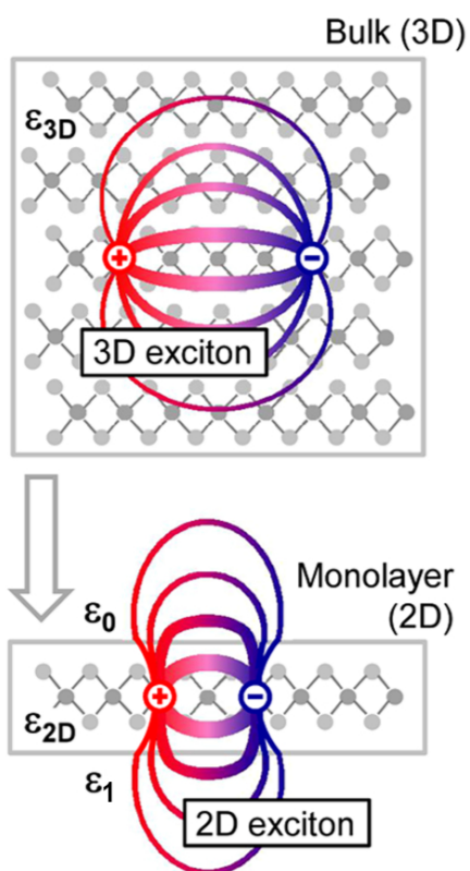
Figure 1.2: Schematic of an exciton and associated electric field lines in a bulk 3D material compared to a 2D monolayer. \epsilon_{3D} is the bulk dielectric constant, whereas \epsilon_{2D} is the 2D dielectric constant. \epsilon_0 and \epsilon_1 are dielectric constants of a surrounding vacuum medium and underlying substrate, respectively. Adapted from Chernikov et al. 2 .
