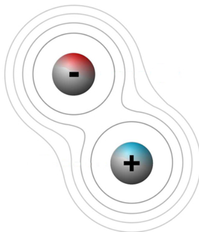
Figure 1.1: Schematic of an exciton containing a single electron and hole, with electric field lines extending from each.
