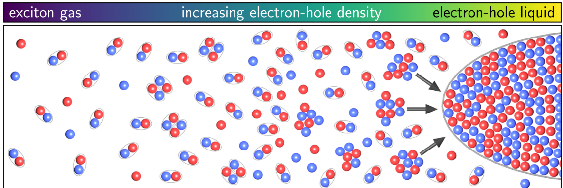
Figure 6.4: Evolution of electron-hole interactions with increasing e-h density. As density increases, the non-interacting gas of excitons gives rise to exciton-exciton interactions, eventually leading to condensation into a 2D electron-hole liquid.
