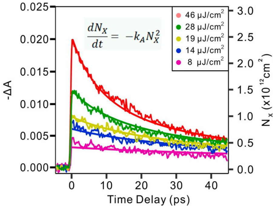
Figure 1.5: Change in photoluminescence absorbance and exciton dynamics for various pump fluences. Solid lines represent fits to the raw data (jagged lines) according to top equation, also Equation (1) below. The right axis denotes the scale of photoexcited excitons derived from the model. Adapted from Sun et al. 6 .
