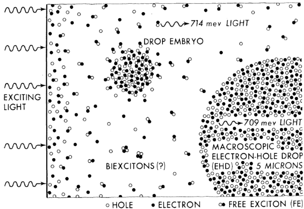
Figure 1.10: Schematic of electron-hole liquid droplet formation out of a gas of photoexcited excitons and free electrons and holes. Adapted from Jeffries 15 .
