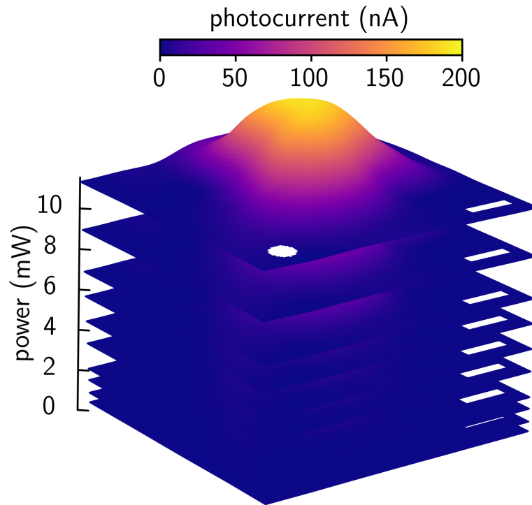
Figure 6.1: Spatial photocurrent maps for increasing laser power. Wavelength \lambda = 1200 nm, T = 297 K, and time delay \Delta t = 120 ps. Scale bars 3 \mu\text{m} . White circle indicates the full width at half maximum of the diffraction-limited beamspot.
