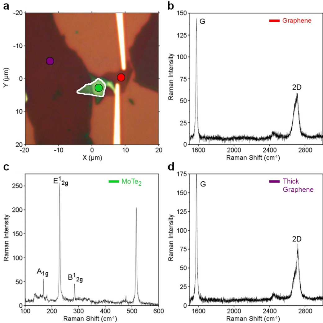
Figure 4.2: Raman spectroscopy of a graphene-MoTe 2 -graphene photocell. (a) Optical image of the device with top graphene, MoTe 2 , and bottom graphene layers indicated with color-coded markers. White outline indicates region of 3-layer overlap. (b), (c), (d) Raman spectra of the top graphene, middle MoTe 2 , and bottom graphene layers, respectively, taken at the position of the corresponding markers in (A).
