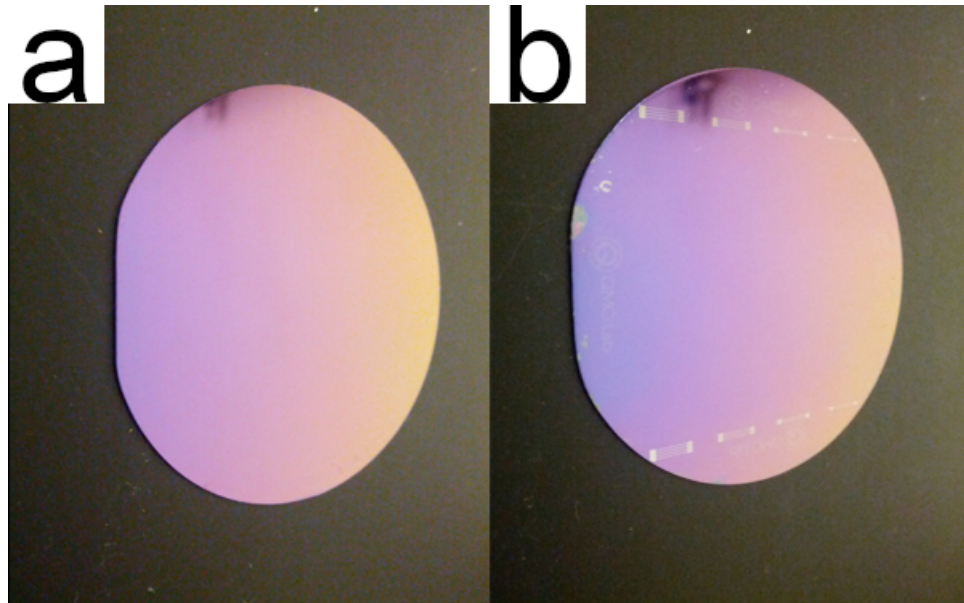
Figure 3.2: Si wafers used as substrates for graphene-MoTe 2 -graphene heterostructures. (a) Commercial 2-inch diameter Si/SiO 2 wafer with a 290 nm oxide. (b) Same Si wafer with etched identifying markers used to locate ultrathin flakes or devices.
