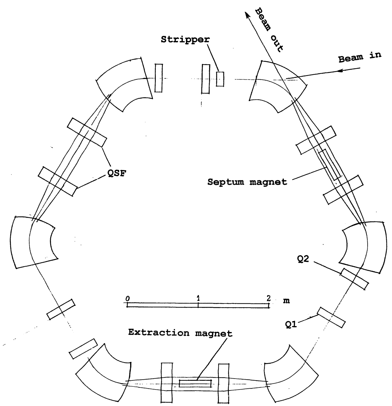
Fig.1 Ring for enhancing output of stripper
