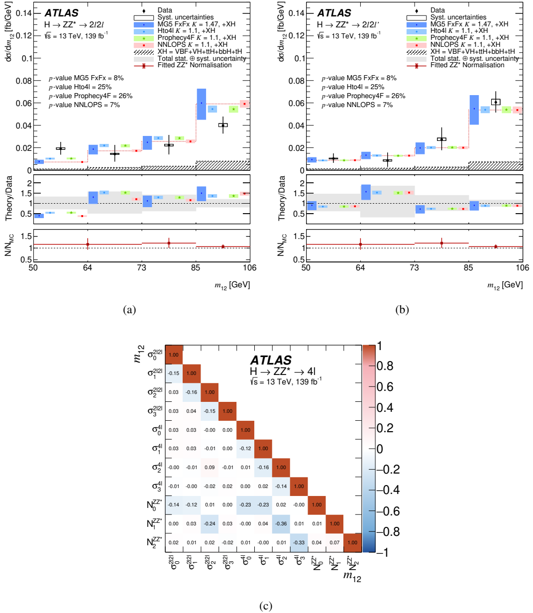
Figure 43: Differential fiducial cross sections for the invariant mass m_{12} of the leading Z boson in (a) the 4\mu and 4e decay channels and (b) the 2e2\mu and 2\mu 2e decay channels. The corresponding correlation matrix is shown in (c).
