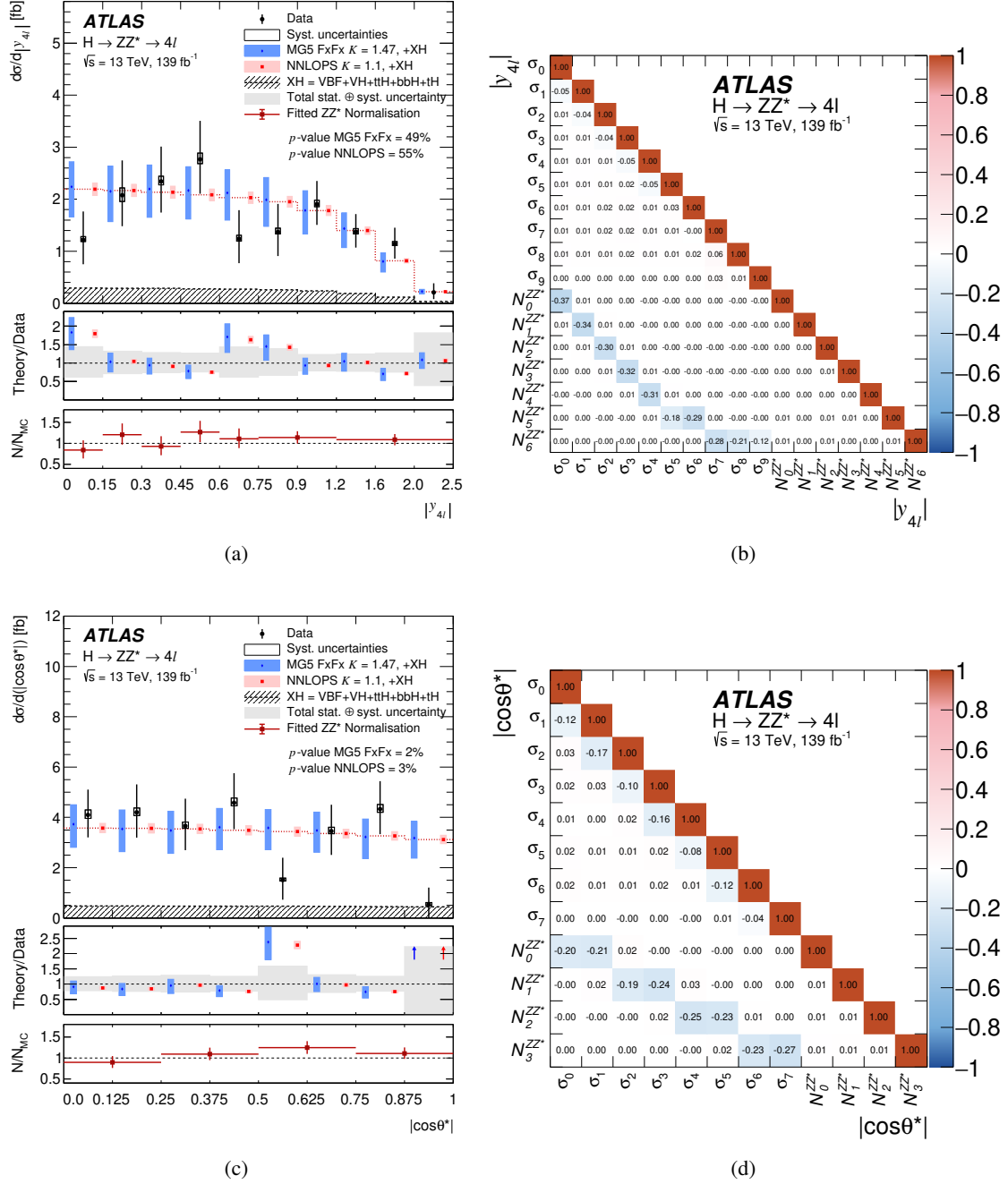
Figure 21: Differential fiducial cross-sections for (a) the rapidity, |y_{4\ell}| , of the Higgs boson and (c) the production angle, |\cos \theta^*| , of the leading Z boson. The corresponding correlation matrices between the measured cross sections and the ZZ^* background normalisation factors are also shown (b) and (d).
