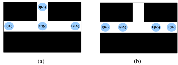
Fig. 1. Instances of multi-robot motion planning problem
