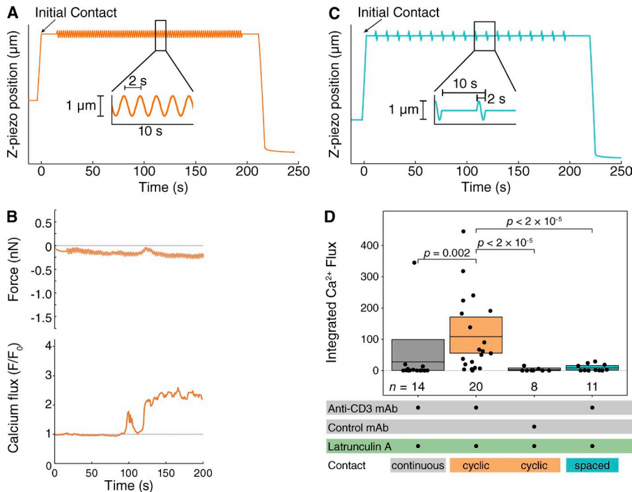
Figure 4. Application of cyclical force rescues Ca 2+ flux in LatA-treated cells. (A) Z-position of cantilever during application of cyclical force. The ramp-up indicates lowering of the cantilever until the contact. The cantilever is held in place for 15 s and then begins a sinusoidal movement with amplitude 0.5 \mu\text{m} and period 2 s. After 180 s, the tip is again held constant for 15 s, then retracted. (B) Time courses for force on the cantilever and normalized Fluo-4 intensity for a cell treated with LatA subjected to the cyclical force in A. (C) Z-position of cantilever during the spaced cyclic force. Sinusoidal pulses from A were spaced out with constant dwells lasting 8 s, resulting in a waveform with a 10-s period. (D) Time-integrated calcium flux for LatA-treated cells with no external force, continuous cyclical force, with a spaced cyclical force or cyclical force with an irrelevant antibody. Data were pooled for LatA continuous contact (same points as Fig. 3 D), LatA cyclic contact ( n = 20 cells from five independent experiments), LatA cyclic contact with control antibody ( n = 8 cells from two independent experiments), and spaced cyclic contacts ( n = 11 from two independent experiments). Box shows the mean and 95% CI.
