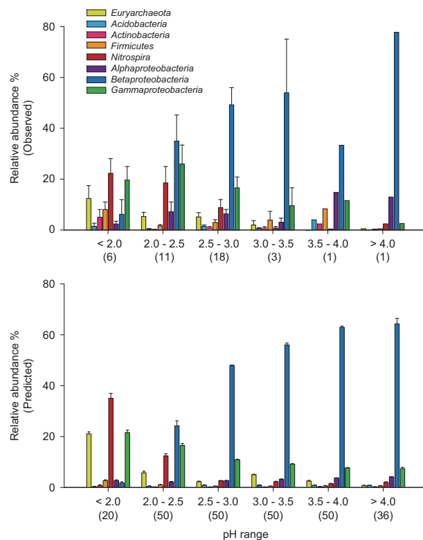
Figure 4 The comparison of predicted and observed relative abundances (%) of dominant lineages along the gradient of pH levels. Values were mean \pm s.e. and the numbers in bracket indicate the number of samples that considered in each pH group.
