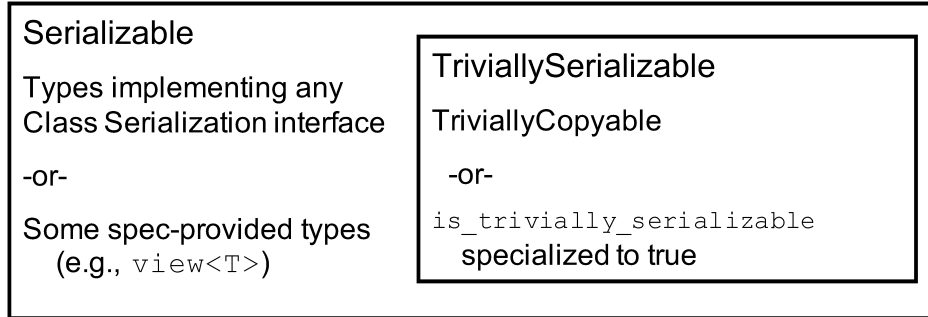
Figure 4: Serialization Concepts.
