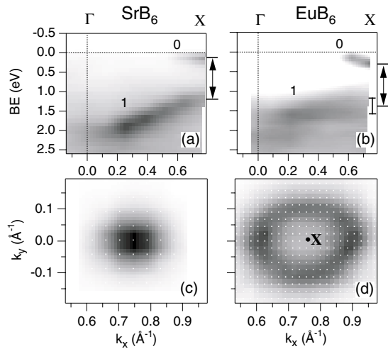
FIG. 2. Near- E_F valence band structure for (a) \text{SrB}_6 and (b) \text{EuB}_6 along \Gamma - X showing small band 0 electron pockets above the X -point gap to band 1. E_F intensity maps of the X -point at h\nu = 30 eV for (c) \text{SrB}_6 and (d) \text{EuB}_6 showing differing electron pocket sizes.
