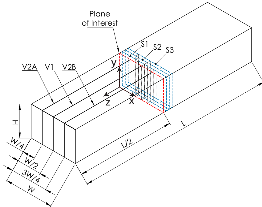
Fig. 2 – Dimensioned diagram of the measurement article with the location of measurement planes ( W=77.8 mm, H=51.2 mm, and L=304.8 mm). The biaxial measurement plane is at z = 0 mm and the three confirmation measurements (V1, V2A and V2B) are at x = 38.9 mm, 19.45 mm, and 58.35 mm. Three slices were removed adjacent to the plane of interest by cutting at z = -5 mm (S1), -10 mm (S2), and -15 mm (S3). Each slice has a slitting measurement at the mid-width of the slice and at \pm 10 mm (S1), \pm 15 mm (S2), and \pm 20 mm (S3) from the mid-width.
