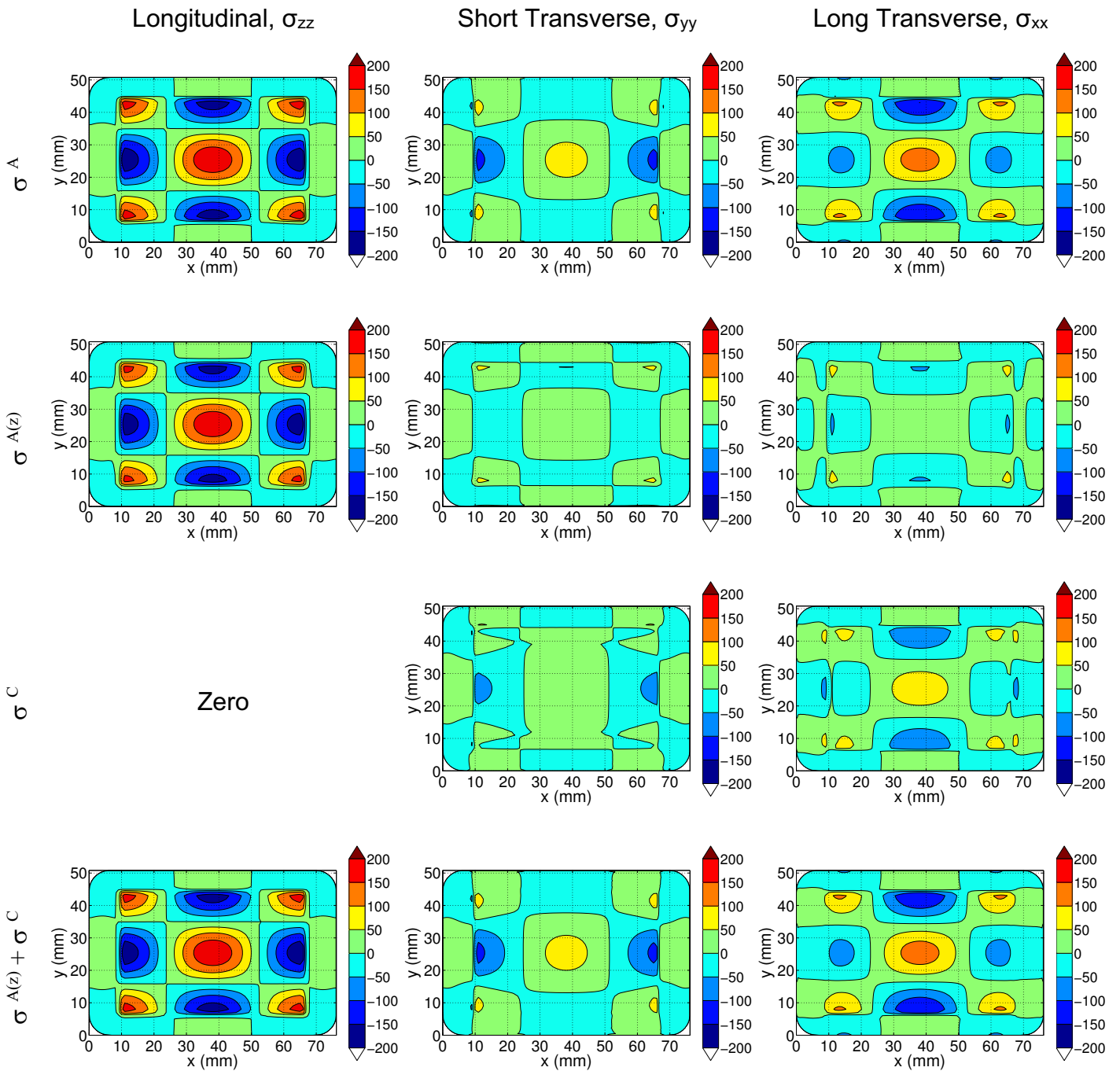
Fig. 3 – Contour plots of the initial stress ( \sigma^A ) (top row), the effect of the longitudinal stress in the slice ( \sigma^{A(z)} ) (second row), the stress remaining in the slice ( \sigma^C ) (third row), and the sum of \sigma^{A(z)} and \sigma^C (bottom row) for each stress component
