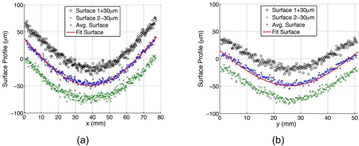
Fig. 6 – Measured surface displacements along the (a) horizontal direction at mid-vertical dimension and (b) vertical direction at mid-horizontal dimension. Note: the data from surface 1 is offset by 30\ \mu\text{m} and the data from surface 2 is offset by -30\ \mu\text{m} , so that the average and fit are also visible on the same plot
