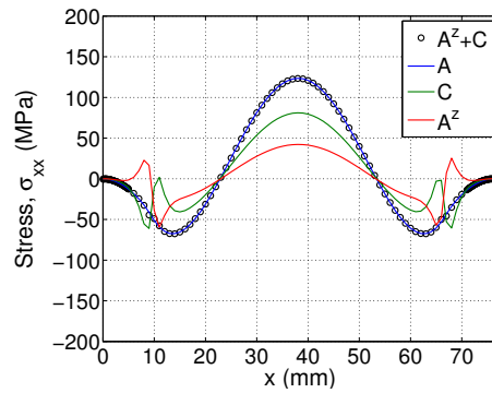
(c) Long Transverse, \sigma_{xx}
