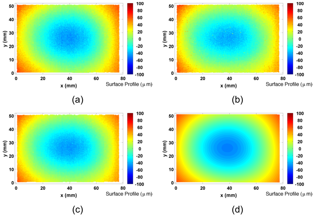
Fig. 5 – Measured surface displacement from the contour method measurement. (a) Surface “1”, (b) surface “2”, (c) averaged surface, and (d) fitted surface
