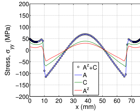
(b) Short Transverse, \sigma_{yy}
