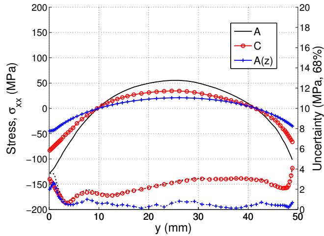
Fig. 10 – Stress and uncertainty of the two contributions to the transverse stress measurement and the total ( \sigma^A ), at a horizontal position of 18.9 mm. Uncertainty is shown as dotted lines
