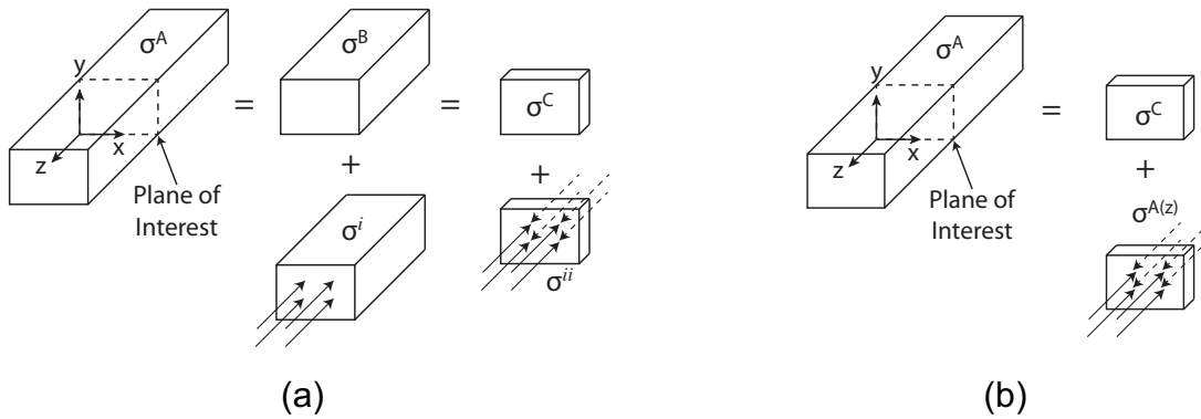
Fig. 1 – Stress decomposition diagrams. (a) The original stresses ( \sigma^A , all stress components, at the plane of interest) are equal to the stress release from cutting the part in half ( \sigma^i ), the stress released when removing a thin slice ( \sigma^{ii} ), and the stress remaining in the slice ( \sigma^C ). (b) The original stress ( \sigma^A ) is equal to the stress remaining in a thin slice ( \sigma^C ) plus the effect of total longitudinal stress on the thin slice ( \sigma^{A(z)} )
