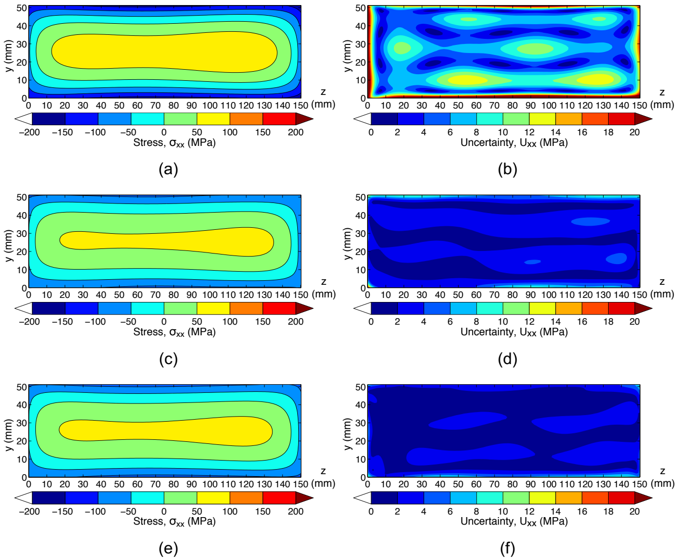
Fig. 11 – Measured transverse stress and uncertainty (68% confidence interval) at x = 38.9\text{mm} ((a) and (b)); x = 18.9\text{mm} ((c) and (d)); and x = 58.9\text{mm} ((e) and (f))
