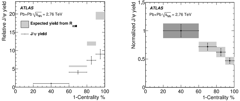
Fig. 3. Left: Relative J/\psi yield as a function of centrality normalized to the most peripheral bin shown as black dots with errors. The expected relative yields, obtained assuming a scaling with a number of binary collisions, are also shown as boxes reflecting 1\sigma systematic uncertainties. Right: Normalized J/\psi yield as a function of centrality. The statistical errors are shown as vertical bars while the gray boxes also include the combined systematic errors. Uncertainties from the most peripheral bin are not propagated to higher centrality bins.
