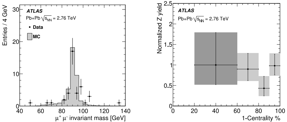
Fig. 4. Left: Di-muon invariant mass distribution after the selection described in the text. Right: Normalized Z yield as a function of centrality for 38 selected Z candidates. The statistical errors are shown as vertical bars while the gray boxes also include the combined systematic errors. The uncertainties in the most peripheral bin are not propagated to higher centrality bins.
