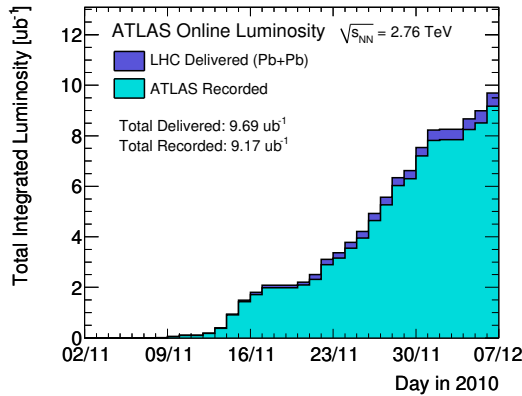
Fig. 1. Cumulative integrated luminosity versus day, delivered to (dark gray/dark blue) and recorded by (light gray/light blue) ATLAS for lead–lead collisions during stable beams and for 2.76 TeV center-of-mass energy per nucleon pair.
