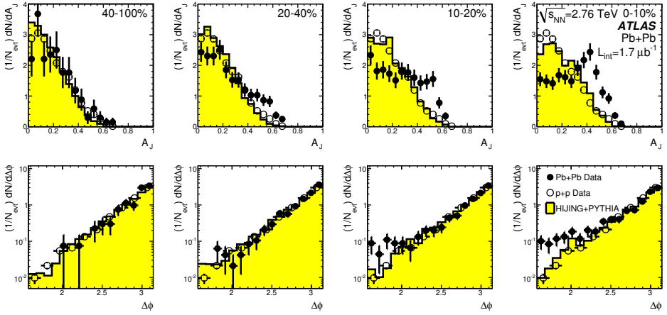
Fig. 2. Top: Dijet asymmetry distribution A_J for lead–lead data (solid points) and unquenched HIJING with superimposed PYTHIA dijets (solid gray (yellow) histograms), as a function of collision centrality (left to right from peripheral to central ones). Proton–proton data at \sqrt{s} = 7 TeV, analyzed with the same jet selection, is shown as open circles. Bottom: Distribution of the azimuthal angle separation \Delta\phi between two jets, for data and HIJING + PYTHIA, also as a function of centrality.
