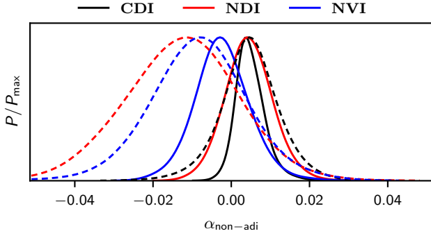
Fig. 38. Posterior probability density of the observable non-adiabatic fraction of the CMB temperature variance, assuming a generally correlated mixed adiabatic and isocurvature model. These results used Planck TT+lowE+lensing data (dashed lines) and TT,TE,EE+lowE+lensing data (solid lines).
