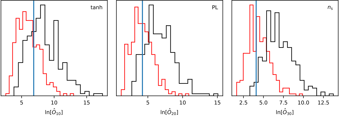
Fig. 47. Histograms of the quantity \hat{O}_{j0} for the tanh, power-law, and n_s gradient modulation models using Planck temperature data combined with 300 statistically isotropic polarization simulations (red outlines) or 300 polarization simulations modulated according to the best-fit parameters from the temperature data (black). The blue lines indicate the values for the actual SMICA polarization data. A large value relative to the isotropic (red) simulations would indicate that the modulation model is preferred over \Lambda CDM.
