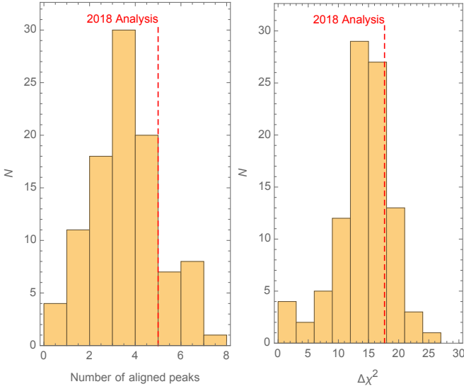
Fig. 34. Left: Number of aligned peaks in the power spectrum and the bispectrum for the log feature model. Right: Mean improvement of those same peaks in 100 simulated bispectra combined with the unbinned high- \ell likelihood.
