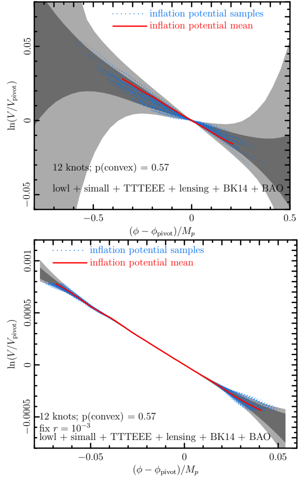
Fig. 27. Top: Reconstructed shape of the single-field inflaton potential from the cubic-spline power spectra mode-expansion using 12 knots and the Planck TT,TE,EE+lowE+lensing+BK14+BAO data. Bottom: Result when r is fixed at 0.001. Instead of plotting as a function of wavenumber k we plot \ln V(\phi)/V_{\text{pivot}} about a pivot field value \phi_{\text{pivot}} . Note that the range on the \phi axis is quite different for the small r case than the floating case.
