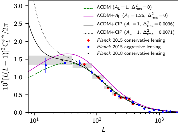
Fig. 44. Conservative Planck 2015 lensing data (red points), aggressive Planck 2015 lensing data (blue points with error bars), and conservative Planck 2018 lensing data (black points in grey boxes), along with the best-fit models to the Planck data: the best-fit adiabatic \Lambda CDM model to 2018 TT+lowE (green dashed line); the best-fit \Lambda CDM+ A_L model to 2018 TT+lowE (magenta solid line, A_L = 1.26 ); and the best-fit \Lambda CDM+CIP model to 2018 TT,TE,EE+lowE and conservative lensing data (black solid line, \Delta_{\text{rms}}^2 = 0.0036 ) and to 2015 TT,TE,EE+lowP and conservative lensing data (black dotted line, \Delta_{\text{rms}}^2 = 0.0071 ). As CIP modifies only the very low- L part of the lensing power spectrum, the conservative 2015 lensing data ( 40 \leq L \leq 400 ) are insensitive to CIP even when \Delta_{\text{rms}}^2 = 0.0071 . On the other hand, the first two data points of the 2015 aggressive lensing data disfavour the large CIP amplitude (Smith et al. 2017), which gives a very good fit to all the other data. Planck 2018 conservative lensing data cover the range 8 \leq L \leq 400 and consequently disfavour CIP variances \Delta_{\text{rms}}^2 \gtrsim 0.004 .
