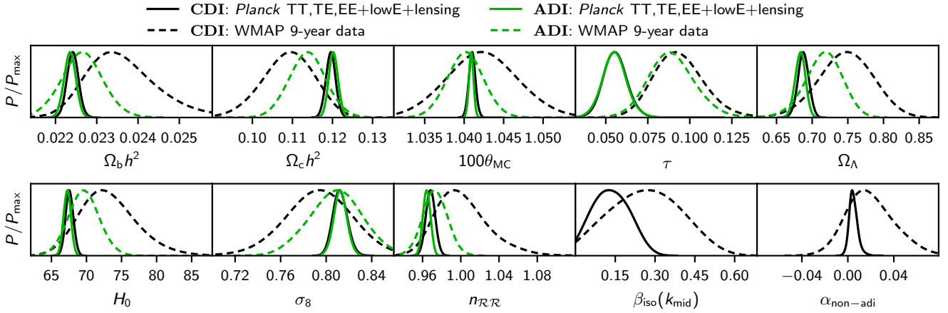
Fig. 40. Comparison of posterior probability density for selected cosmological parameters with Planck data and pre- Planck (i.e., WMAP 9-year) data. Black lines indicate the results obtained for the generally correlated mixed CDI+ADI model, and green lines for the pure adiabatic model.
