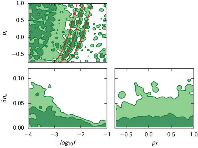
Fig. 30. Joint 68% and 95% CL constraints on the axion monodromy parameters using Planck (unbinned) TT,TE,EE+lowE+BK14, for the case of p = 4/3 . All smoothing has been turned down in the p_f - \log_{10}(f/M_{\text{Pl}}) posterior to avoid smoothing the features highlighted in red.
