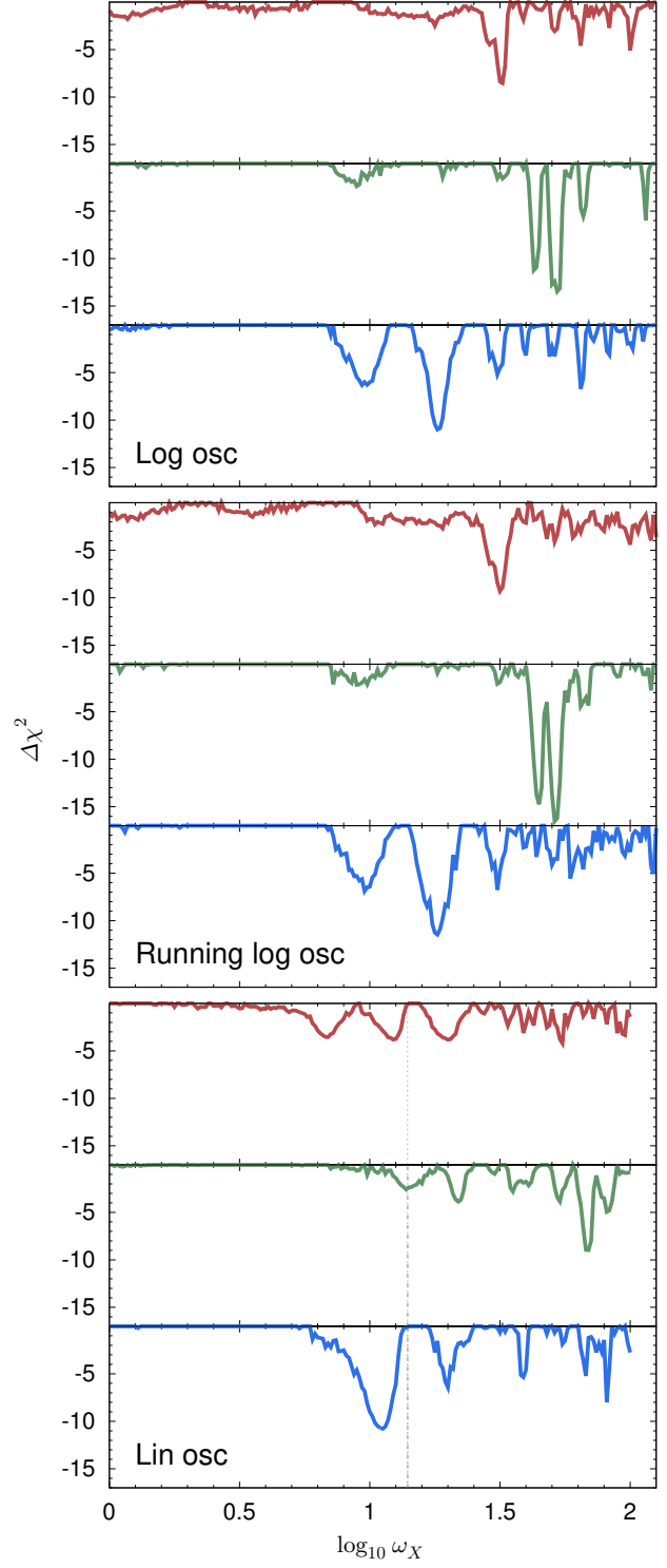
Fig. 29. Profile likelihood of the frequency parameter in the three oscillatory feature models for TT (red curves), EE (green), and TT,TE,EE data (blue). The dotted grey line in the bottom panels marks the frequency for which the linear oscillation model leads to a modulation of the angular power spectra whose wavelength roughly matches that of the CMB's acoustic oscillations. Note the lack of alignment between the temperature and polarization likelihood peaks in the vicinity of this frequency.
