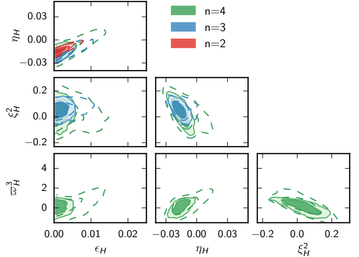
Fig. 13. Taylor expansion of H(\phi) at order n = 2, 3 , and 4 in the observable region, making no assumption about the end of inflation. The parameters are combinations of Taylor coefficients with flat priors. Dashed contours are Planck TT,TE,EE+lowE, while solid contours are Planck TT,TE,EE+lowE+BAO+BK14. The scales are the same as in PCI15 .
