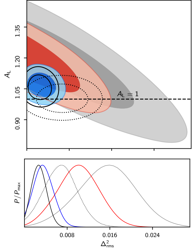
Fig. 45. Degeneracy between A_L and \Delta_{\text{rms}}^2 in the \Lambda CDM+ A_L +CIP model (top panel) and constraints on \Delta_{\text{rms}}^2 in the \Lambda CDM+CIP model, where A_L = 1 (bottom panel).
