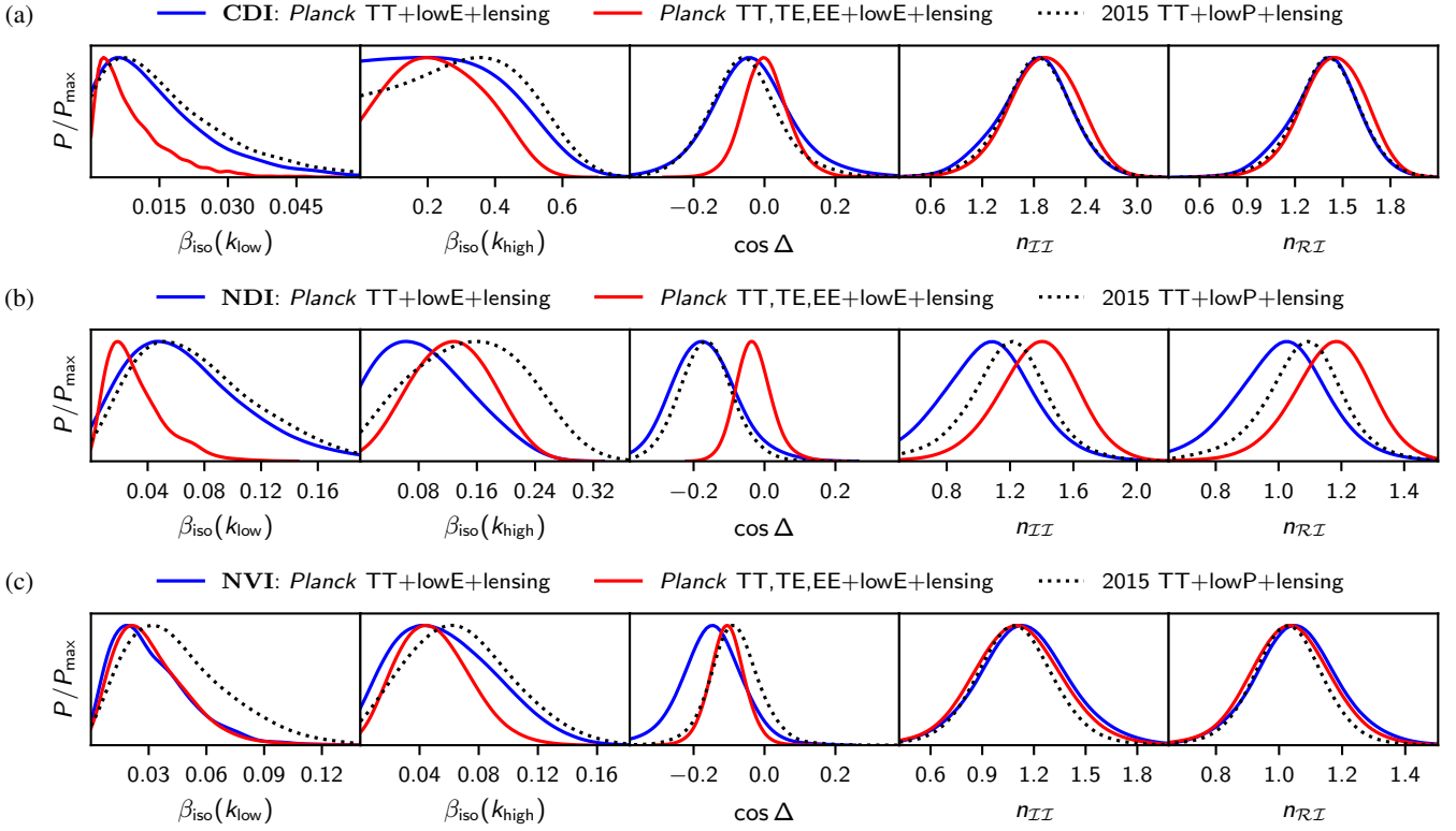
Fig. 37. Constraints on the primordial isocurvature fraction, \beta_{\text{iso}} , at k_{\text{low}} = 0.002 \text{ Mpc}^{-1} and k_{\text{high}} = 0.100 \text{ Mpc}^{-1} ; the primordial correlation fraction, \cos \Delta ; the isocurvature spectral index, n_{II} ; and the correlation spectral index, n_{RI} = (n_{RR} + n_{II})/2 , for the generally correlated mixed ADI+CDI model (a), for the ADI+NDI model (b), and for the ADI+NVI model (c). All these parameters are derived, and the distributions shown here result from a uniform prior on the primary parameters shown in Fig. 36. However, the effect of the non-flat derived-parameter priors is negligible for all parameters except for n_{II} (and n_{RI} ) where the prior biases the distribution toward unity. Note that these spectral indices are not well constrained, since we do not have a detection of non-zero isocurvature or correlation amplitude. With a sufficiently small isocurvature or correlation amplitude, an arbitrarily small or large spectral index leads to a very good fit to the data, since the model is then practically adiabatic over the range covered by the Planck data.
