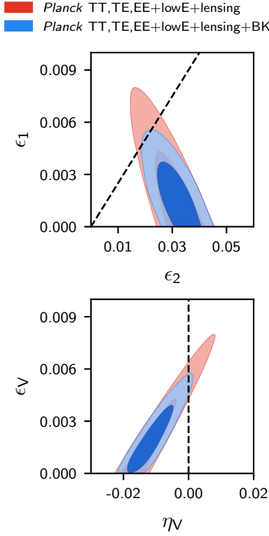
Fig. 6. Marginalized joint two-dimensional 68 % and 95 % CL regions for (\epsilon_1, \epsilon_2) (top panel) and (\epsilon_V, \eta_V) (bottom panel) for Planck TT,TE,EE+lowE+lensing (red contours), compared with Planck TT,TE,EE+lowE+lensing+BK14 (blue contours). The dashed lines divide between convex and concave potentials.
