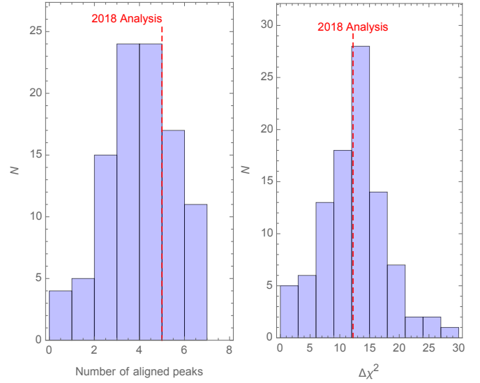
Fig. 35. Left: Number of aligned peaks in the power spectrum and the bispectrum for the linear feature model. Right: Mean improvement of those same peaks in 100 simulated bispectra combined with the unbinned high- \ell likelihood.
