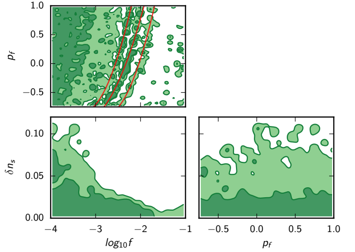
Fig. 31. Same as Fig. 30, but for the case of p = 1 .
