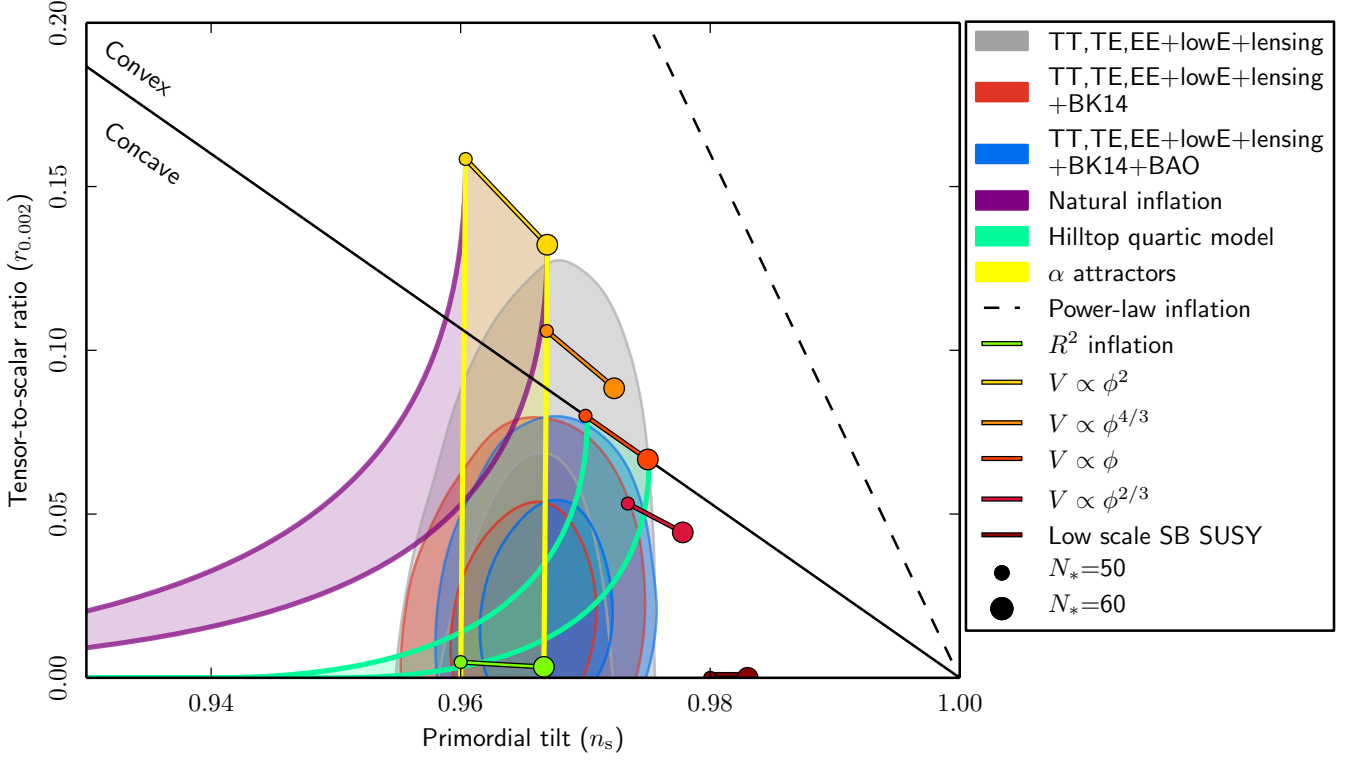
Fig. 8. Marginalized joint 68 % and 95 % CL regions for n_s and r at k = 0.002 \text{ Mpc}^{-1} from Planck alone and in combination with BK14 or BK14 plus BAO data, compared to the theoretical predictions of selected inflationary models. Note that the marginalized joint 68 % and 95 % CL regions assume dn_s/d \ln k = 0 .
