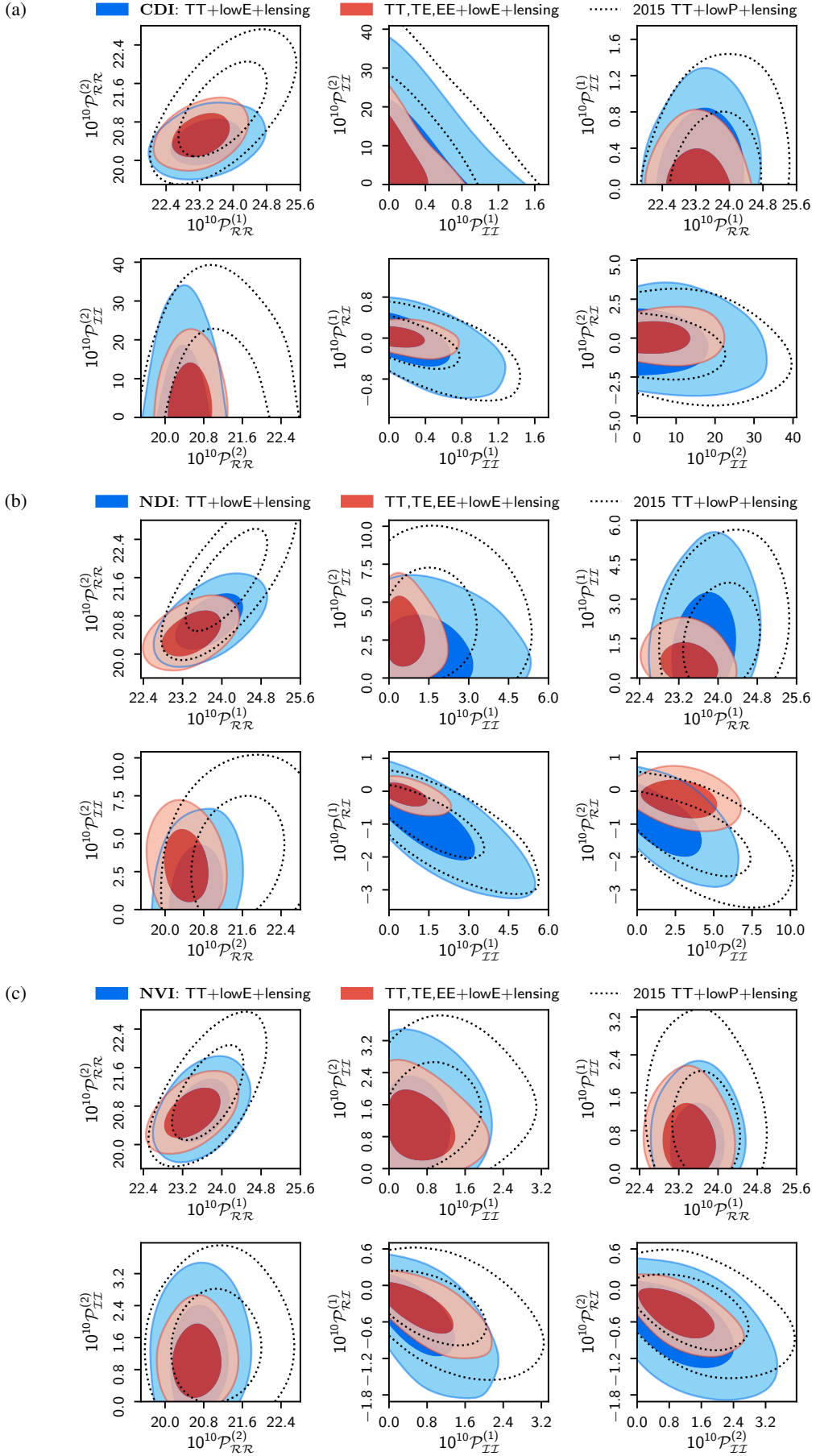
Fig. 36. Constraints on the primordial perturbation power in generally correlated ADI+CDI (a), ADI+NDI (b), and ADI+NVI (c) models at two scales, k_1 = 0.002 \text{ Mpc}^{-1} (1) and k_2 = 0.100 \text{ Mpc}^{-1} (2). Note that in our modelling \mathcal{P}_{\mathcal{R}\mathcal{I}}^{(2)} is not an independent parameter.
