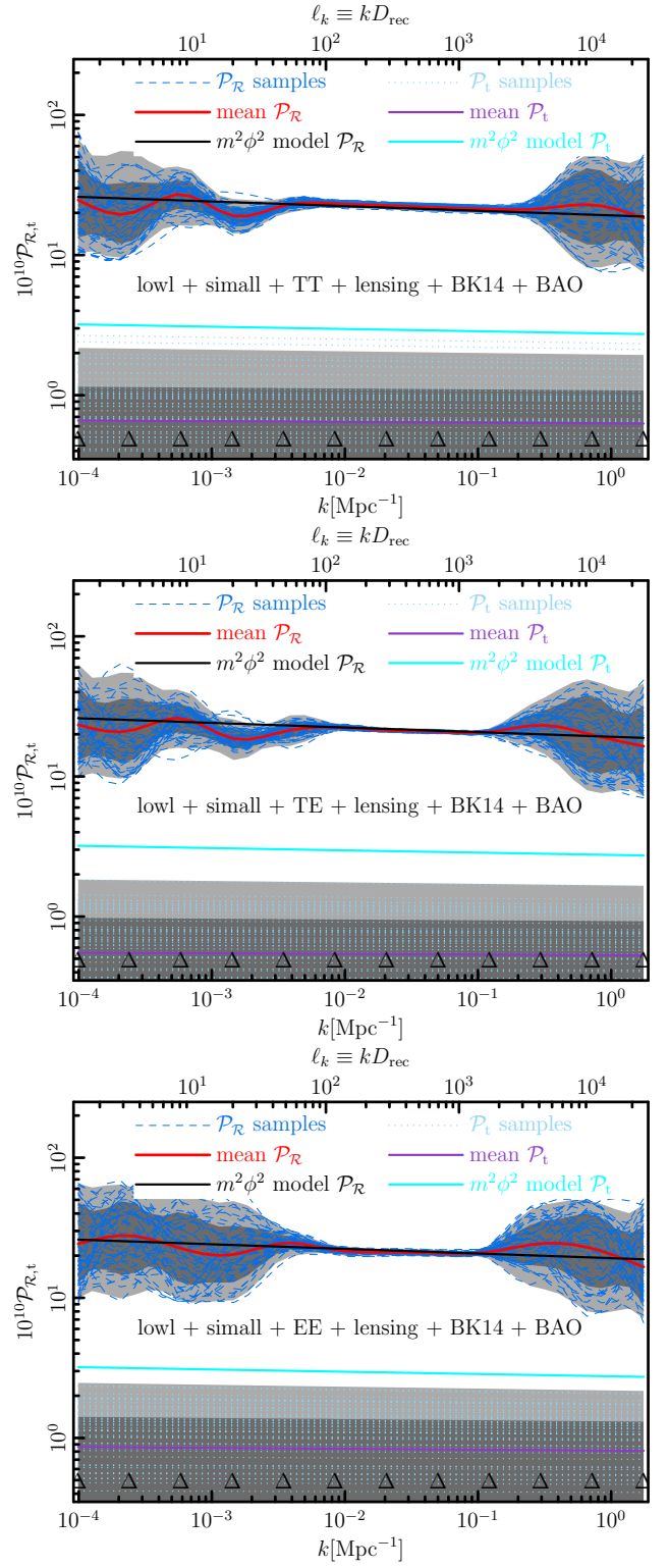
Fig. 25. Reconstructed 12-knot power spectra. The robustness of the reconstruction is apparent when sub-selections of the Planck data are used: Planck TT+lowE+lensing+BK14 (top); Planck TE+lowE+lensing+BK14 (middle); and Planck EE+lowE+lensing+BK14 (bottom).
