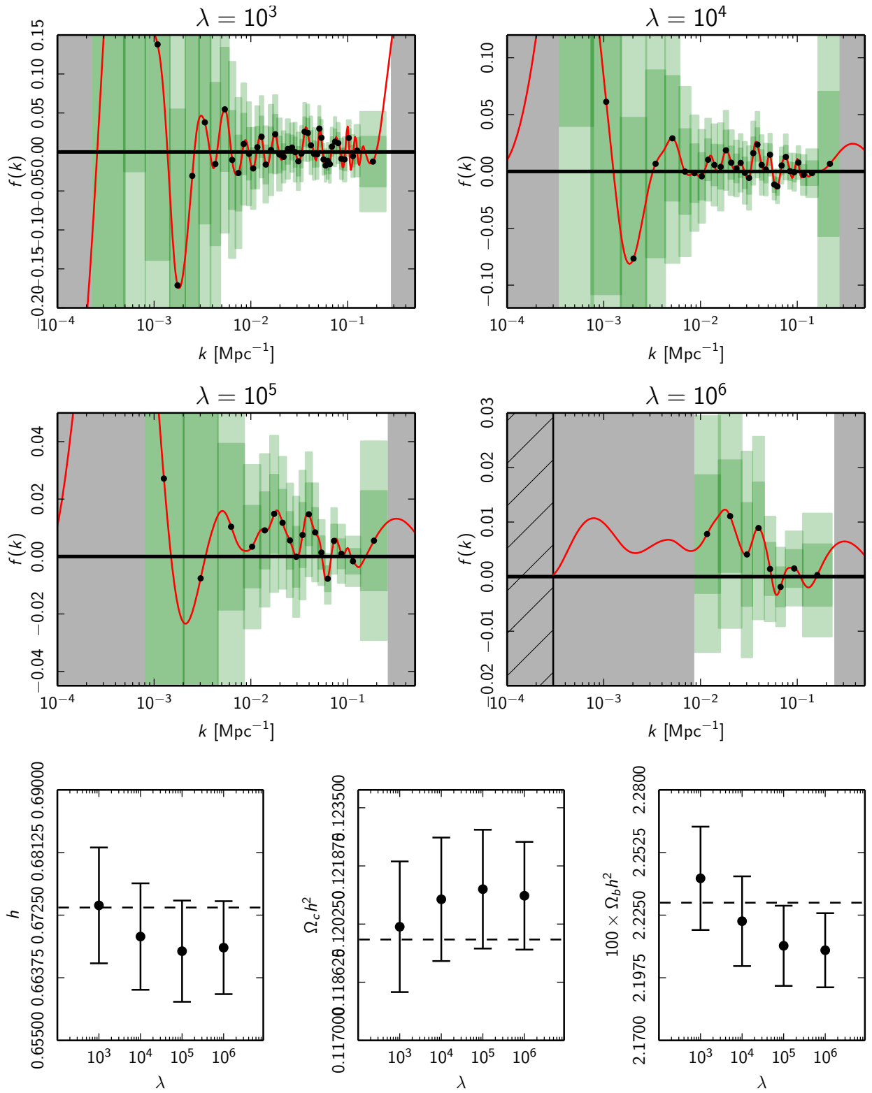
Fig. 19. Planck TT,TE,EE+lowE penalized likelihood reconstruction.
