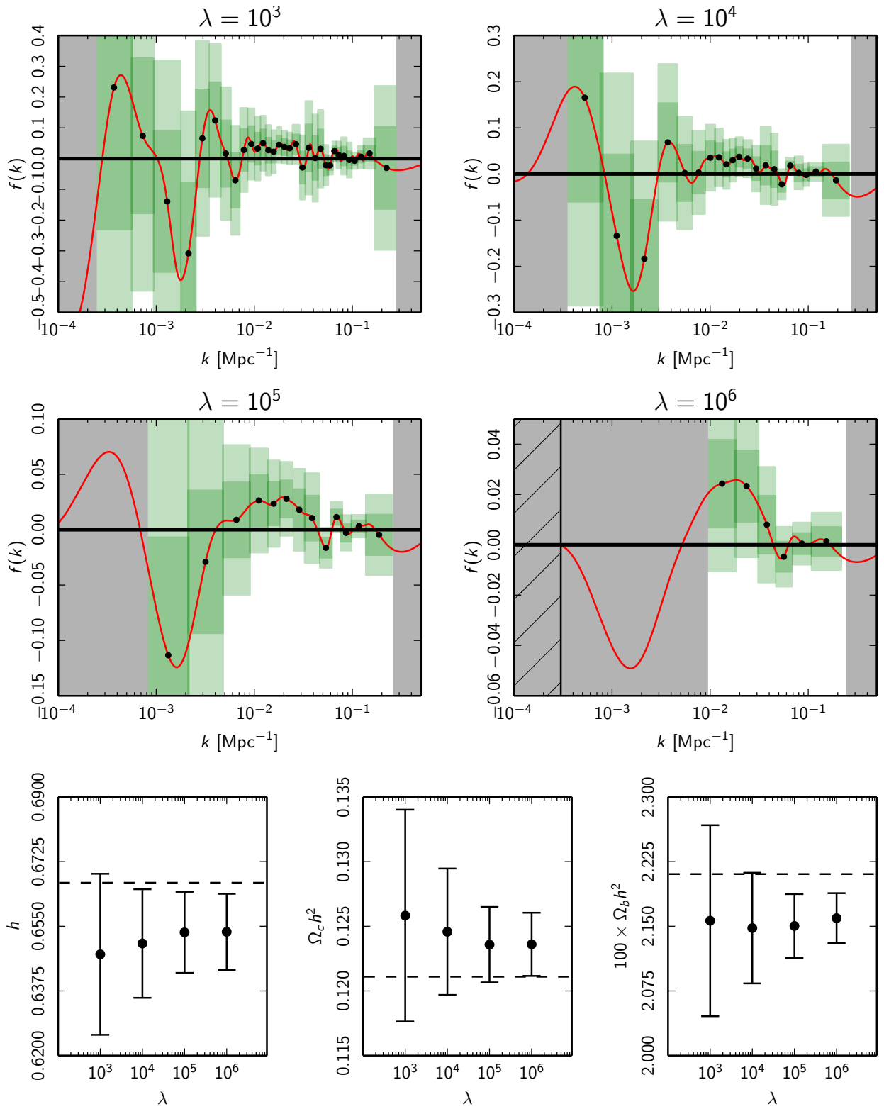
Fig. 18. Planck TT+lowE penalized likelihood reconstruction.
