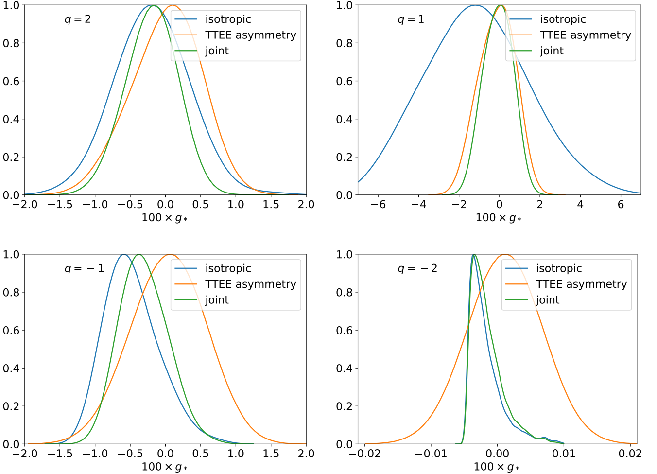
Fig. 48. Marginalized posteriors for quadrupolar modulation parameter g_* , using SMICA data for the TT+EE asymmetry constraints (orange curves) and Planck TT, TE, EE+lowE for the isotropic constraints (blue curves), which probe the modification to the power spectrum via Eq. (114). Top: constraints for q = 2 and 1 (left and right, respectively). Bottom: constraints for q = -1 and -2 (left and right, respectively). Strongly negative g_* is suppressed for q < 0 , due to the unphysical prediction of negative power.
