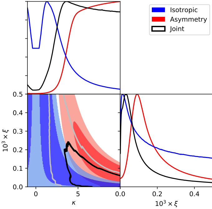
Fig. 46. Posteriors for the curvaton dipolar modulation model parameters \kappa and \xi . Contours enclose 68 % and 95 % of the posteriors. The model can explain the well-known dipolar asymmetry: note the preference for \xi > 0 in the asymmetry constraint (red contours and curves). However, the modulation preferred by the asymmetry constraint is reduced substantially when the isotropic constraint (blue) is added (black). The asymmetry constraint here uses SMICA, while the isotropic constraint uses Planck TT,TE,EE+lowE+lensing. Resolution is reduced at very small \kappa due to the sampling in \beta_{\text{iso}} .
