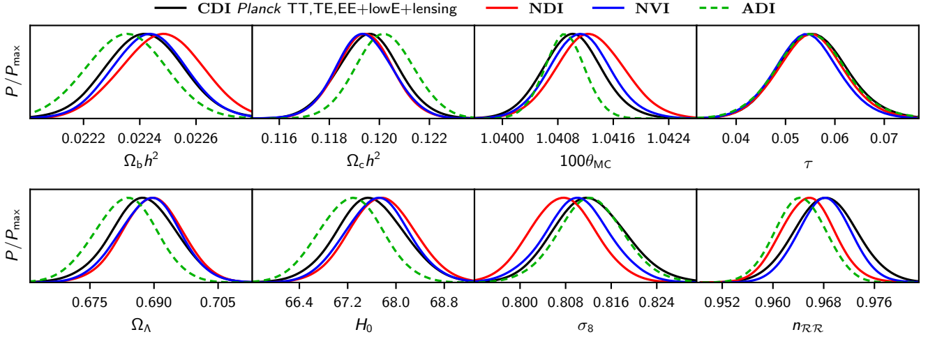
Fig. 39. Comparison of posterior probability density for the standard cosmological parameters in mixed adiabatic and isocurvature models (solid lines) to those in pure adiabatic \Lambda CDM model (ADI, dashed green lines), using Planck TT,TE,EE+lowE+lensing data.
