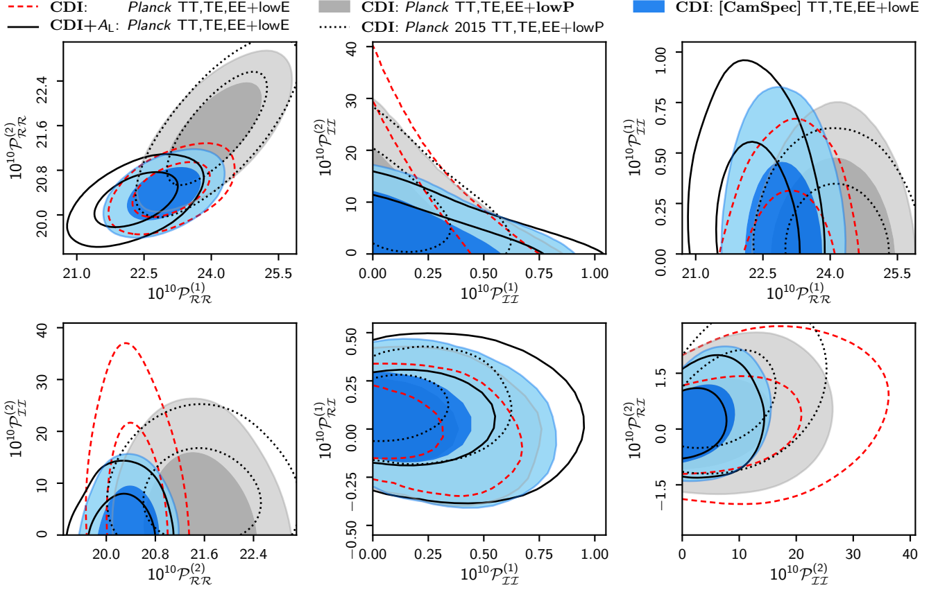
Fig. 41. Comparison of the effect of Planck 2018 likelihood choices and phenomenological lensing amplitude, A_L , on the constraints on the generally correlated mixed adiabatic and CDI model. The reference case, indicated by the red dashed curves, is for the 2018 baseline Planck high- \ell likelihood supplemented by the low- \ell Commander TT likelihood and the low- \ell SimAll EE likelihood. This combination is the same as in Fig. 37a (red curves), except now without the lensing likelihood, which to some extent hides the differences between other likelihoods and the effect of A_L . Black solid contours show the results using the same likelihood as in the reference case, but now for the mixed adiabatic and CDI model when simultaneously allowing A_L to vary. The remaining two curves are for the mixed adiabatic and CDI model (with A_L = 1 ), but now changing the low- \ell likelihood from Commander TT+ SimAll EE to LFI 70 GHz T,E,B (grey), or high- \ell likelihood from Planck to CamSpec (blue).
