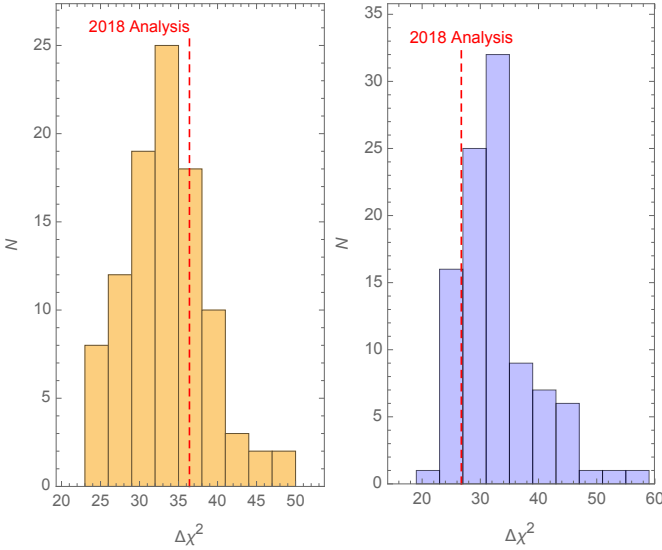
Fig. 33. Typical best-fit improvement in units of \Delta\chi^2 in 100 simulations compared to the real data (red dashed lines) for the log feature (left) and the linear feature (right) models.
