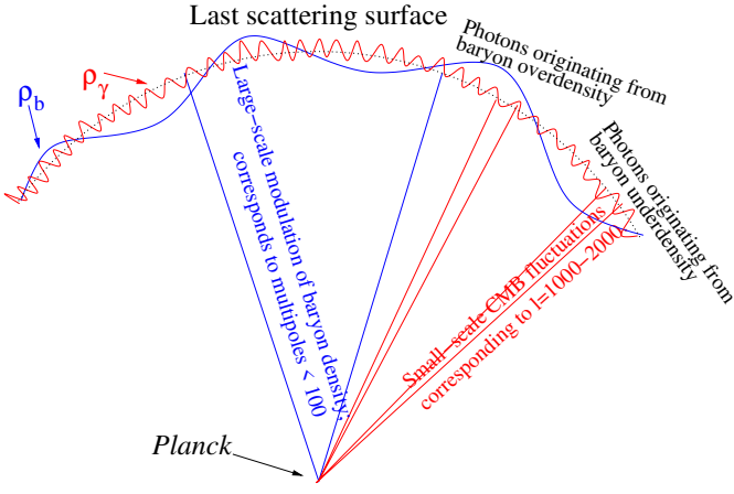
Fig. 43. Illustration of how the large-scale modulation of the baryon density by CIP gets converted into a small-scale “smoothing” effect of the temperature and polarization anisotropies.
