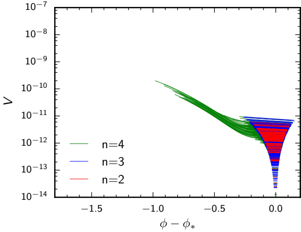
Fig. 12. Representative sample of the observable region of inflaton potentials allowed at the 95 % CL, when the potential is Taylor-expanded at order n = 2, 3 , and 4 in the observable region, making no assumption about the end of inflation, and using Planck TT,TE,EE+lowE+BAO+BK14. In natural units (where \sqrt{8\pi}M_{\text{Pl}} = 1 ). We use the same scales as in PCI15 . Note that there is another branch of solutions that is symmetric under (\phi - \phi_*) \rightarrow -(\phi - \phi_*) .
