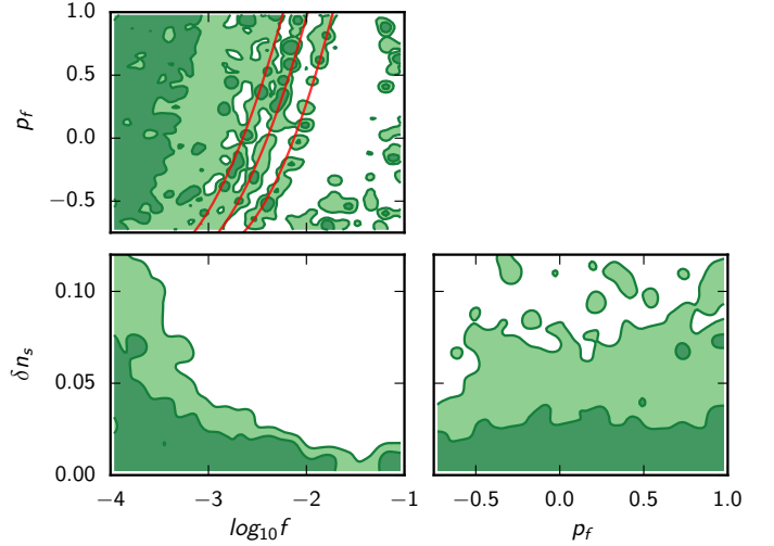
Fig. 32. Same as Fig. 30, but for the case of p = 2/3 .
