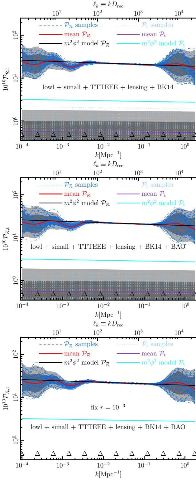
Fig. 24. Reconstructed primordial scalar power spectrum derived using Planck TT,TE,EE+lowE+lensing+BK14 data and 12 knots for the cubic spline interpolation (with positions marked as \Delta at the bottom of each panel). Mean (ensemble-averaged) spectra are heavy lines, allowed \pm 1\sigma and \pm 2\sigma regions for trajectories are the shaded regions, and the dashed lines denote selected trajectories with parameters sampled within the \pm 1\sigma posterior. Below the scalar power is the tensor power reconstruction. The addition of the BAO likelihood shown in the middle panel makes almost no visual difference to the reconstructions. In the bottom panel, fixing the tensor-to-scalar ratio to r = 0.001 also shows only small differences in reconstruction. Knot positions in k roughly translate to multipoles through kD_{\text{rec}} , where D_{\text{rec}} is the comoving distance to recombination.
