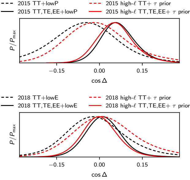
Fig. 42. Scale-independent primordial correlation fraction in the mixed adiabatic and CDI model. The black curves are with Planck high- \ell and low- \ell data, while the red ones result from using only the high- \ell Plik likelihood supplemented with a Gaussian prior on the optical depth. For the 2015 data (top panel) this prior was \tau = 0.078 \pm 0.019 , whereas for the 2018 case (bottom panel) we have adopted \tau = 0.055 \pm 0.007 from the Planck 2018 TT,TE,EE+lowE+lensing CDI chain.
