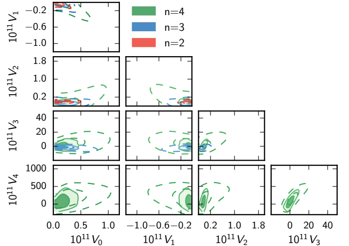
Fig. 11. Taylor expansion of V(\phi) at order n = 2, 3 , and 4 in the observable region, making no assumption about the end of inflation. In natural units (where \sqrt{8\pi}\mathcal{M}_{\text{Pl}} = 1 ). The parameters are the Taylor coefficients, obtained here as derived parameters with non-flat priors. Dashed contours are Planck TT,TE,EE+lowE, while solid contours are Planck TT,TE,EE+lowE+BAO+BK14. The scales are the same as in PCI15.
