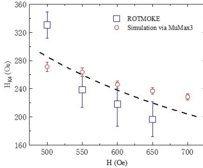
Fig. 4: H_{K_4} from ROTMOKE experiment and MuMax3 simulation above 500 Oe. Dashed line represents
