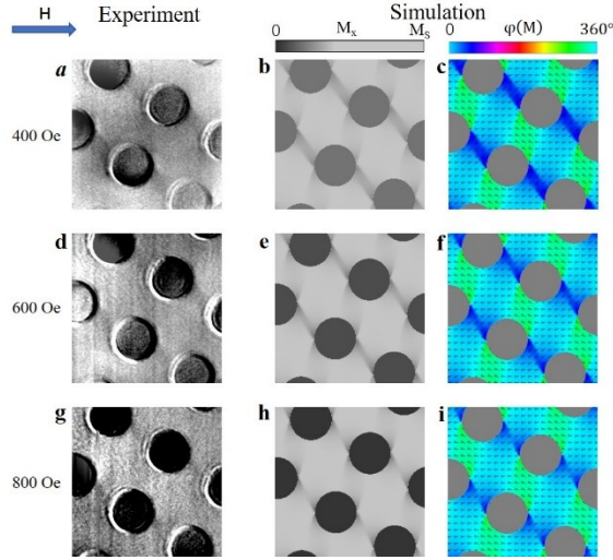
Fig. 5: Experimental images from MTXM and simulated images from MuMax3. a, d, g : Experimental MTXM images with in-plane magnetic field of 400, 600 and 800 Oe, respectively, along the direction as shown on the top left. b, e, h : Simulated MTXM images with the x-component of magnetization ( M_x ) represented by the greyscale colormap shown on top. c, f, i : Colored images showing the magnetization direction in space. The colormap on top shows the magnetization angle \varphi(M) relative to the field direction.
