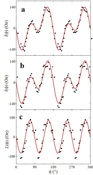
Fig. 3: ROTMOKE result. Magnetic torque l(\varphi) at H = 600 Oe with the optical plane parallel to a , [10] axis, and b , [01] axis of the sample, respectively. In experiment, (a) and (b) were achieved by fixing the optical plane in space but rotating sample by 90^\circ around the surface normal direction. The identical result of a and b shows that the uniaxial anisotropy is an artifact. c , Redefined torque L(\varphi) using eqn. (3) to eliminate the artifact of the uniaxial anisotropy. Red lines are fitting curves using eqn. (2).
