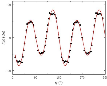
Fig. 6: An example of simulated torque l(\varphi) via MuMax3 at H = 600 Oe.
