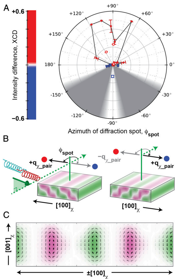
Fig. 3. Rotational symmetry of chiral polar arrays observed in azimuthal pattern of XCD. (A) XCD intensity plotted versus azimuth, \phi_{\text{spot}} , for each diffraction spot from the polar arrays. Red circles indicate XCD > 0; blue squares indicate XCD < 0. Filled markers were measured at n_{\text{SL}} = 4 ; hollow markers were measured at n_{\text{SL}} = 3 . Gray regions show experimentally inaccessible sample geometries. (B) Diffraction patterns for two sample orientations (separated by 180° azimuthally) exhibit similar XCD (red and blue circles) relative to the scattering geometry: \Phi = 0^\circ (Left) and 180^\circ (Right). Curved arrows indicate \phi_{\text{spot}} measured from the in-plane projection (dashed green arrow) of the incoming X-rays. Sample is depicted with counter-rotated polarization cores (small black arrows) and alternating axial polarization (green and magenta) domains. (C) Polarization structure is averaged over both orientations in the (010)_{\chi} cross-section. These polar cores possess a chiral texture that is robust versus a twofold rotation. Error bars in A represent uncertainty in fitting the XCD spectra at each azimuth ( Azimuthal XCD Measurements ).
