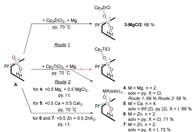
Scheme 2 Reductive metalation of A using Cp 2 ZrCl 2 /Mg ( 3 ·MgCl 2 ) as well as Mg/MgCl 2 ( 4 ), Ca/Cal 2 ( 5 ), Zn/ZnCl 2 ( 6 ) and Zn/ZnI 2 ( 7 ).
