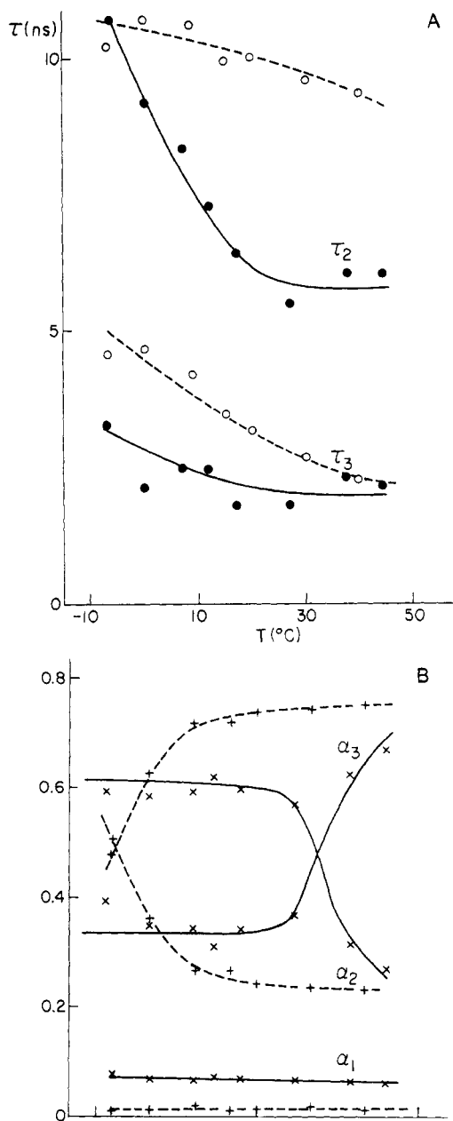
FIGURE 1: Lifetime values ( \tau ) (A) and associated preexponential factors ( \alpha ) (B) vs. temperature of cis -PnA ( \bullet and \times ) and of trans -PnA ( \circ and + ) in dodecane, as determined by a three-component analysis.
