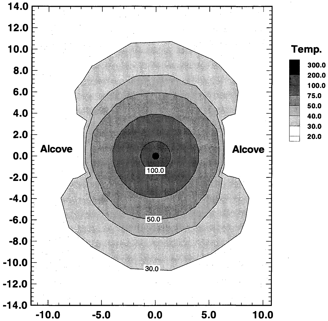
Figure 6.1-1 Temperature response for Base Case at 1 year in 2D - simulation.
