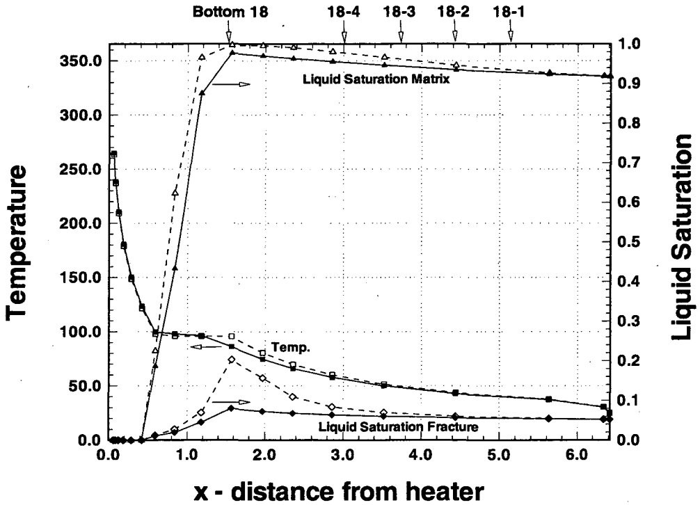
Figure 4.3-4 Comparison of temperature / liquid saturation at 1 year along X - axis at Y = 6.00 m and Z = 0.0 m for two different fracture continuum conceptualizations. Solid symbols / lines denote a homogenous domain, hollow symbols and dashed lines denote Base Case.
