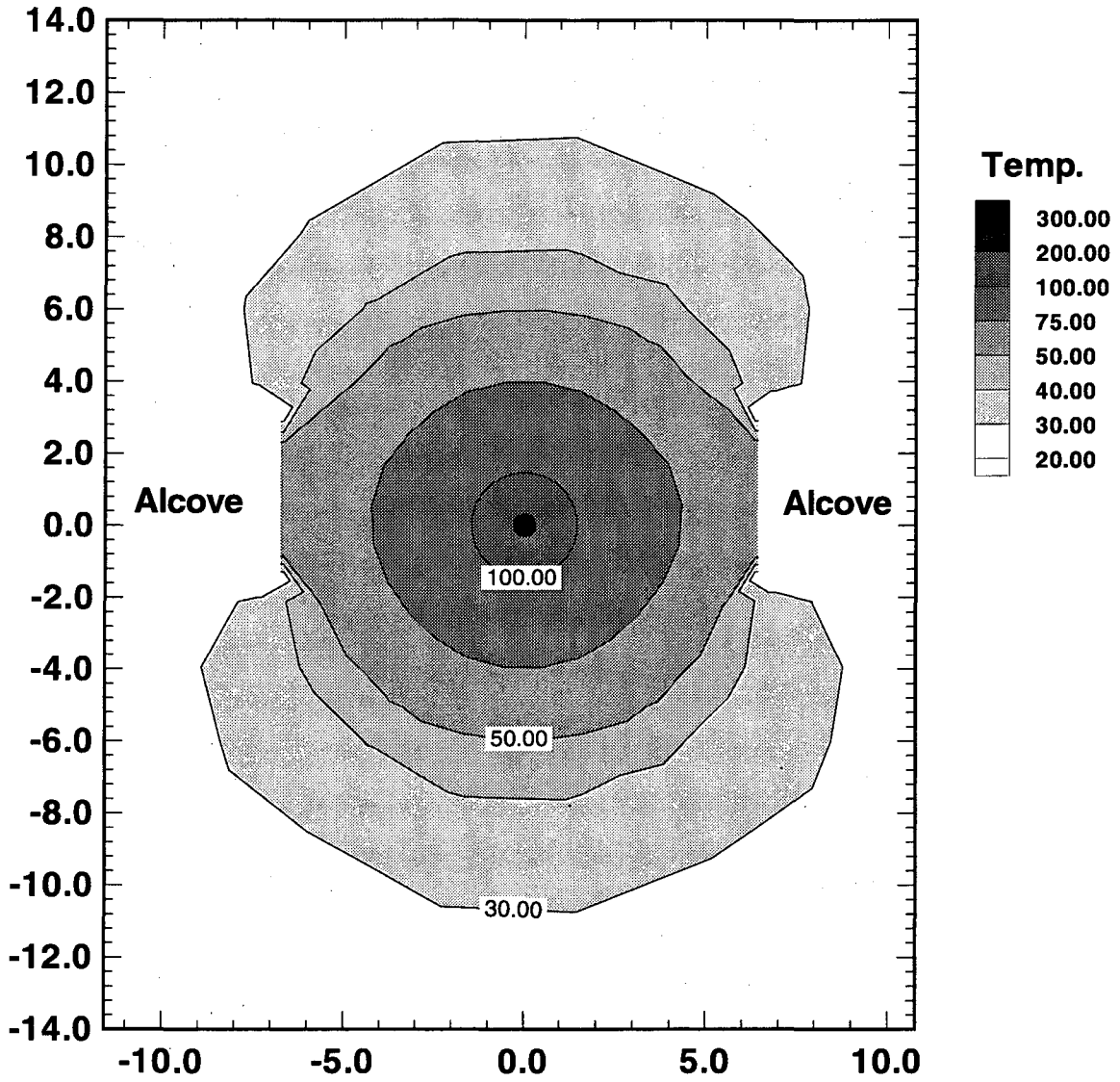
Figure 6.2-1 Temperature response for case with perfect insulation at alcove walls at 1 year in 2D - simulation.
