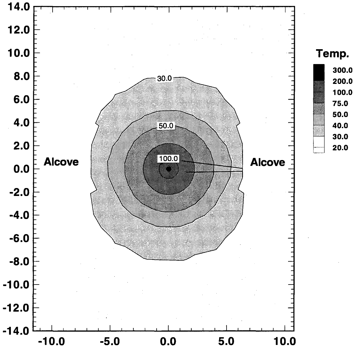
Figure 4.2-1 Temperature response for Base Case at 1 year in XZ - cross section at Y = 4.25 m.
