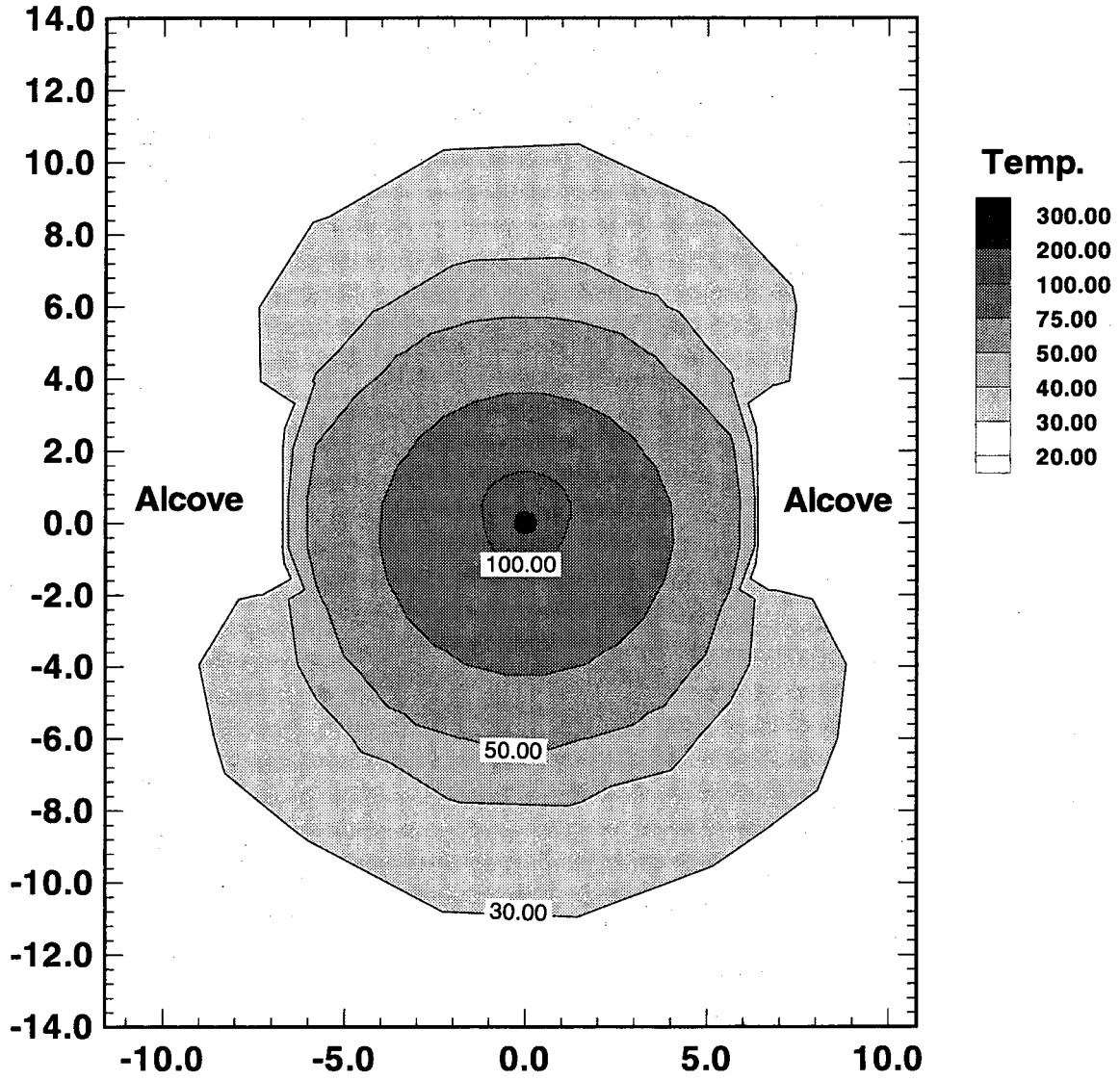
Figure 6.5-1 Temperature response for case with high fracture permeability at 1 year in 2D - simulation.
