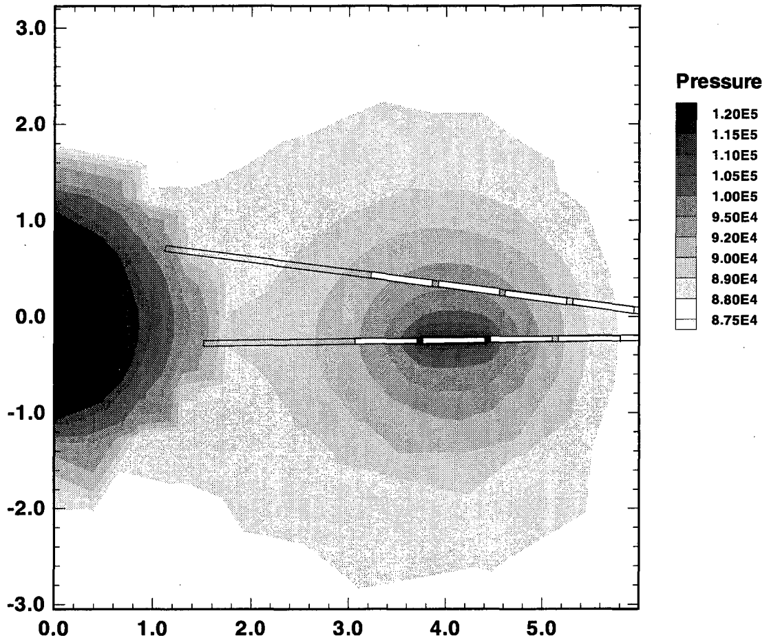
Figure 5.2-16 Steady state pressure (in Pa) for constant flow air injection in Zone 2 of Borehole 18 for injection test performed at 1 year. Results are shown in test hole plane (i.e. XZ - cross section at Y = 4.25 m).
