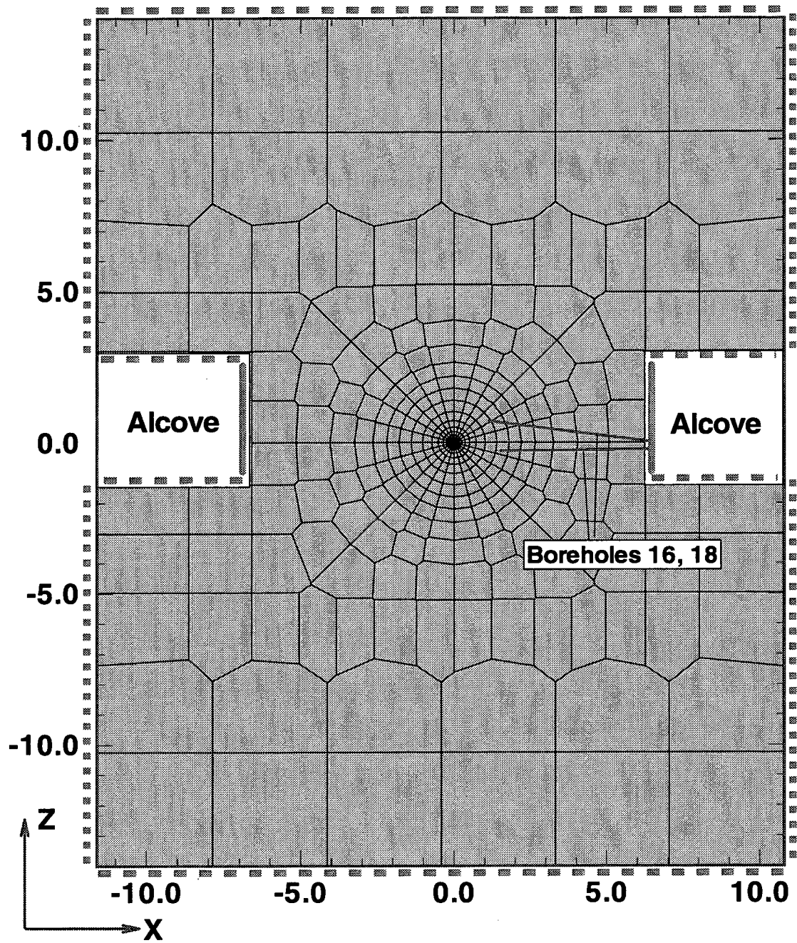
Figure 4.1-1 XZ - cross section of the discretization grid. Dashed lines indicate a constant primary variable boundary, dotted lines represent a closed boundary, and the solid lines along the vertical alcove walls represent the thermal insulation. Also indicated is the location of the air permeability test holes 16 and 18.
