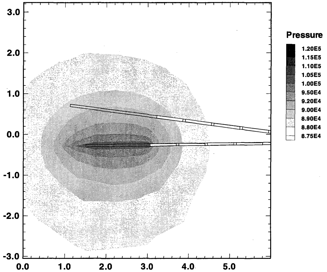
Figure 5.2-8 Steady state pressure (in Pa) for constant flow air injection in Zone 3 of Borehole 18 for injection test performed at 21 months for a 1 year heating period. Results are shown in test hole plane (i.e. XZ - cross section at Y = 4.25 m).
