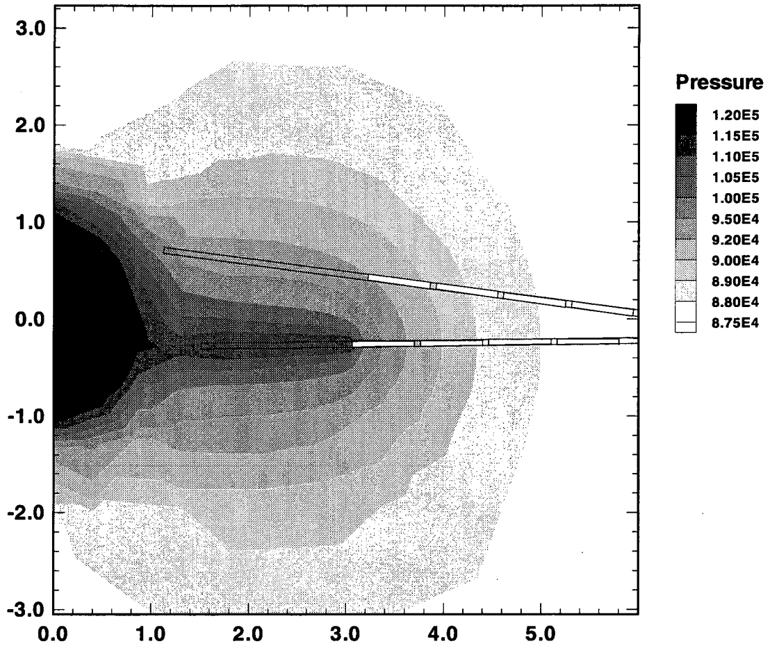
Figure 5.2-5 Steady state pressure (in Pa) for constant flow air injection in Zone 3 of Borehole 18 for injection test performed at 1 year. Results are shown in test hole plane (i.e. XZ - cross section at Y = 4.25 m).
