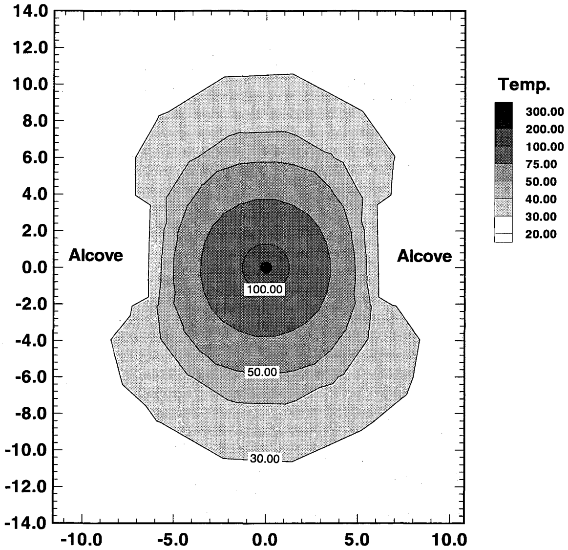
Figure 6.2-5 Temperature response for case with non-insulated alcove walls at 1 year in 2D - simulation.
