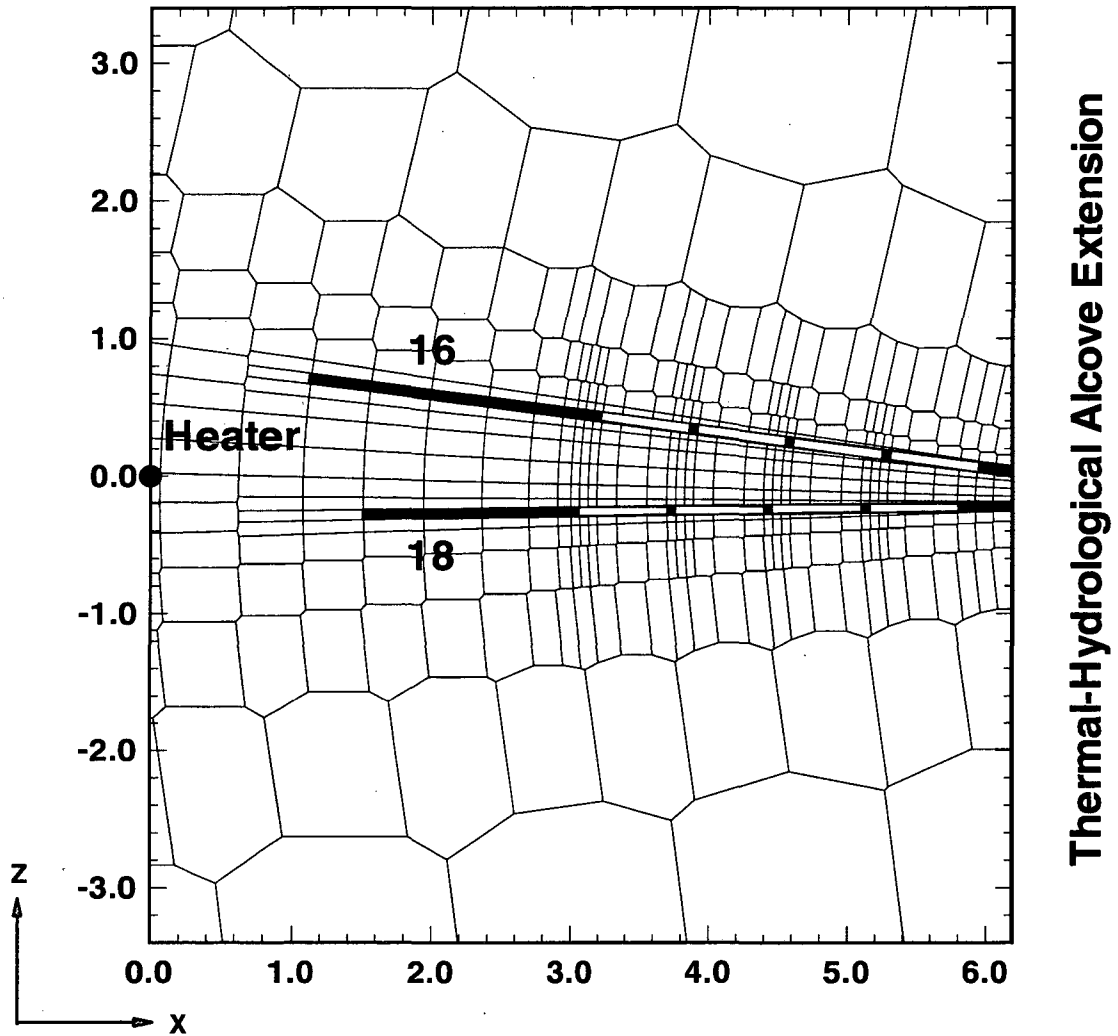
Figure 5.1-2 Details of grid design in XZ - cross section for air injection runs showing packer and sensor arrangement in Boreholes 16 and 18.
