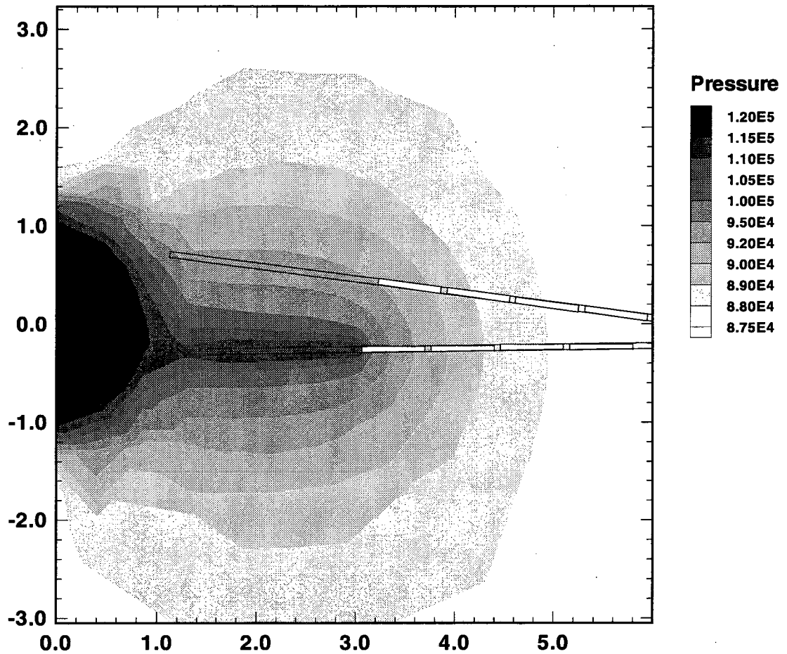
Figure 5.2-4 Steady state pressure (in Pa) for constant flow air injection in Zone 3 of Borehole 18 for injection test performed at 9 months. Results are shown in test hole plane (i.e. XZ - cross section at Y = 4.25 m).
