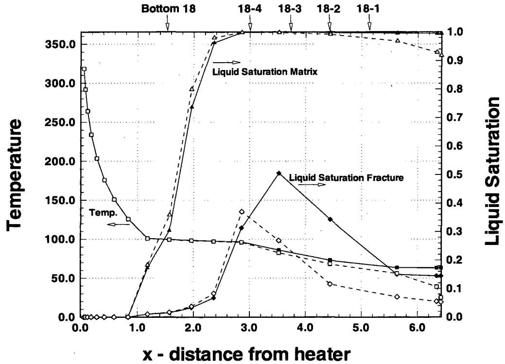
Figure 6.2-4 Comparison of temperature / liquid saturation at 1 year along X - axis at Z = 0.0 m for two different alcove boundary conditions in 2D - simulation. Solid symbols / lines denote a perfect insulation for heat, liquid and gas; hollow symbols and dashed lines denote insulation for heat only, as used in the Base Case.
