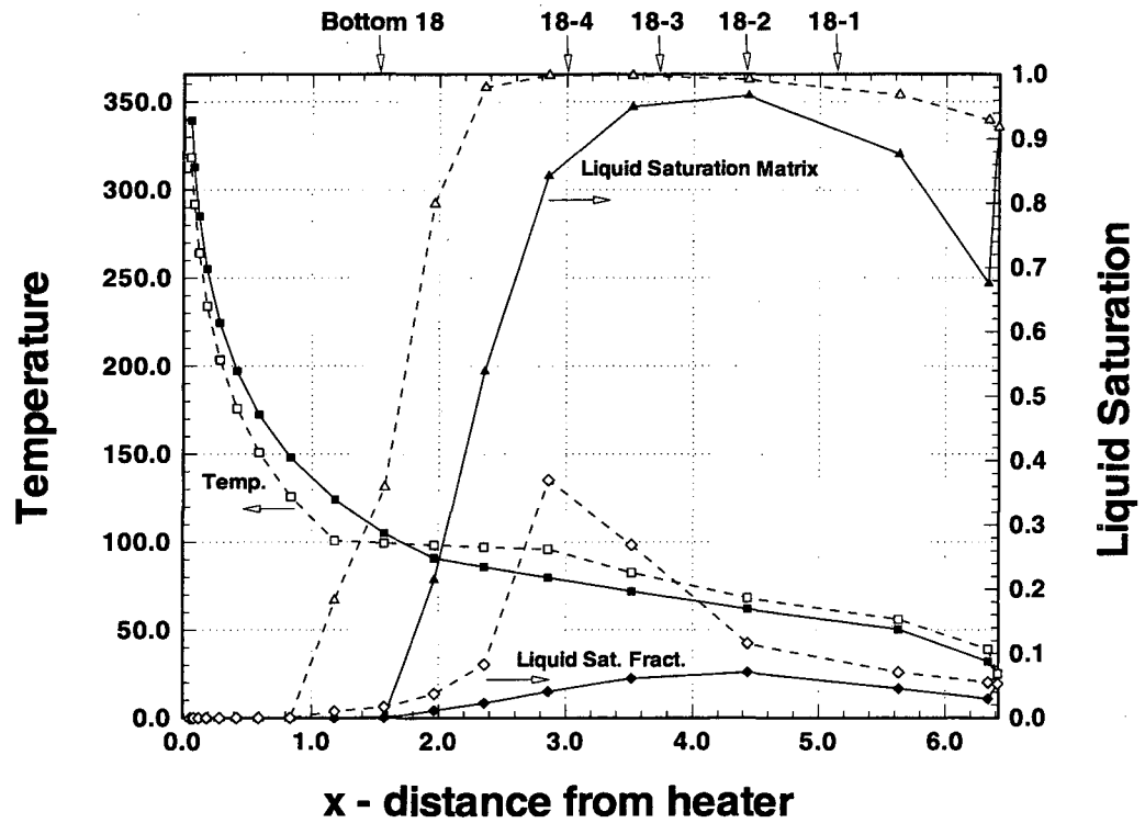
Figure 6.3-4 Comparison of temperature / liquid saturation at 1 year along X - axis at Z = 0.0 m for ordinary and enhanced vapor diffusion in 2D - simulation. Solid symbols / lines denote enhanced vapor diffusion, hollow symbols and dashed lines denote ordinary vapor diffusion, as used in the Base Case.
