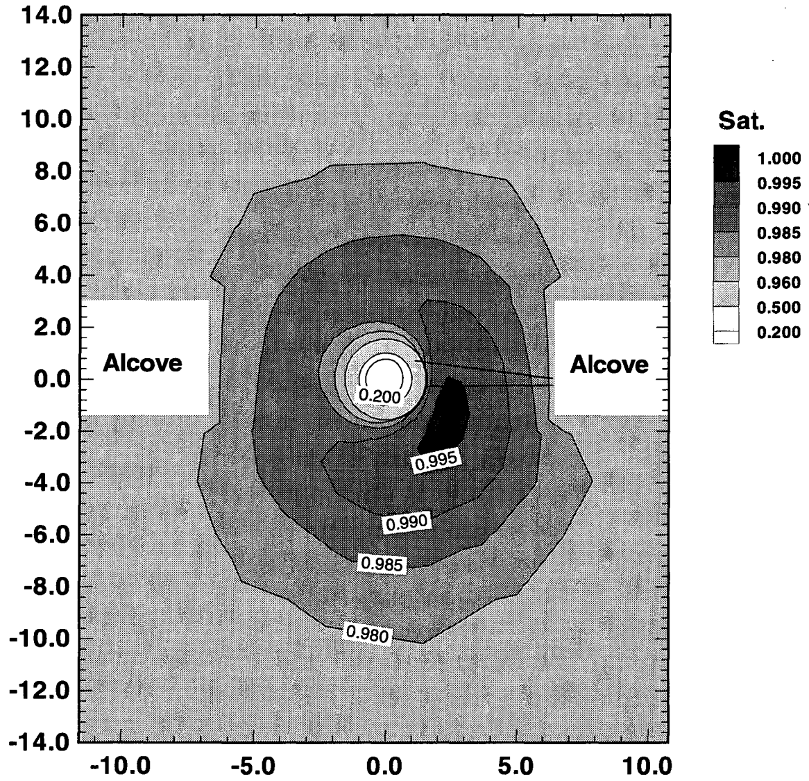
Figure 4.4-2 Equivalent continuum liquid saturation for case with high initial saturation at 1 year in XZ - cross section at Y = 4.25 m.
