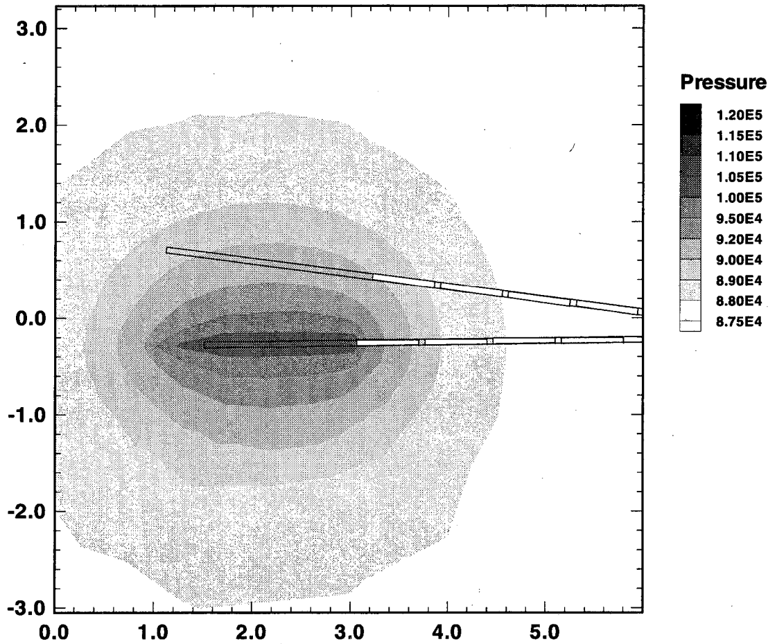
Figure 5.2-6 Steady state pressure (in Pa) for constant flow air injection in Zone 3 of Borehole 18 for injection test performed at 15 months for a 1 year heating period. Results are shown in test hole plane (i.e. XZ - cross section at Y = 4.25 m).
