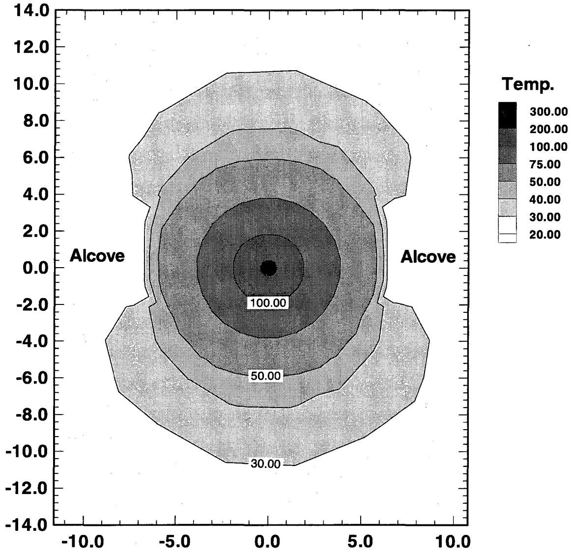
Figure 6.4-1 Temperature response in the matrix at 1 year in 2D - simulation using dual-permeability approach.
