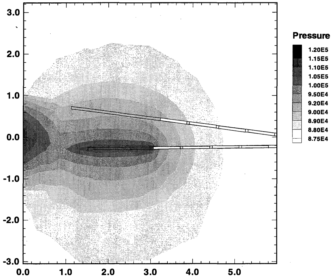
Figure 5.2-2 Steady state pressure (in Pa) for constant flow air injection in Zone 3 of Borehole 18 for injection test performed at 77 days. Results are shown in test hole plane (i.e. XZ - cross section at Y = 4.25 m).
