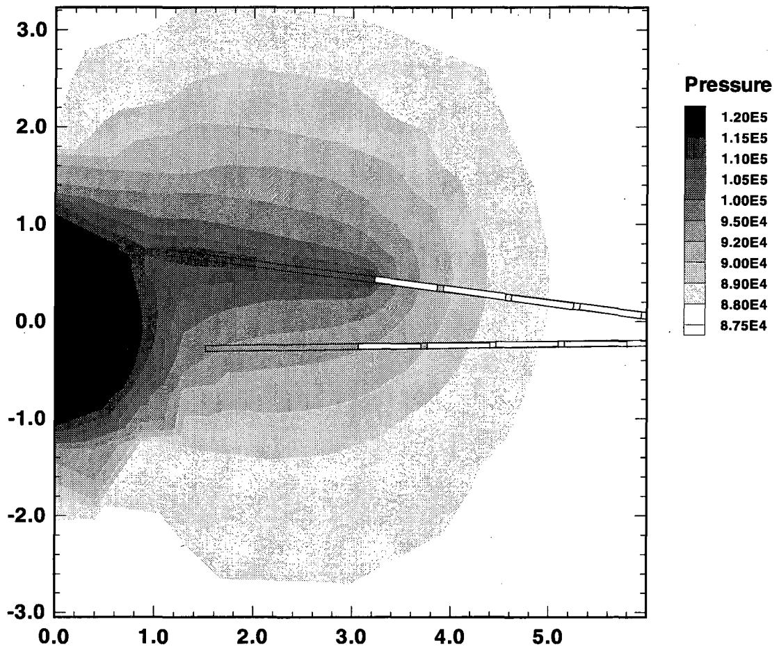
Figure 5.2-18 Steady state pressure (in Pa) for constant flow air injection in Zone 3 of Borehole 16 for injection test performed at 1 year. Results are shown in test hole plane (i.e. XZ - cross section at Y = 4.25 m).
