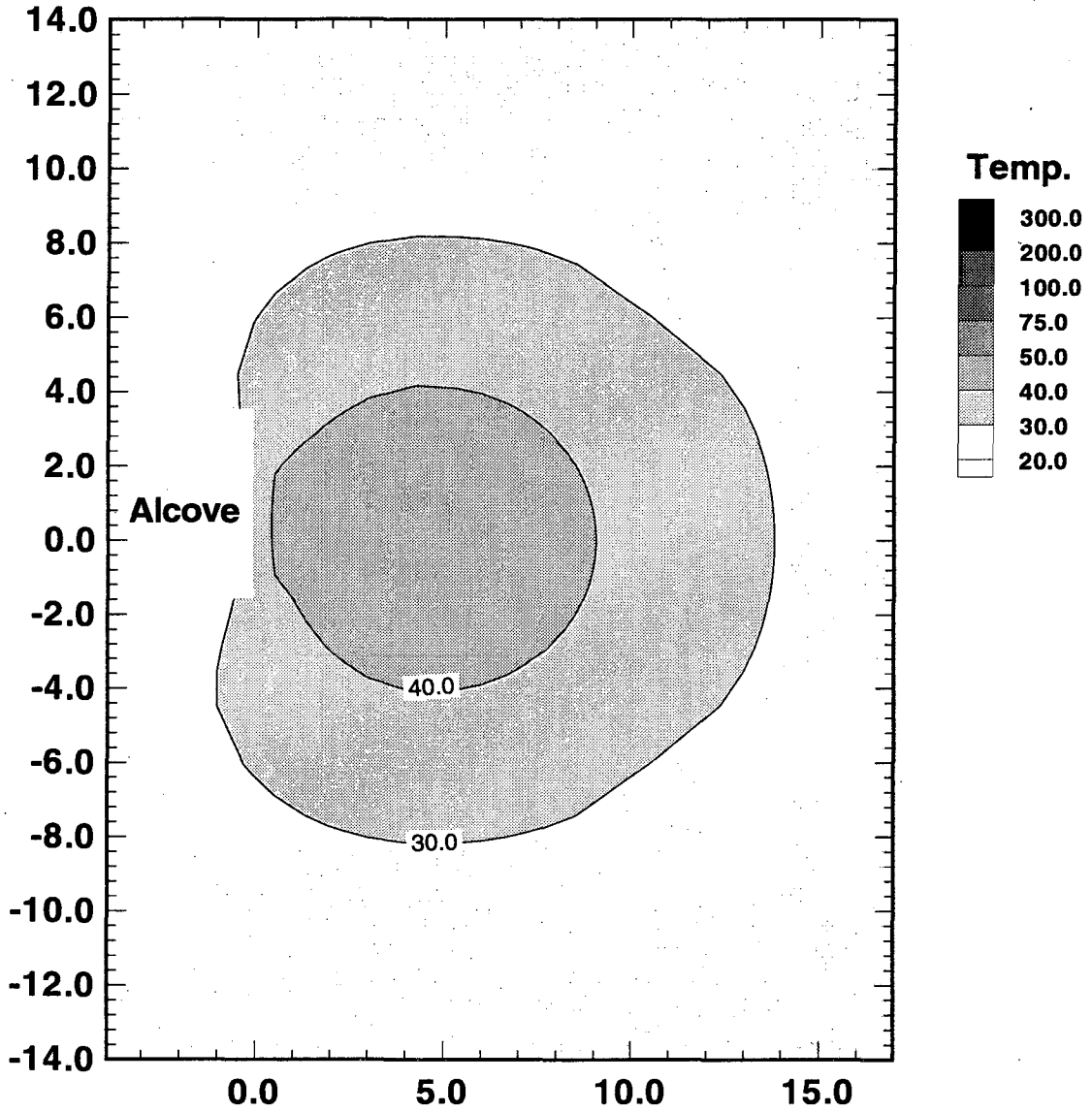
Figure 4.2-12 Temperature response for Base Case at 15 months after 1 year heating period in YZ - cross section at X = 0.00 m.
