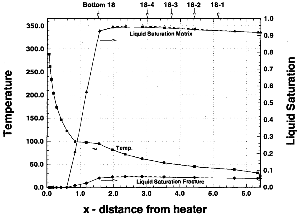
Figure 4.3-3 Comparison of temperature / liquid saturation at 1 year along X - axis at Y = 4.25 m and Z = 0.0 m for two different fracture continuum conceptualizations. Solid symbols / lines denote a homogenous domain, hollow symbols and dashed lines denote Base Case.
