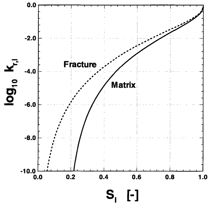
Figure 3.3-2 Liquid relative permeability function for matrix and fractures with ECM model using Base Case parameters.
