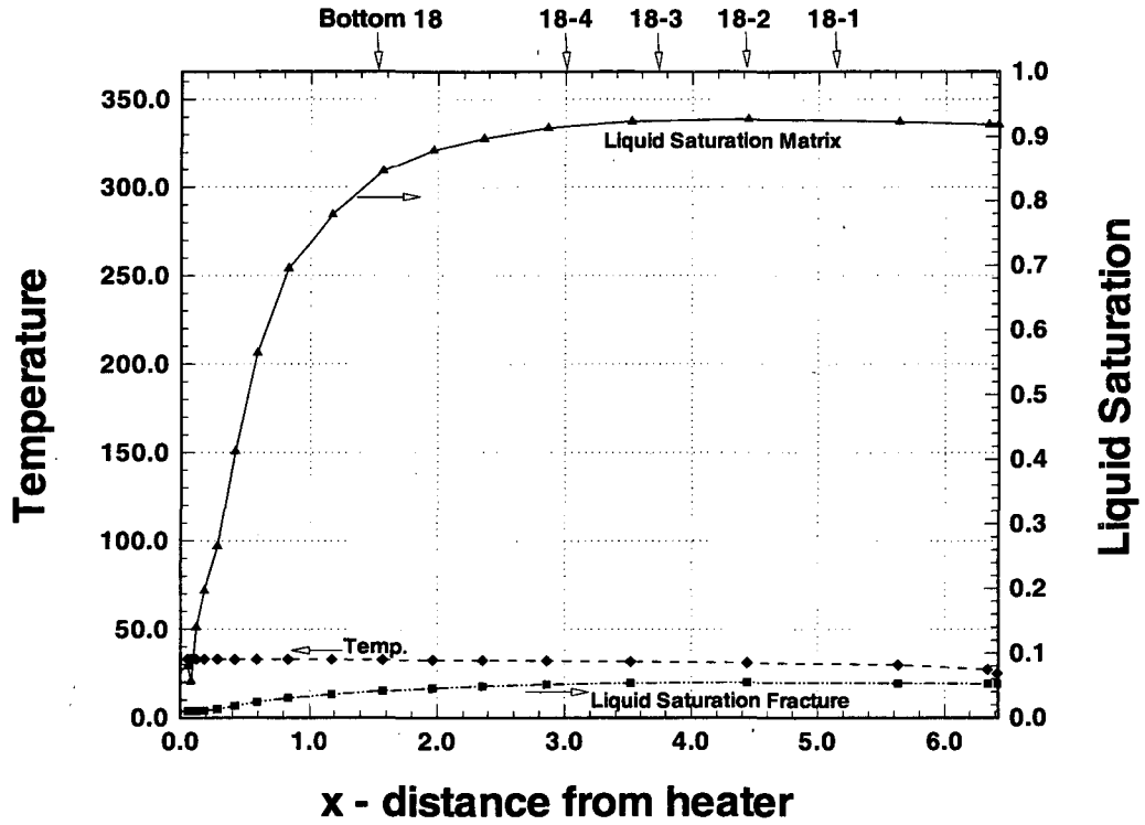
Figure 4.2-25 Temperature / liquid saturation for Base Case at 21 months after 1 year heating period along X - axis at Y = 4.25 m and Z = 0.0 m.
