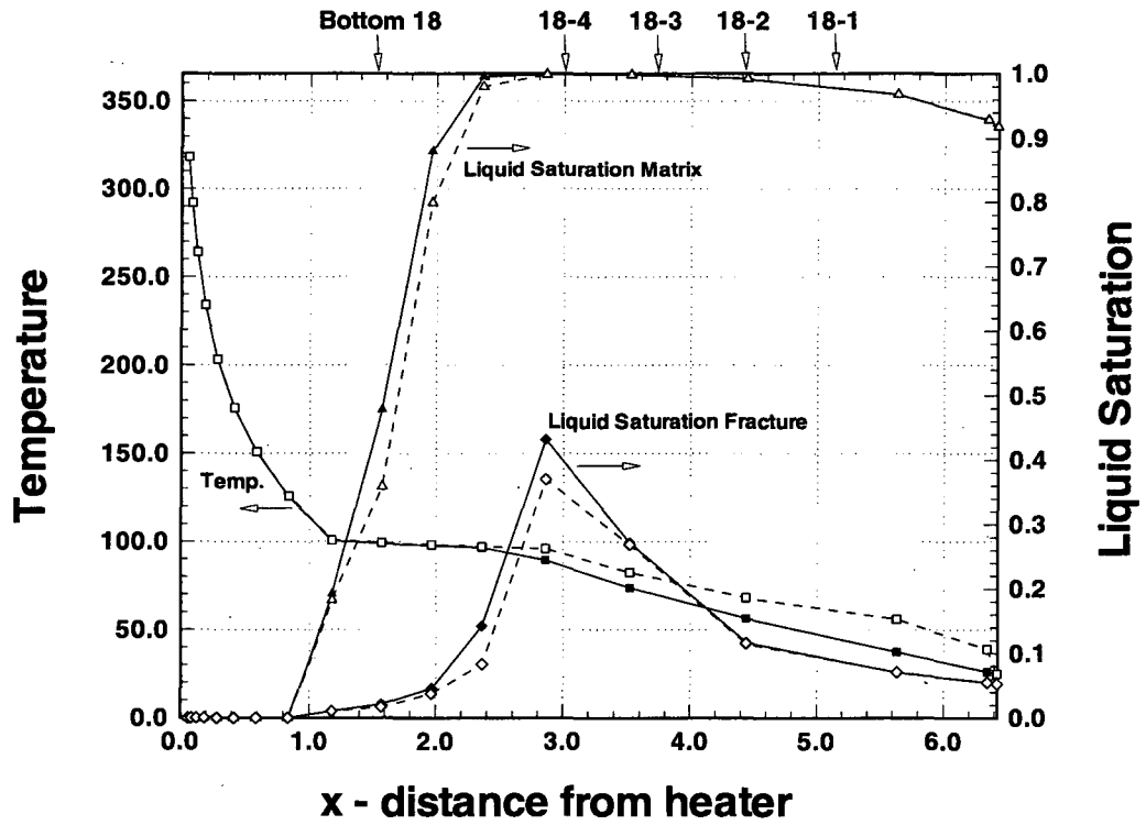
Figure 6.2-8 Comparison of temperature / liquid saturation at 1 year along X - axis at Z = 0.0 m for two different alcove boundary conditions in 2D - simulation. Solid symbols / lines denote no insulation, hollow symbols and dashed lines denote insulation for heat only, as used in the Base Case.
