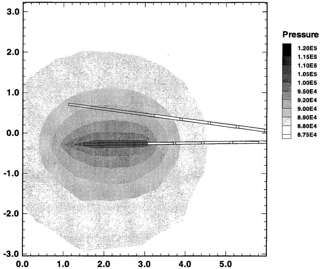
Figure 5.2-7 Steady state pressure (in Pa) for constant flow air injection in Zone 3 of Borehole 18 for injection test performed at 18 months for a 1 year heating period. Results are shown in test hole plane (i.e. XZ - cross section at Y = 4.25 m).
