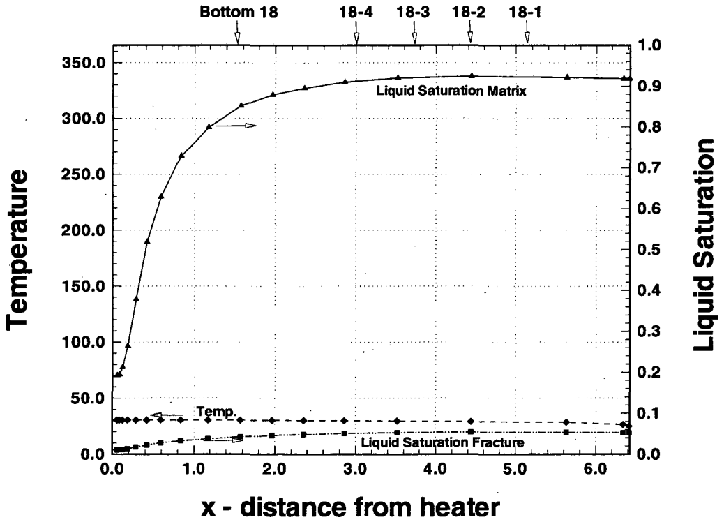
Figure 4.2-26 Temperature / liquid saturation for Base Case at 2 years after 1 year heating period along X - axis at Y = 4.25 m and Z = 0.0 m.
