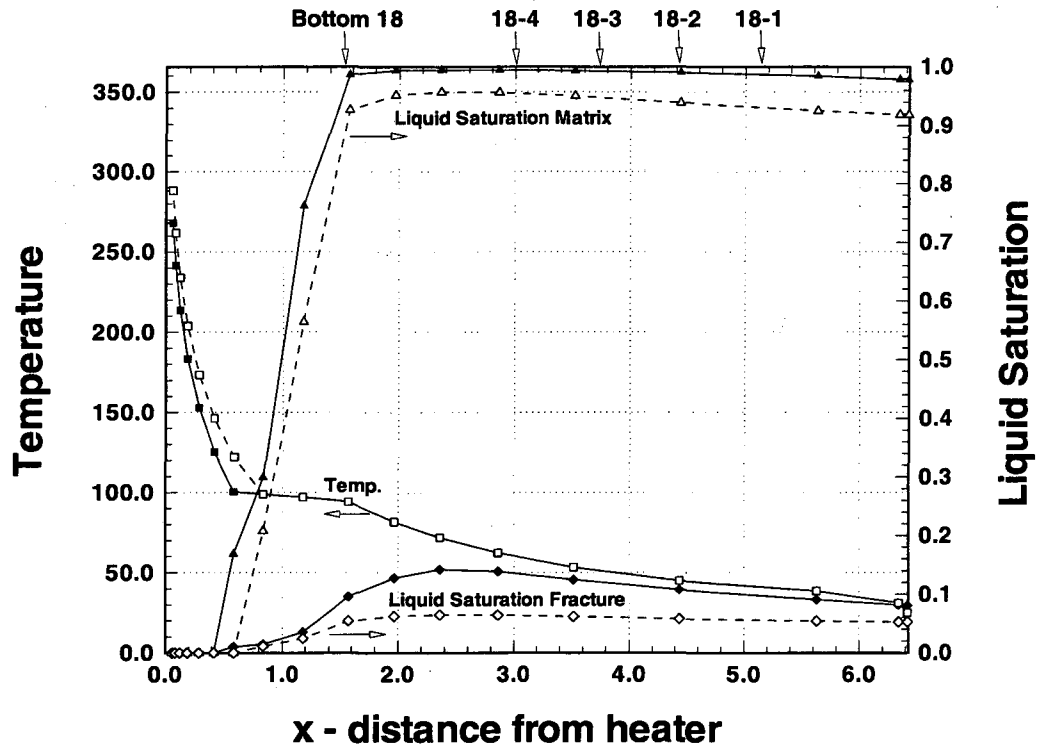
Figure 4.4-4 Comparison of temperature / liquid saturation at 1 year along X - axis at Y = 4.25 m and Z = 0.0 m for two different initial saturation values. Solid symbols / lines denote a high initial matrix saturation of 98 %, hollow symbols and dashed lines denote Base Case with an initial matrix saturation of 92 %.
