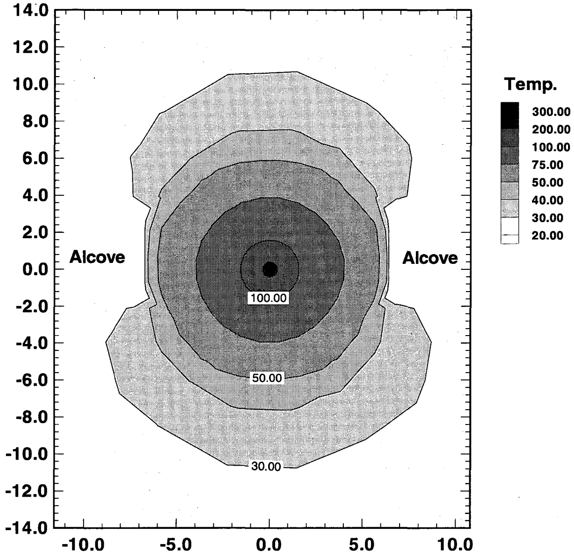
Figure 6.6-1 Temperature response for case with low matrix permeability at 1 year in 2D - simulation.
