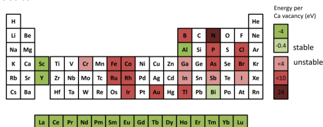
Fig. 4: Energy per Ca vacancy for the structure Ca 13 M 2 B 192 H 192 where each candidate dopant ion, M, is shown in green (stable dopant) or red (unstable dopant). Doping CaB 12 H 12 with Al, Bi, and rare-earth elements is energetically favorable.
