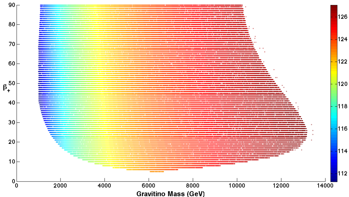
FIG. 5: Two-Dimensional Scan of BGW Parameter Space for \tan\beta = 42.5 . Distribution of points with proper EWSB and chargino mass, for m_t = 173.5 GeV. The Higgs mass (in units of GeV) is indicated by the color. The region in the lower left is excluded by the chargino mass bound as before. The region to the right at extreme values of m_{3/2} is excluded by a lack of reliable EWSB.
