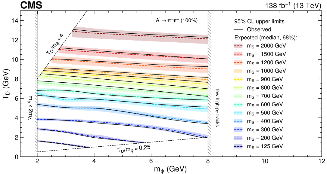
FIG. 4. The observed and expected exclusions for the nominal S cross section in the plane of m_\phi and T_D , for various m_S values, for the case m_{A'} = 1.0 GeV ( A' \rightarrow \pi^+\pi^- with \mathcal{B} = 100\% ). The regions below the observed limits are excluded.
