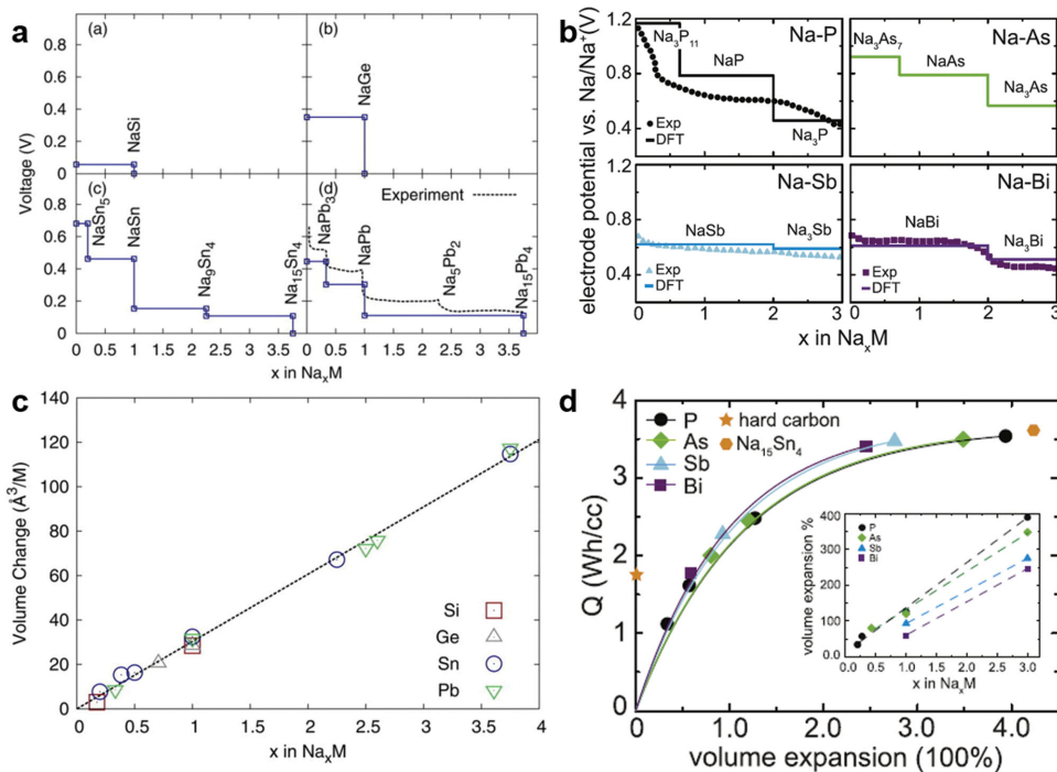
Figure 16. Calculated voltage profiles of Na–M alloys with respect to \text{Na}^+/\text{Na} for a) group-14 elements and b) group-15 elements and calculated volume changes for c) group-14 elements and d) group-15 elements. Experimental values are also given if available. Reproduced with permission. [411,412] Copyright 2011, The Electrochemical Society. Copyright 2015, Elsevier.
