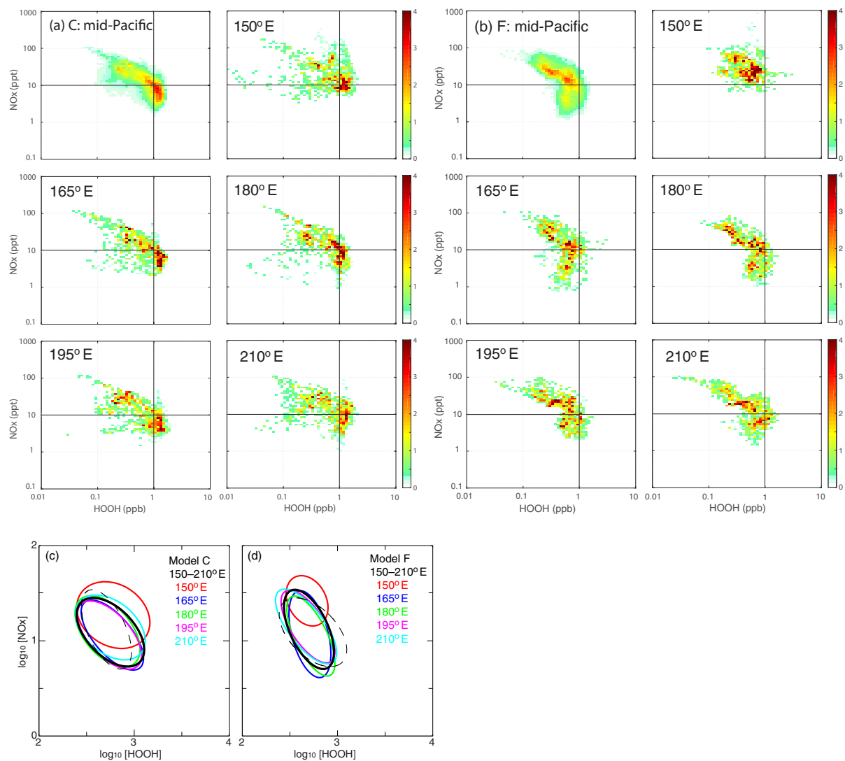
Figure 8. AIR-weighted 2-D probability distributions for \text{NO}_x vs. HOOH averaged over tropical Pacific block ( 150\text{--}210^\circ\text{E} , 20^\circ\text{S}\text{--}20^\circ\text{N} , 0\text{--}12\text{ km} ) and for different single-longitude transects from 150\text{--}210^\circ\text{E} , shown for models (a) C (GFDL-AM3) and (b) F (UCI-CTM). The fitted 2-D ellipses are shown for the full block (thick black line) and five longitude transects (colored lines) for models (c) C and (d) F. The block ellipse for the other model is shown as a thin black dashed line.
