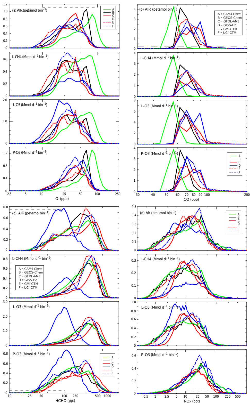
Figure 5. Six modeled 1-D probability distributions for \text{O}_3 , CO, \text{NO}_x , and HCHO, where the air parcels have been weighted by air mass (row 1), L-CH 4 (row 2), L-O 3 (row 3), and P-O 3 (row 4). The domain being sampled in the models is the tropical Pacific: 20° S–20° N, 150–210° E, 0.5–12 km. Units for the air weighting are petamoles per bin where the bins are set at 20 per decade (sizes marked by dashed lines in upper or lower panels) and Mmoles per bin per day for the reactivity-weighted plots (rows 2–4).
