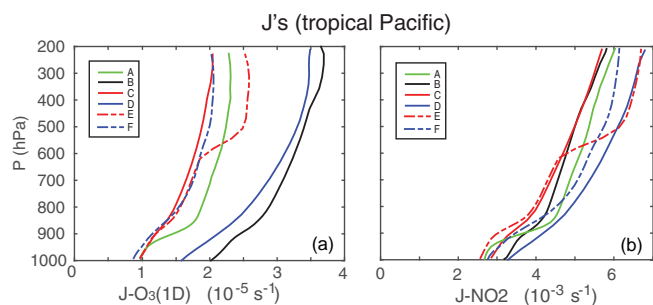
Figure 4. Modeled 24 h average J -values for \text{O}_3 + hv \Rightarrow \text{O}(^1D) + \text{O}_2 (a, \text{s}^{-1} ) and \text{NO}_2 + hv \Rightarrow \text{NO} + \text{O} (b, \text{s}^{-1} ) for the tropical Pacific ( 20^\circ\text{S} – 20^\circ\text{N} , 150 – 210^\circ\text{E} ). See Fig. 3 and Table 1 for model codes.
