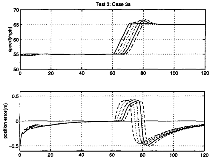
Figure 17: At t = 60 sec, platoon accelerates to 65 mph.
