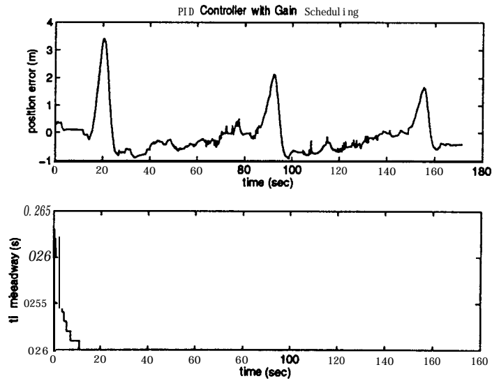
Figure 20: The position error and time headway for PID controller with gain scheduling and no v-v communication.
