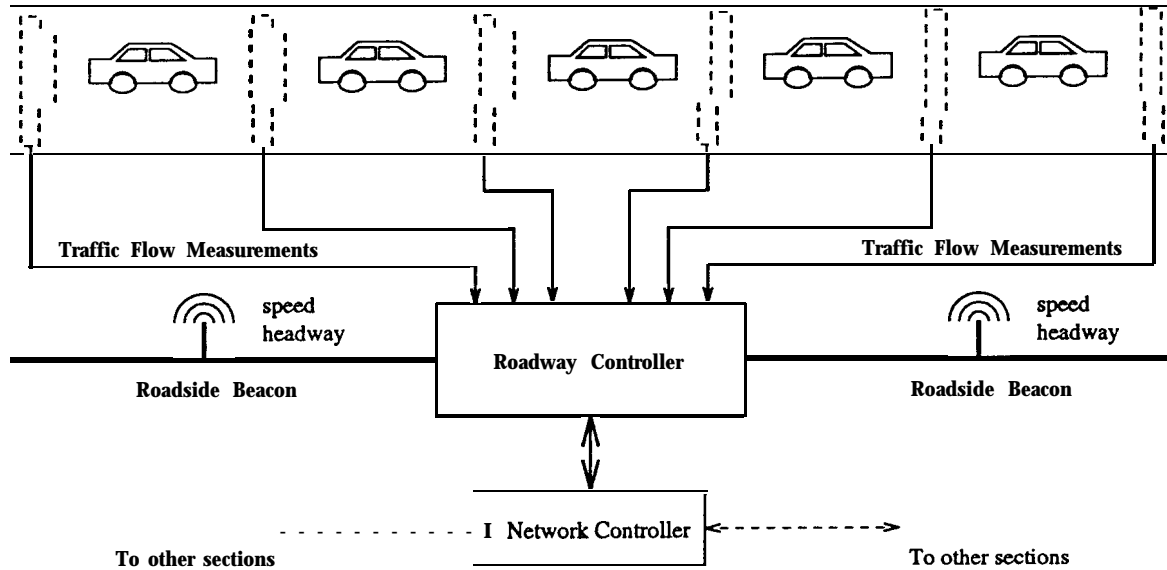
Figure 1: An AHS configuration.
