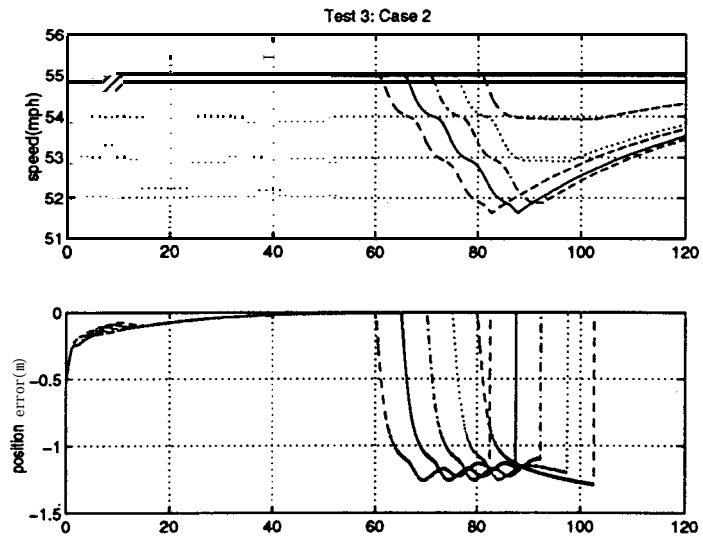
Figure 16: At t = 60 sec, vehicles starts exiting at a consecutive interval of 5 sec.
