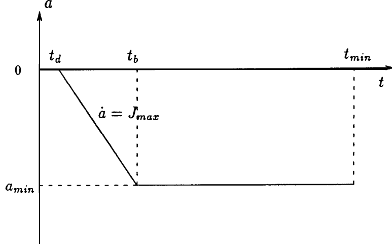
Figure 9: Scenario for calculation of minimum stopping time.
