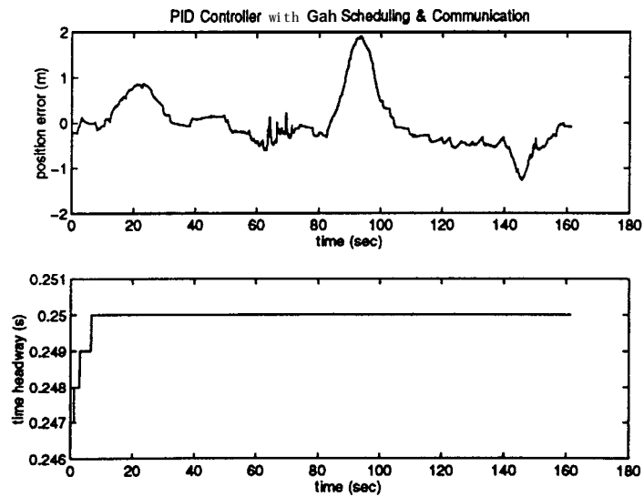
Figure 22: The position error and time headway for PID controller with gain scheduling and v-v communication.
