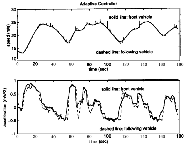
Figure 23: The speed and acceleration profiles for adaptive controller without v-v communication. The sharp spikes in leading vehicle speed are due to sensor noise.
