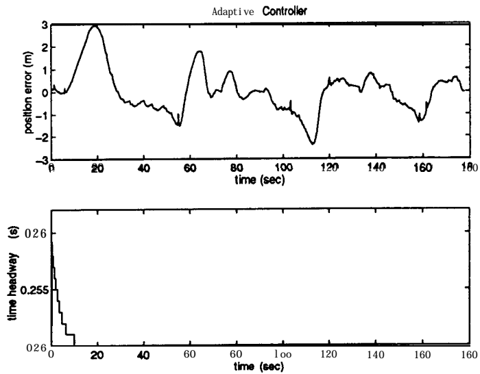
Figure 24: The position error and time headway for adaptive controller without v-v communication.
