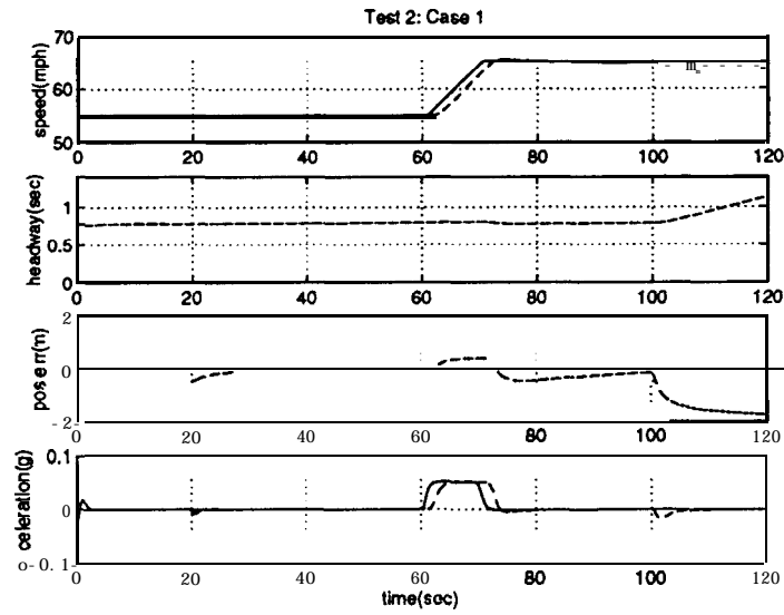
Figure 13: At t = 60 sec V_R changes from 55 to 65 mph.
