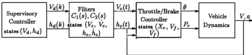
Figure 10: Closed loop system for stability analysis.
