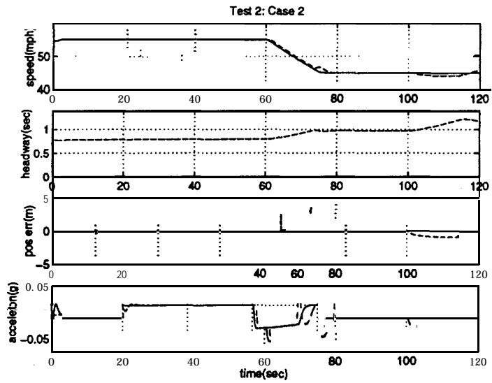
Figure 14: At t = 60 sec, h_R changes from 0.8 to 1.0 sec.
