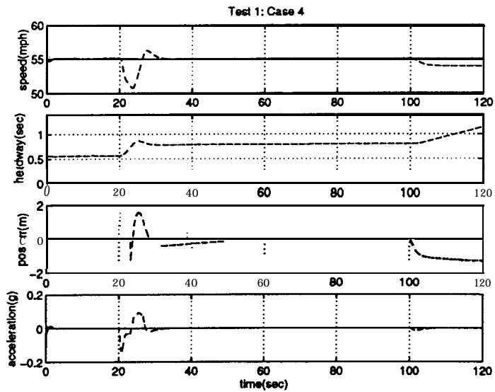
Figure 12: Follower switches on AVF at t = 20 sec with V_f = 55 mph and h_f = 0.6 sec, AVF is switched off at t = 100 sec.
