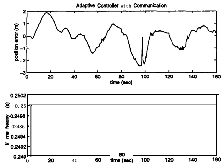
Figure 26: The position error and time headway for adaptive controller with v-v communication.
