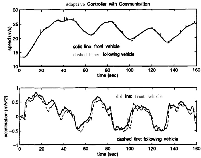
Figure 25: The speed and acceleration profiles for adaptive controller with v-v communication. The sharp spikes in leading vehicle speed are due to sensor noise.
