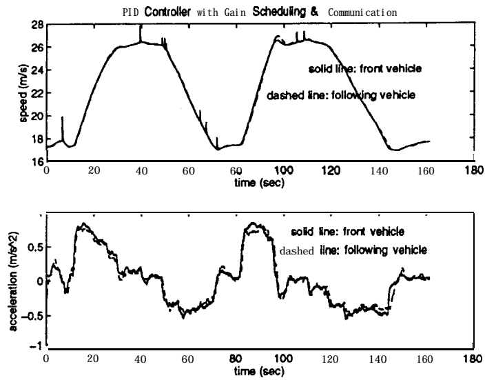
Figure 21: The speed and acceleration profiles for PID controller with gain scheduling and v-v communication. The desired speed profile is 40-55-40-55 with large acceleration.
