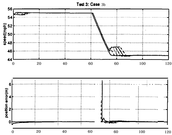
Figure 18: At t = 60 sec, platoon decelerates to 45 mph.
