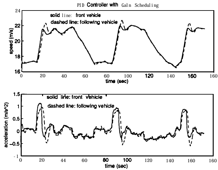
Figure 19: The speed and acceleration profiles for PID controller with gain scheduling and no v-v communication. The desired speed profile is 40-50-40-50 with large acceleration.
