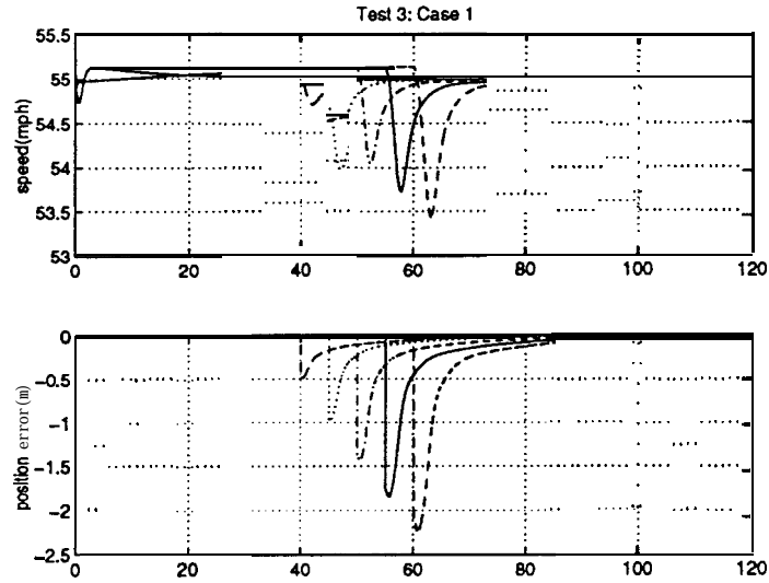
Figure 15: At t = 40 sec, five vehicles joins the leader at a consecutive interval of 5 sec.
