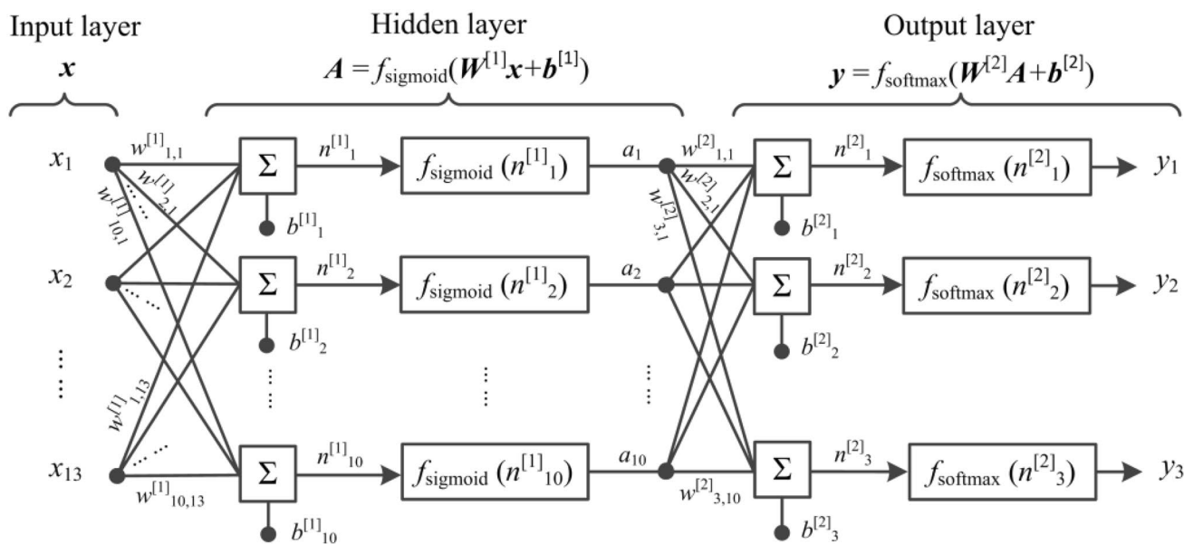
Fig. 4 The ANNs classifier architecture including an input layer ( x = x_1, x_2, \dots, x_{13} ), a hidden layer ( A = a_1, a_2, \dots, a_{10} ) and an output layer ( y = y_1, y_2, y_3 )
