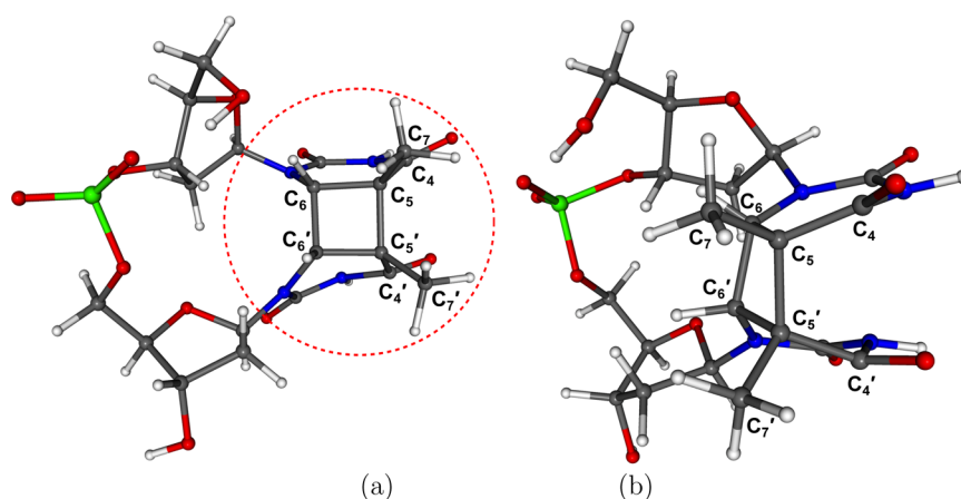
Figure 1. Optimized geometry of TpT* in the closed form: (a) front and (b) side views. The TpT* moiety is marked by red dashed circle.
