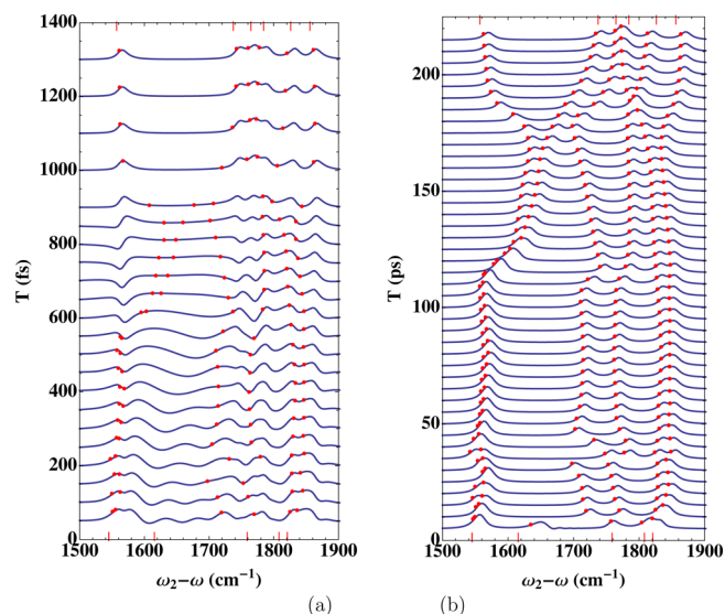
Figure 5. (a) Variation of simulated FSRs signals of TT *- with different delay times T for trajectory A ( \tau_0 = 500 fs). Time intervals are 50 fs up to 900 fs, and 100 fs later. (b) Variation of simulated FSRs signals for trajectory B ( \tau_0 = 100 ps). Time interval is 5 ps. Red dots mark instantaneous frequencies. The stick spectra on the horizontal bottom (top) axis represent the initial (final) frequencies.
