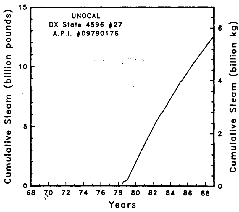
Figure A-45 Steam rate and cumulative mass flow for well DX State 4596 #27
