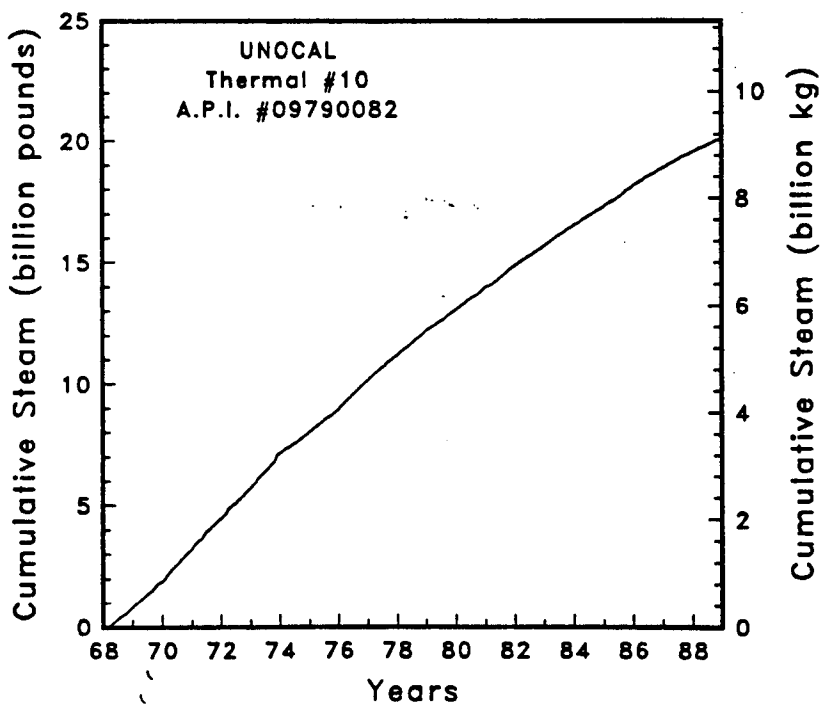
Figure A-233 Steam rate and cumulative mass flow for well Thermal #10
