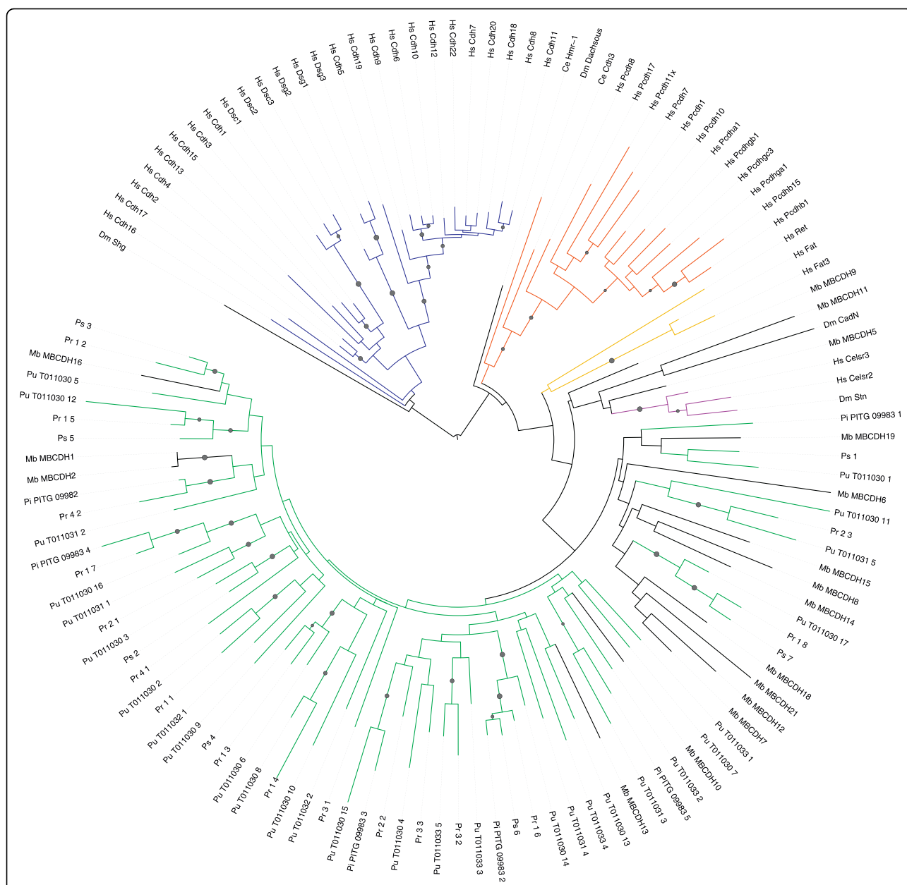
Figure 2 Phylogenetic tree of the cadherin family, showing all members of the novel oomycete subfamily (green) and their relationships to representative metazoan and choanoflagellate cadherins. The major clades of cadherins [96] are colored: C-1 (blue), Cr-1a and Cr-1b (red), C-2 (purple), and Cr-3 (orange). Most of the oomycete cadherins fall within a fairly distinct subfamily (green), though this subfamily has many long branches and also includes some cadherins from the choanoflagellate M. brevicollis (labeled starting with 'Mb') that are also highly diverged from other cadherins. Reliable branches (bootstrap > 50%) are labeled with a circle. All full-length oomycete cadherin domains are shown, from P. ultimum (labeled starting with 'Pu' and ending with the number of the repeat relative to the amino terminus), Ph. infestans (labeled starting with 'Pi'), Ph. sojae (Ps) and Ph. ramorum (Pr). Other cadherins are from the human genome ('Hs') unless labeled starting with 'Dm' ( Drosophila melanogaster ) or 'Ce' ( Caenorhabditis elegans ). The figure was drawn using the iTOL tool [143].
