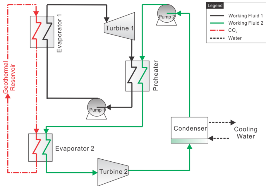
Fig. 26. Coupled ORC
