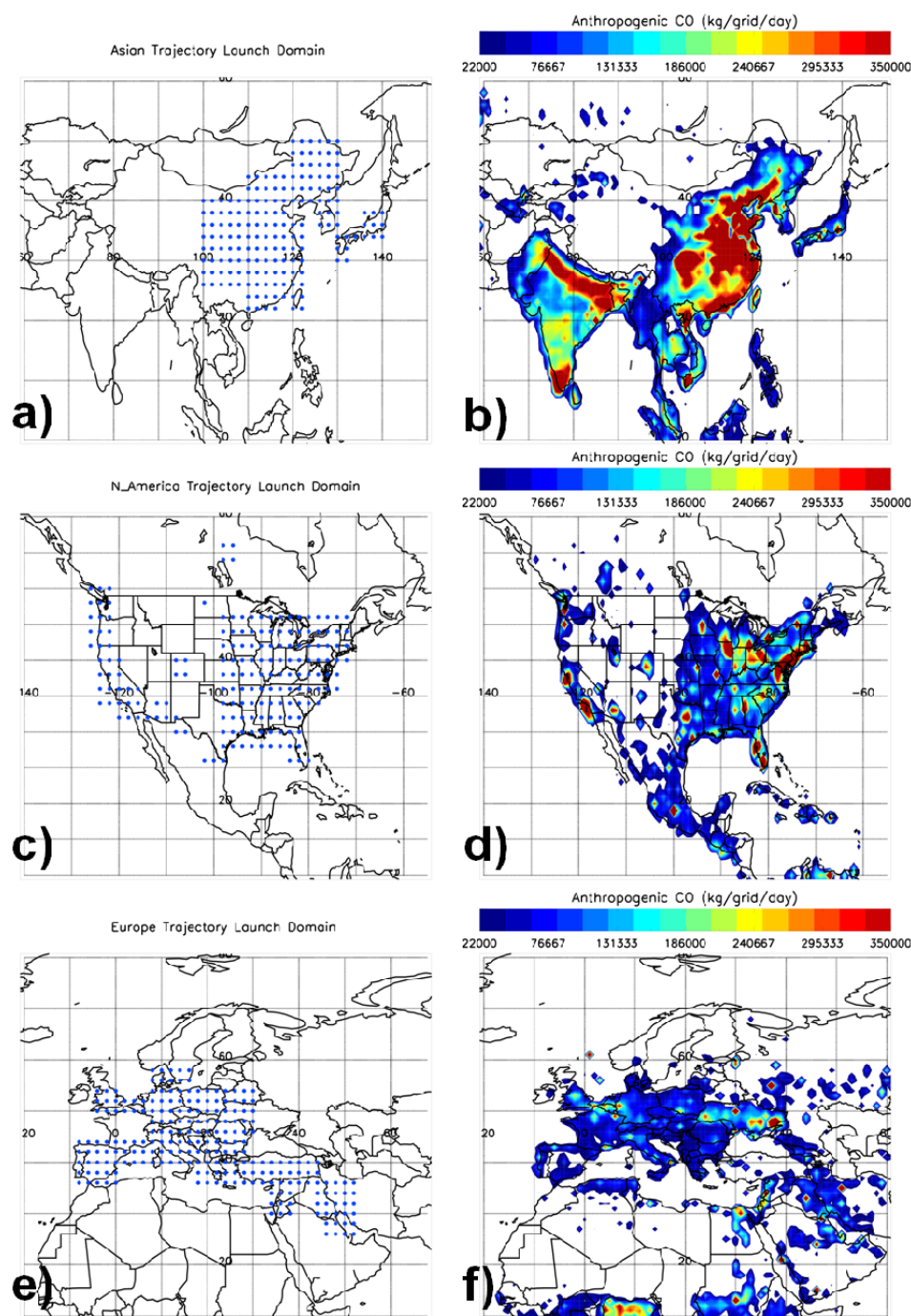
Fig. 2. Trajectory release locations on the 2.0^\circ \times 2.0^\circ grid (blue dots) for (a) Asia, (c) North America, and (e) Europe. These locations were based on anthropogenic emissions during ARCTAS ( \text{kg grid point}^{-1} \text{ day}^{-1} ) for (b) Asia, (d) North America, and (f) Europe from the CGRER data set.
