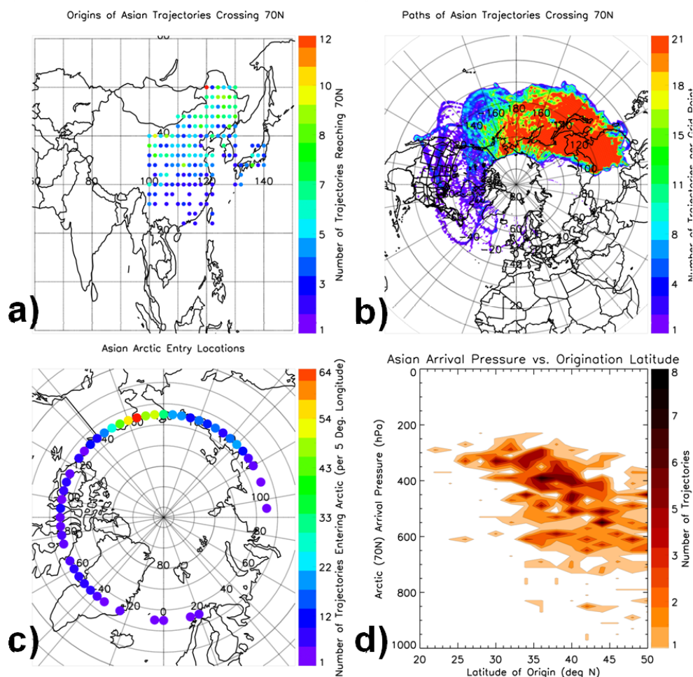
Fig. 4. Trajectory statistics for the eastern Asia domain. (a) Number and originating locations of trajectories reaching the Arctic (70° N) within 15 days. (b) Pathways taken by all 15 day trajectories reaching the Arctic. (c) Number and location of trajectories entering the Arctic. (d) Pressure level at which Arctic bound trajectories arrive at 70° N.
