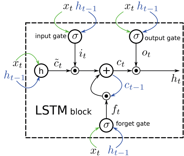
Fig. 2. Illustration of a LSTM block. The green connections are feedforward with associated weight matrices. The blue are feedback weight connections. Best viewed in color.
