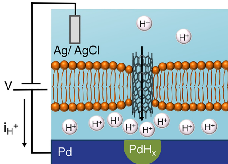
Fig 1. A bioprotonic device with integrated carbon nanotube porins (CNTPs) supports proton current across the SLB through the CNTPs when a negative voltage ( -V ) is applied on the Pd contact. When H^+ reach the surface of the Pd contact, they are reduced to H by an incoming electron and diffuse into the Pd to form palladium hydride ( PdH_x ). The current density at the contact ( -i_{H^+} ), measures the rate of H^+ flux along the CNTPs.
