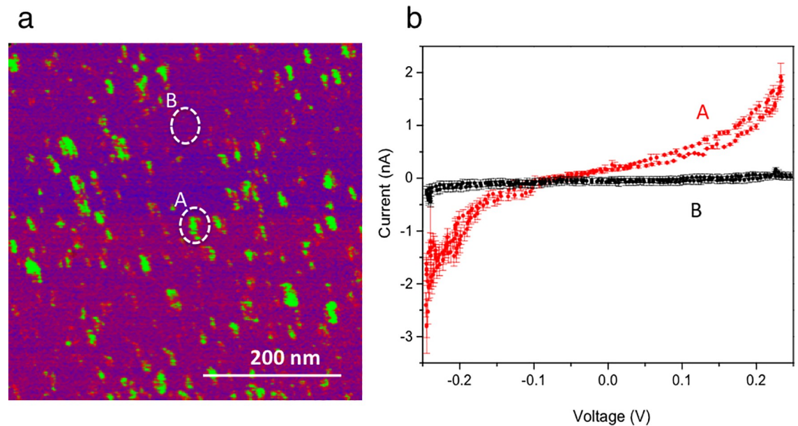
Fig 4. Conductive AFM of SLB with CNTPs channels. (a) The current map for the Pd contact with SLB incorporating CNTPs. The hot spot (green spot) correspond to higher current (red trace) that represent CNT and the background (purple area) correspond to negligible amount of current (black trace) which represent SLB membrane. (b) In the IV curve the red trace collected from the green spot and the back trace collected from the purple area. The green spot has i \sim 1.78 \text{ nA} \pm 0.09 \text{ nA} and purple area has i \sim 5.86 \text{ pA} \pm 0.98 \text{ pA} . This current most likely represents the electron conductivity of CNT. (The data are collected from 3 different areas of the AFM image for both green spot and purple area. The error bars are the root mean square of the displacement of the data from the average value).
