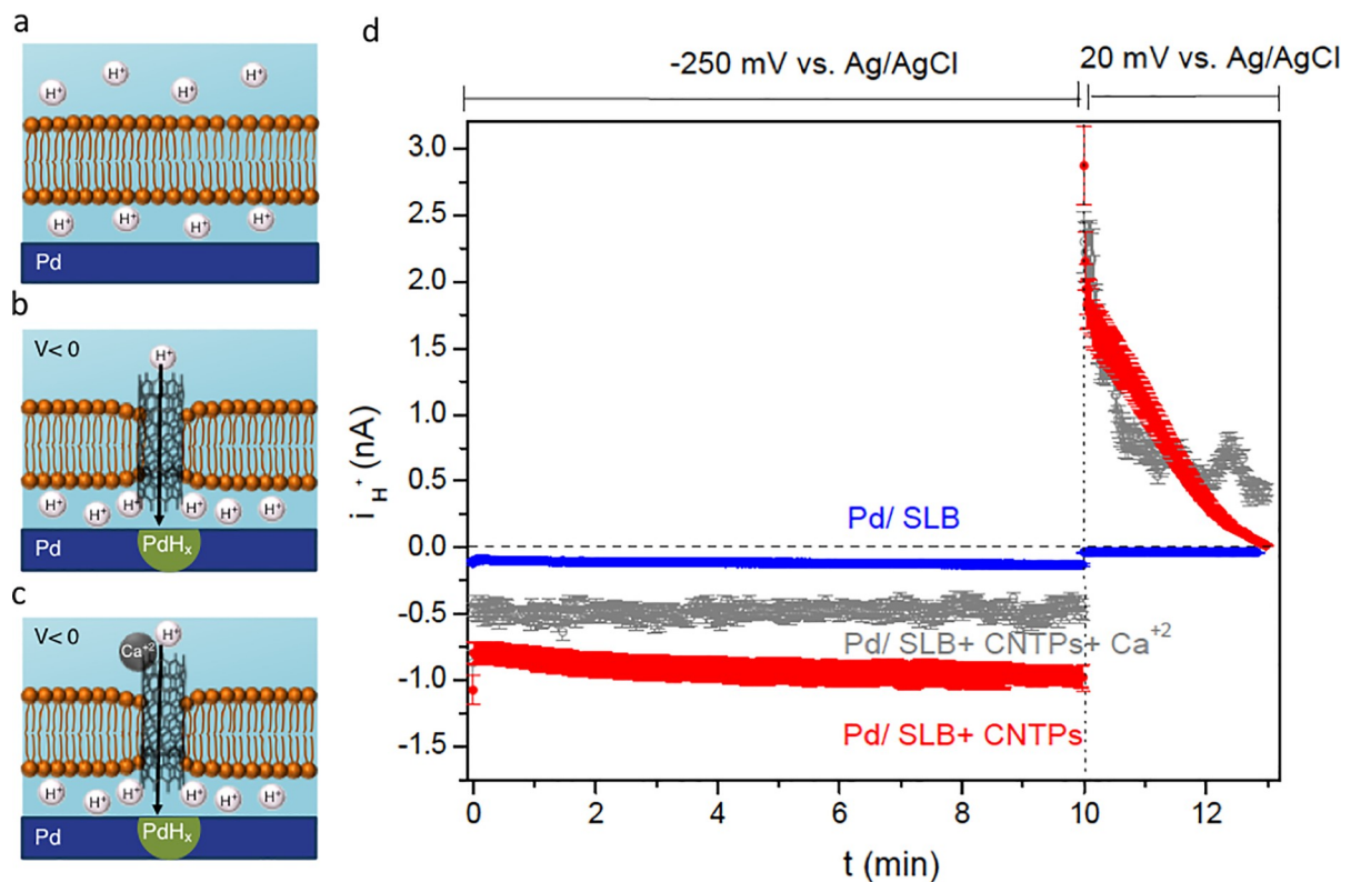
Fig 2. (a) Pd contact with SLB. The SLB blocks H^+ from transferring from the solution to the Pd contact even with V = -250 mV (vs. Ag/AgCl). (b) Pd contact with SLB incorporating 0.8 nm diameter CNTPs is semipermeable to H^+ , with CNTPs facilitating the rapid flow of H^+ to the Pd/solution interface. (c) Upon addition of Ca^{+2} to the bulk solution, H^+ current through CNTPs becomes partially blocked. (d) i_{H^+} vs. time plots recorded at V = -250 mV and V = 20 mV. Blue trace: SLB, red trace: SLB with CNTPs, gray trace SLB with CNTPs in presence of Ca^{+2} ions in the bulk solution. (The data are collected from 3 different devices with different dimensions: Pd / SLB: 3 different devices of 2 \times 50 \mu m , Pd/SLB+CNTPs: 3 different devices of 2 \times 50 \mu m , Pd/SLB+CNTPs+ Ca^{+2} : 3 different devices of 2 \times 50 \mu m . The error bars are the root mean square of the displacement of the data from the average value).
